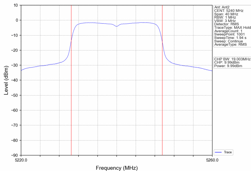
802.11ac(VHT20)_HCH_5240MHz_Ant2_NTNV
