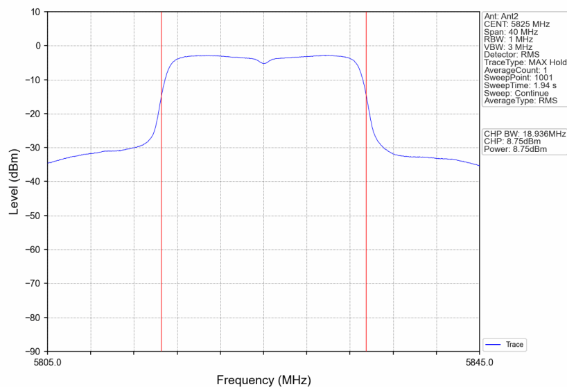
802.11ac(VHT20)_HCH_5825MHz_Ant2_NTNV
