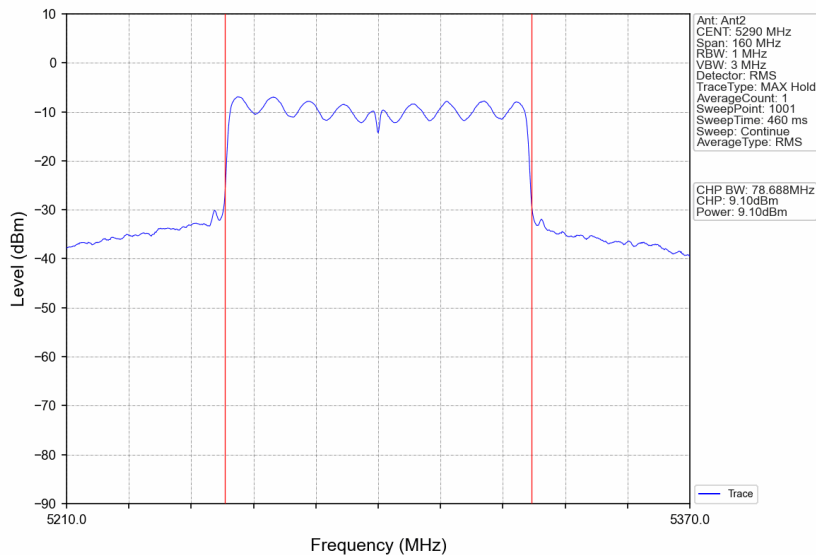
802.11ac(VHT80)_MCH_5290MHz_Ant2_NTNV
