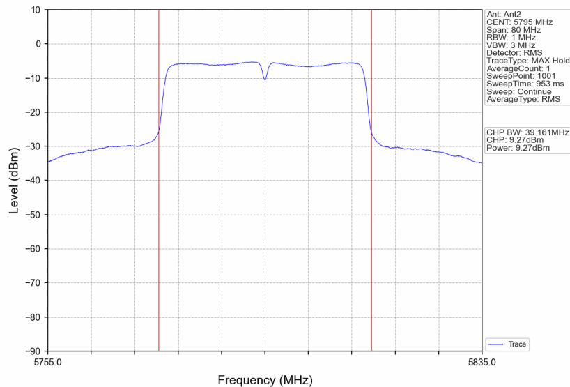
802.11ac(VHT40)_HCH_5795MHz_Ant2_NTNV
