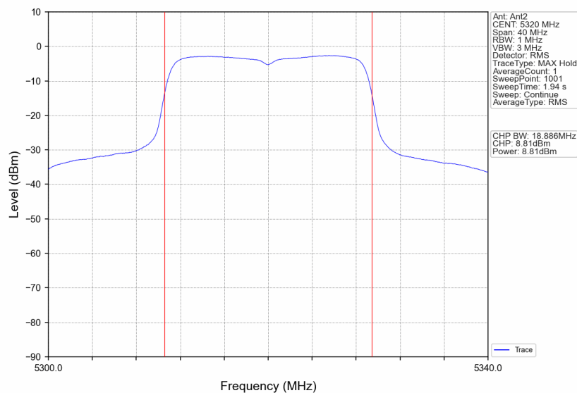
802.11ac(VHT20)_HCH_5320MHz_Ant2_NTNV
