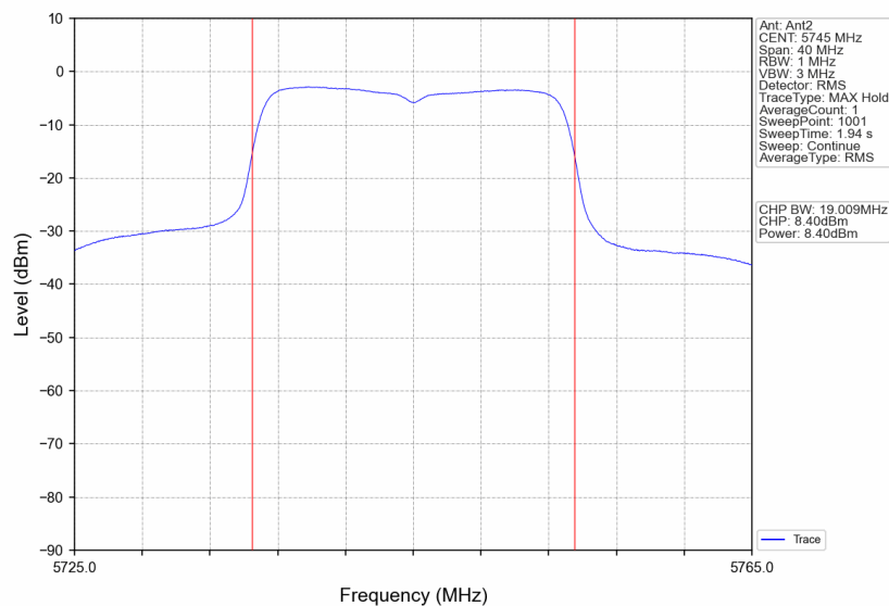
802.11ac(VHT20)_LCH_5745MHz_Ant2_NTNV
