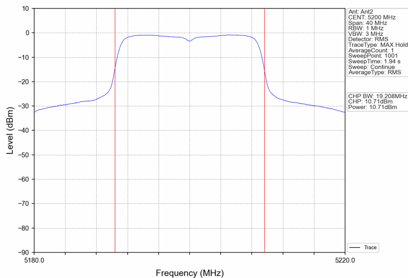
802.11ac(VHT20)_MCH_5200MHz_Ant2_NTNV
