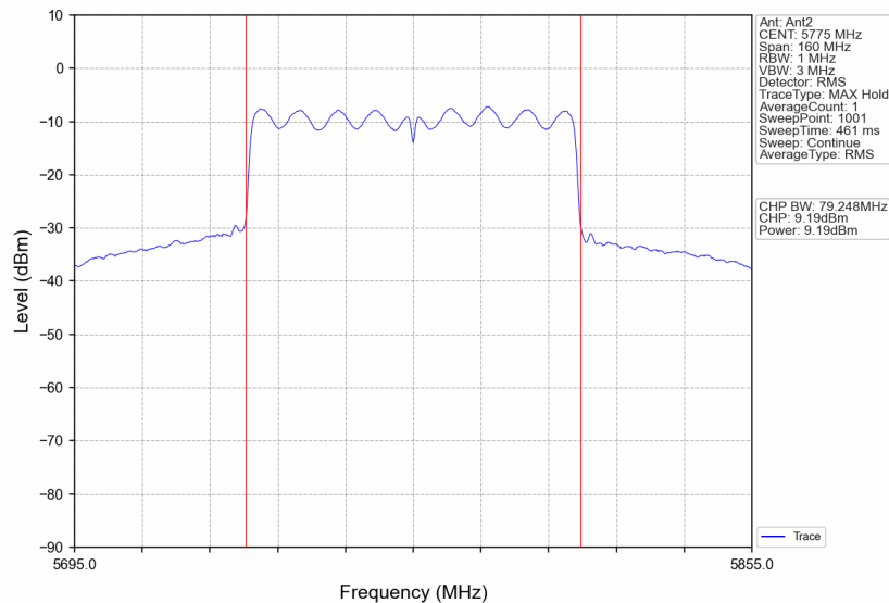
802.11ac(VHT80)_MCH_5775MHz_Ant2_NTNV
