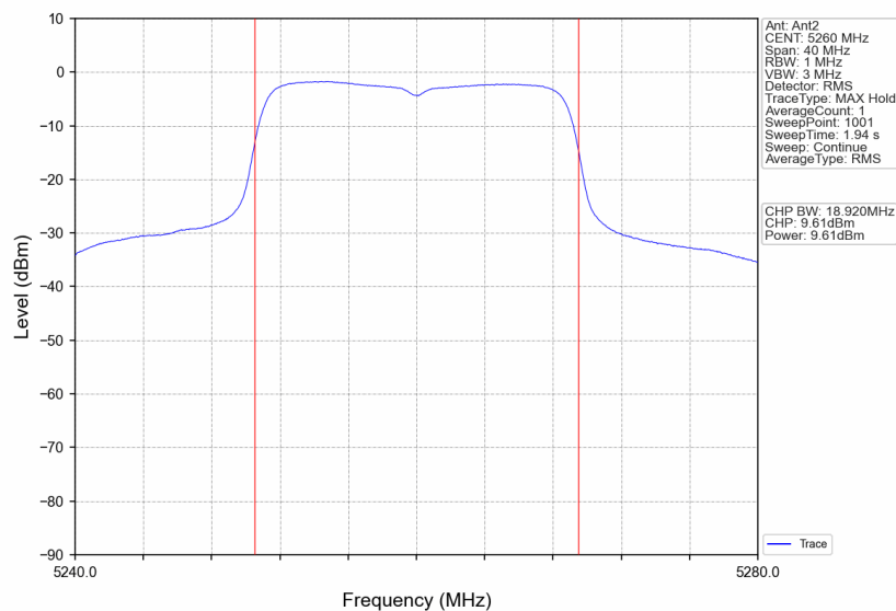
802.11ac(VHT20)_LCH_5260MHz_Ant2_NTNV
