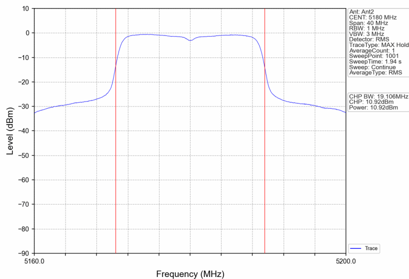
802.11ac(VHT20)_LCH_5180MHz_Ant2_NTNV
