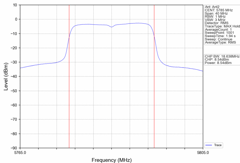
802.11ac(VHT20)_MCH_5785MHz_Ant2_NTNV
