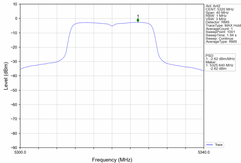
802.11ac(VHT20)_HCH_5320MHz_MIMO_NTNV
