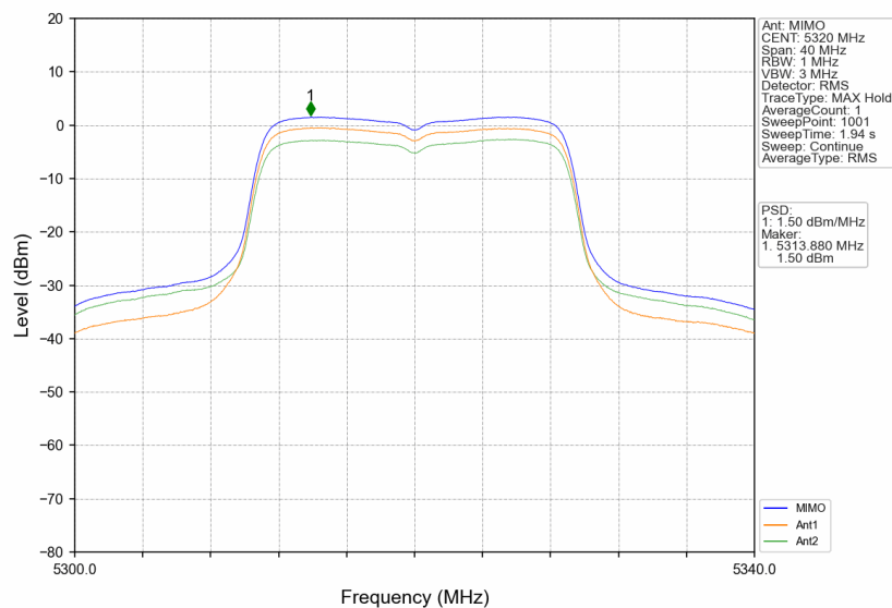
802.11ac(VHT20)_HCH_5320MHz_MIMO_NTNV
