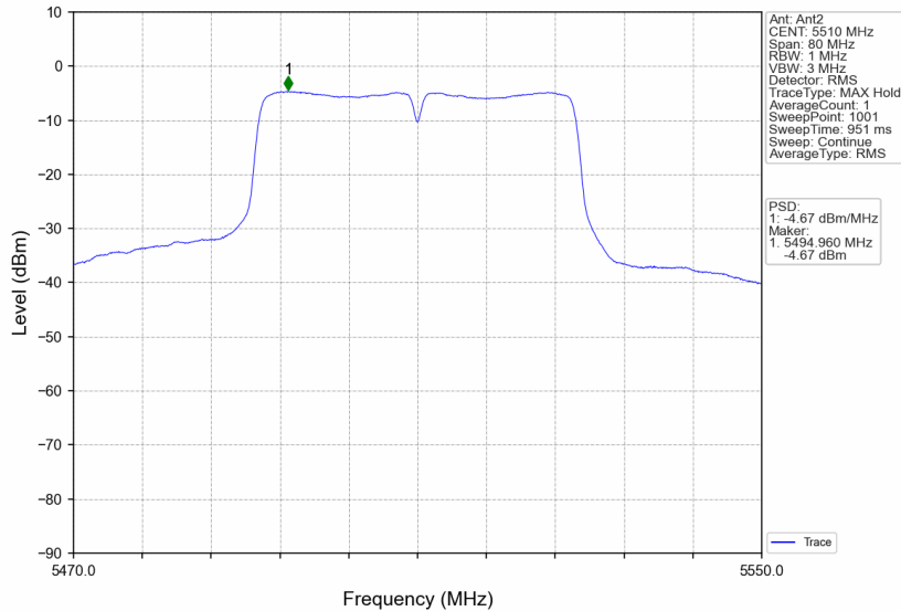
802.11n(HT40)_LCH_5510MHz_MIMO_NTNV
