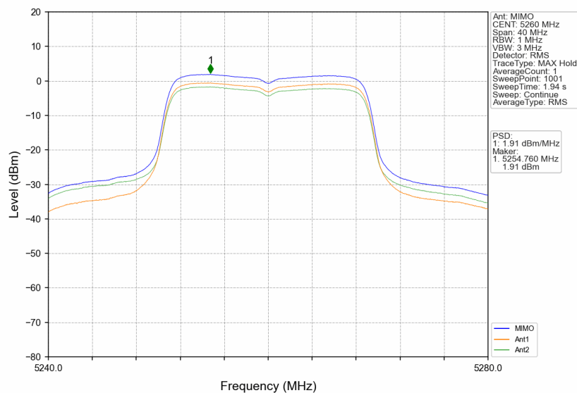
802.11ac(VHT20)_LCH_5260MHz_MIMO_NTNV
