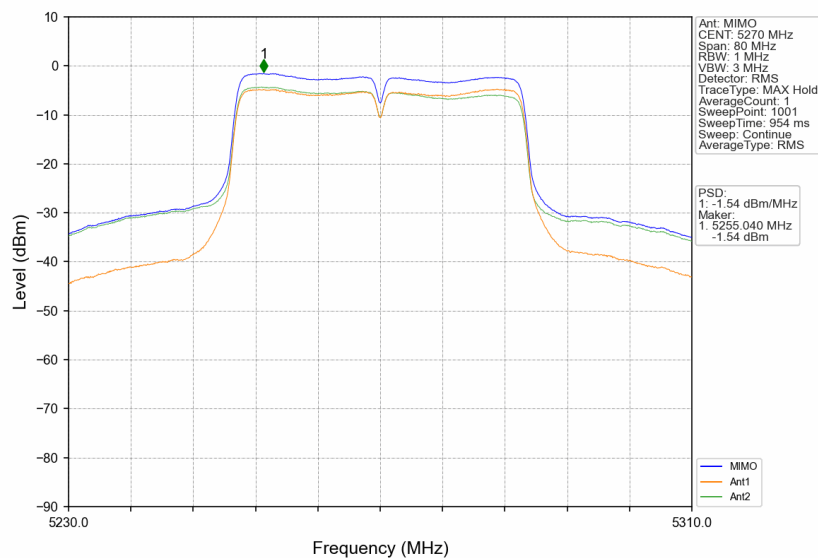
802.11ac(VHT40)_LCH_5270MHz_MIMO_NTNV
