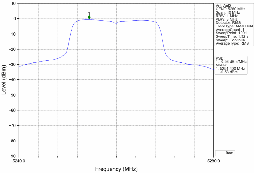
802.11n(HT20)_LCH_5260MHz_MIMO_NTNV
