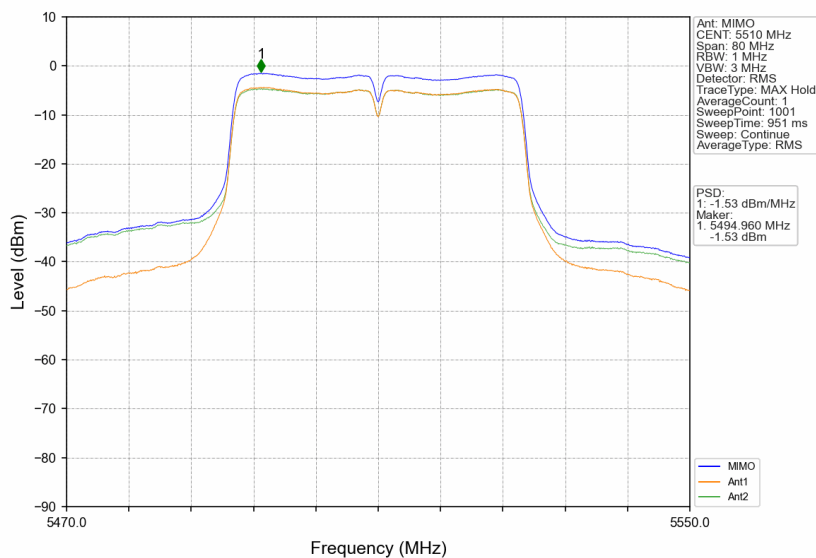
802.11n(HT40)_LCH_5510MHz_MIMO_NTNV
