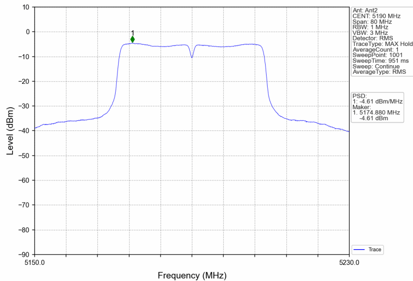
802.11n(HT40)_LCH_5190MHz_MIMO_NTNV
