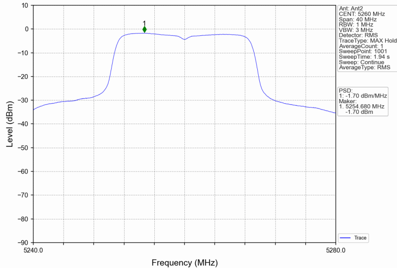
802.11ac(VHT20)_LCH_5260MHz_MIMO_NTNV
