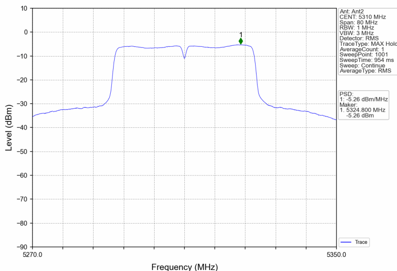
802.11ac(VHT40)_HCH_5310MHz_Ant2_NTNV
