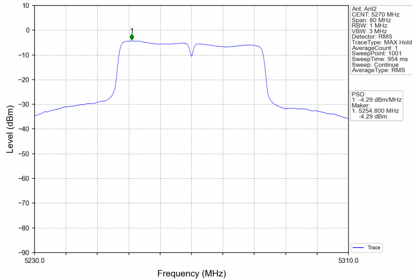
802.11ac(VHT40)_LCH_5270MHz_MIMO_NTNV
