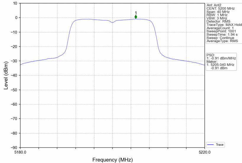
802.11ac(VHT20)_MCH_5200MHz_MIMO_NTNV
