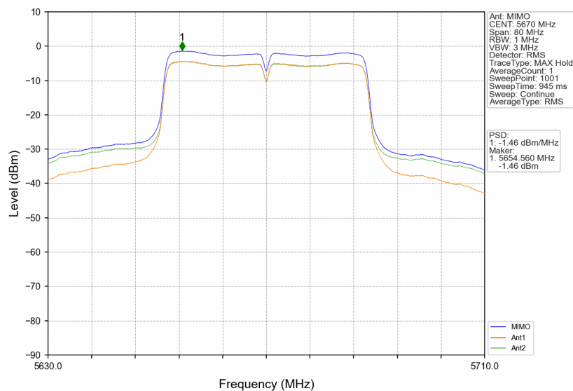
802.11n(HT40)_HCH_5670MHz_MIMO_NTNV
