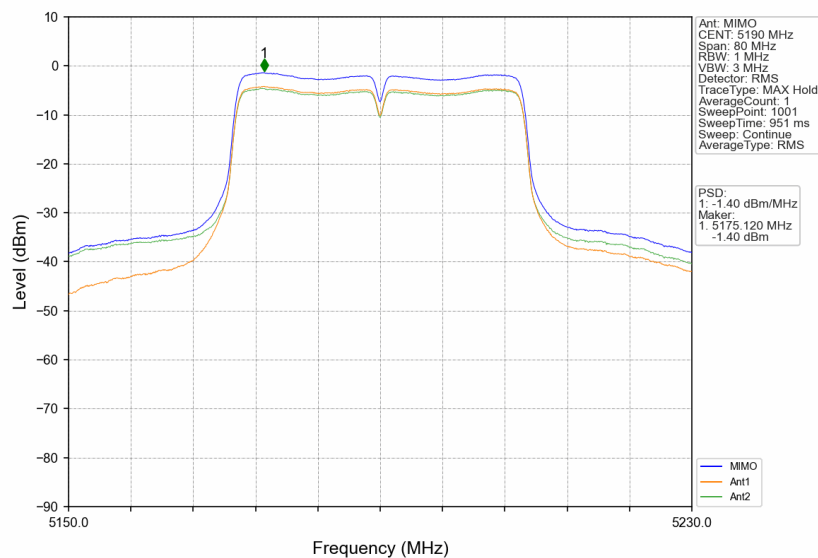
802.11n(HT40)_LCH_5190MHz_MIMO_NTNV
