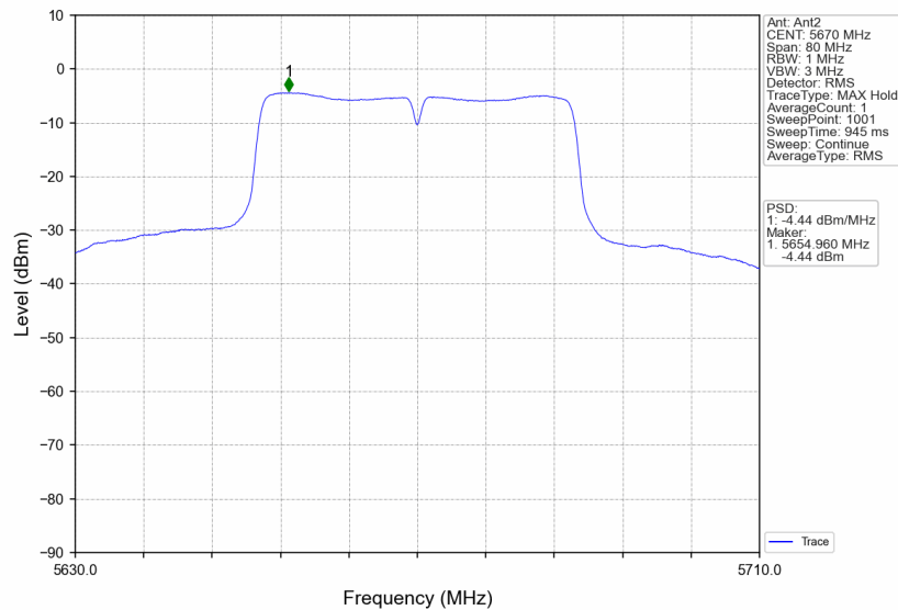
802.11n(HT40)_HCH_5670MHz_MIMO_NTNV
