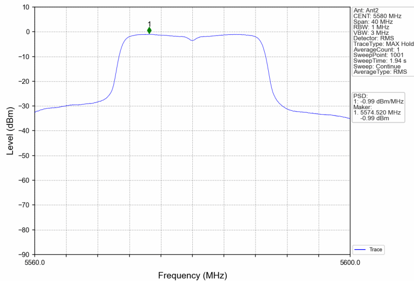
802.11ac(VHT20)_MCH_5580MHz_MIMO_NTNV
