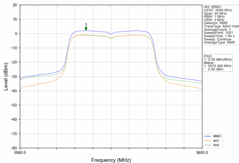
802.11ac(VHT20)_MCH_5580MHz_MIMO_NTNV
