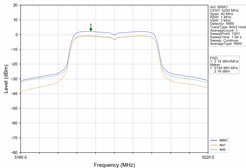
802.11ac(VHT20)_MCH_5200MHz_MIMO_NTNV
