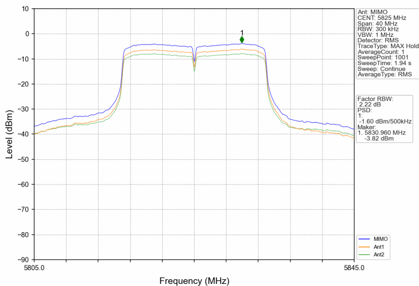
802.11ac(VHT20)_HCH_5825MHz_MIMO_NTNV
