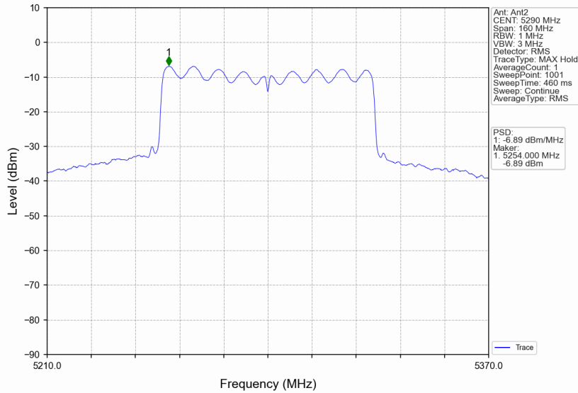
802.11ac(VHT80)_MCH_5290MHz_MIMO_NTNV
