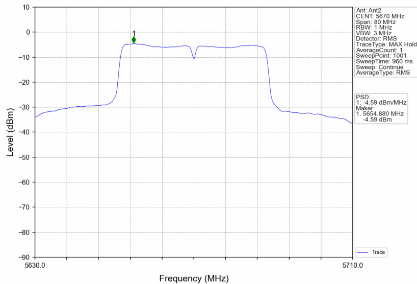
802.11ac(VHT40)_HCH_5670MHz_MIMO_NTNV
