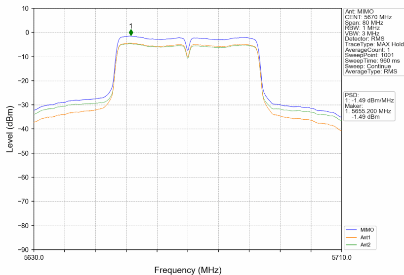
802.11ac(VHT40)_HCH_5670MHz_MIMO_NTNV
