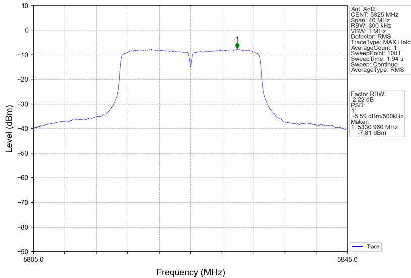
802.11ac(VHT20)_HCH_5825MHz_MIMO_NTNV
