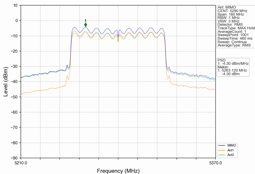
802.11ac(VHT80)_MCH_5290MHz_MIMO_NTNV
