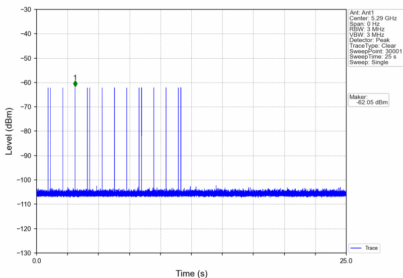
Signal Calibration_802.11ac(VHT80)_2A_5290MHz_RadarType6_Trial0
