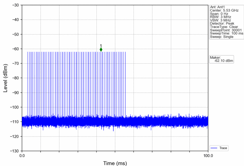
Signal Calibration_802.11ac(VHT80)_2C_5530MHz_RadarType2_Trial0
