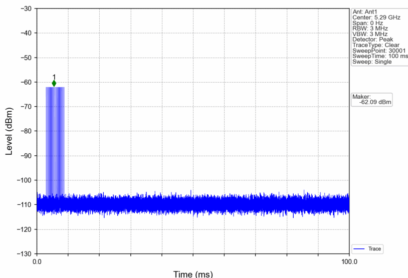
Signal Calibration_802.11ac(VHT80)_2A_5290MHz_RadarType4_Trial0
