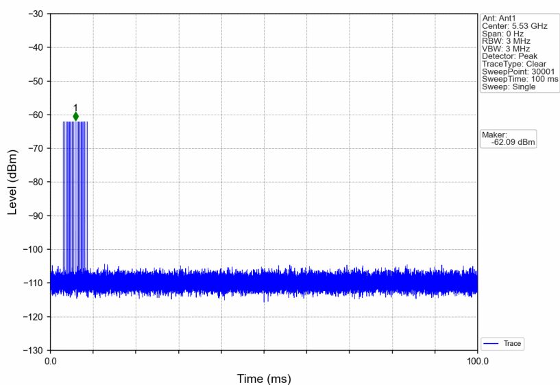
Signal Calibration_802.11ac(VHT80)_2C_5530MHz_RadarType4_Trial0
