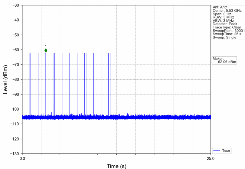
Signal Calibration_802.11ac(VHT80)_2C_5530MHz_RadarType6_Trial0
