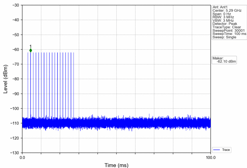
Signal Calibration_802.11ac(VHT80)_2A_5290MHz_RadarType1_Trial0
