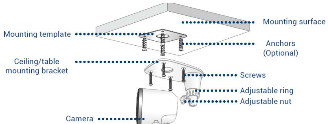
Figure 5-4 Ceiling mounting diagram
