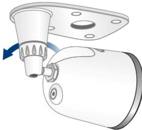
Figure 5-6 Rotate the camera
