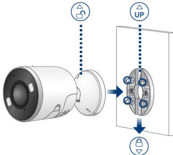
Figure 5-2 Install the bracket
