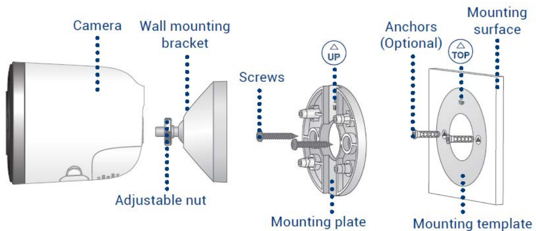
Figure 5-1 Wall mounting diagram
