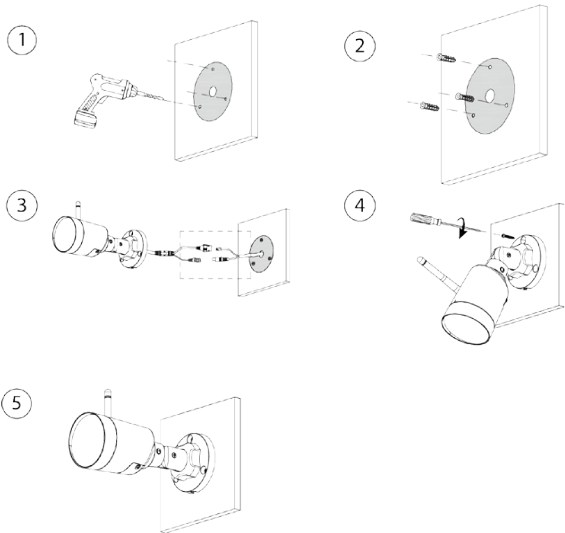
Figure 4-6 Cable going through the mounting surface
