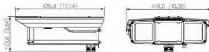
Figure 2-2 Dimensions (mm [inch])
