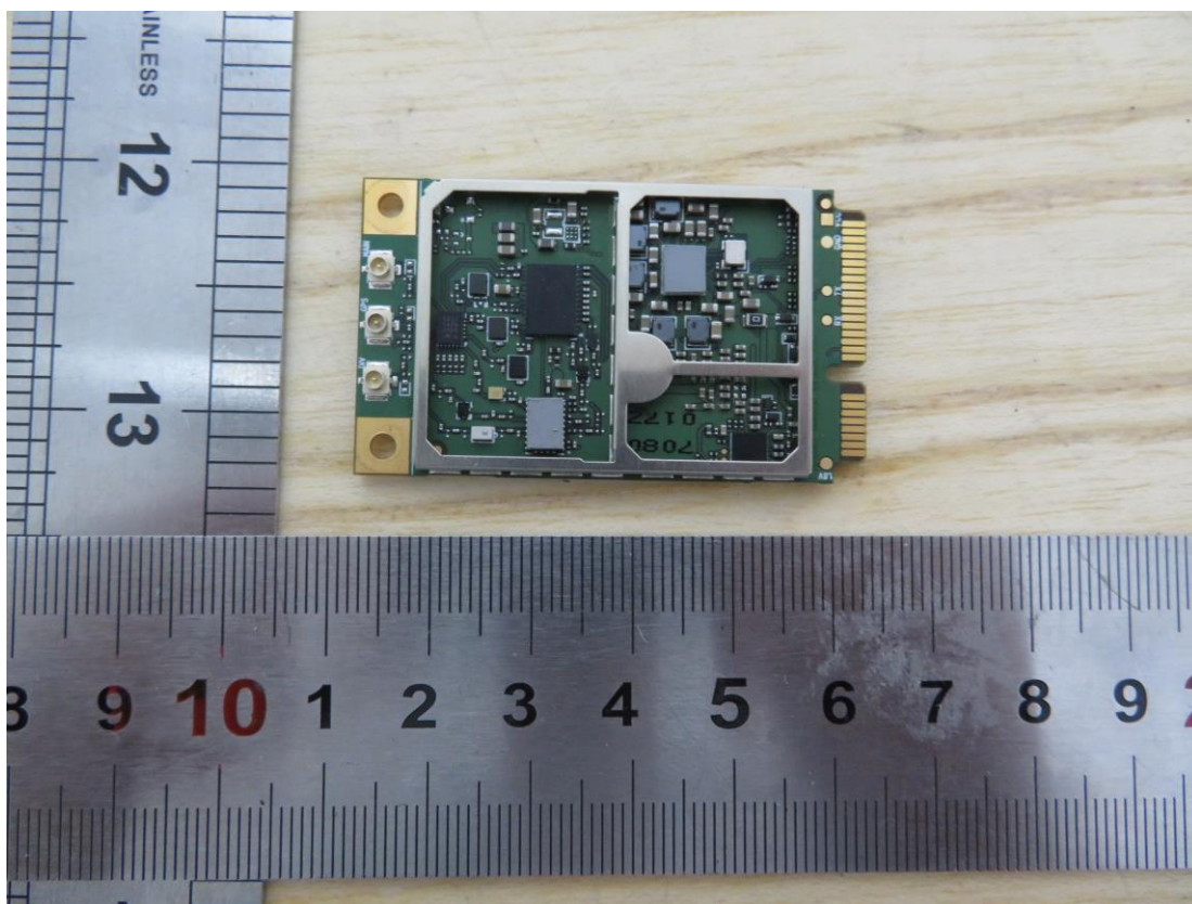
Internal View of EUT-36
