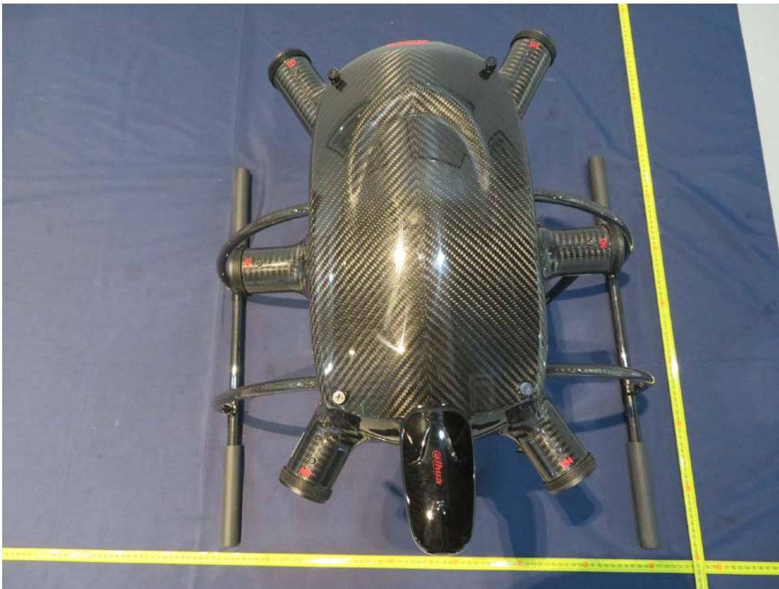
External View of EUT-2
