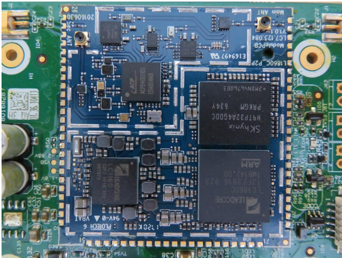
Internal View of EUT-26
