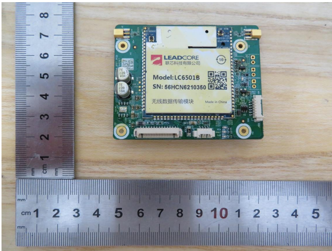
Internal View of EUT-22
