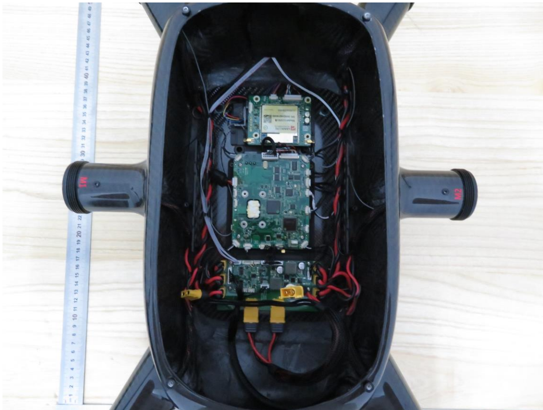
Internal View of EUT-14
