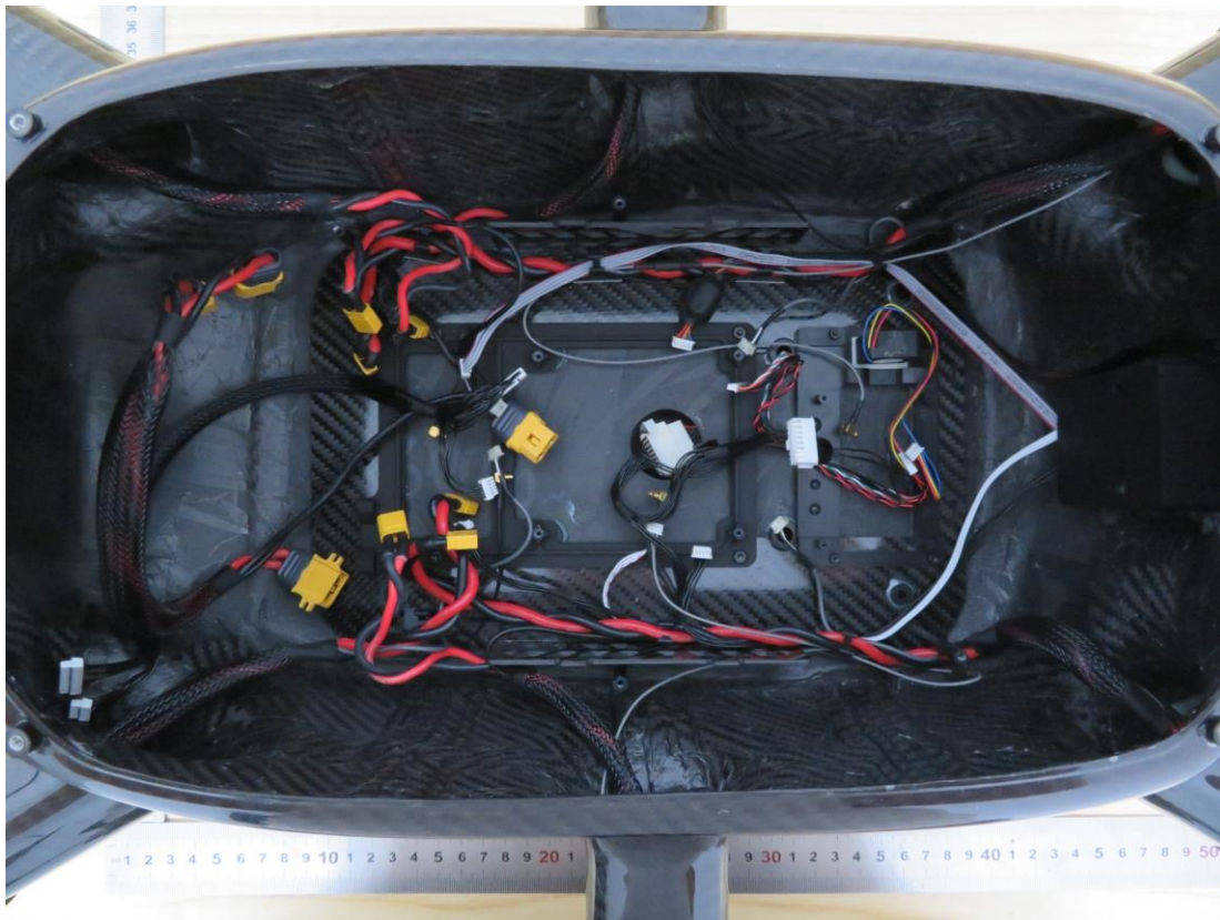
Internal View of EUT-28
