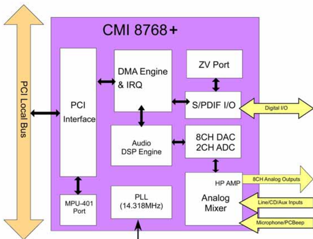
Block Diagram
