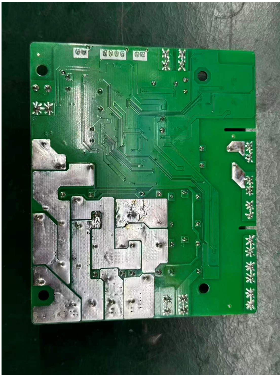
Figure 11: internal view_11 of EUT
