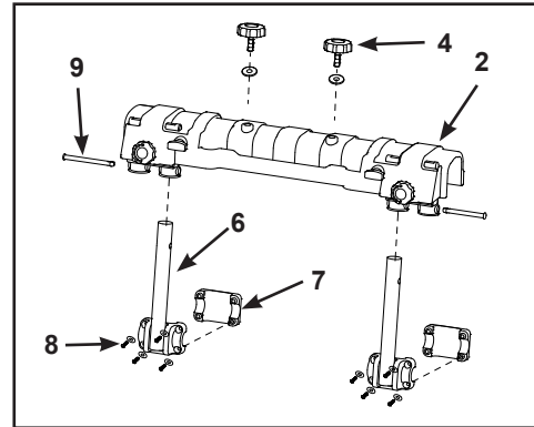
Intex Rectangular Frame Pool Mounting Bracket
