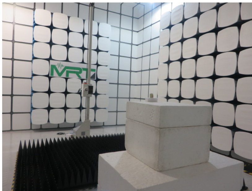
Photograph 2: Test Set-up Photo for measurements above 1GHz
