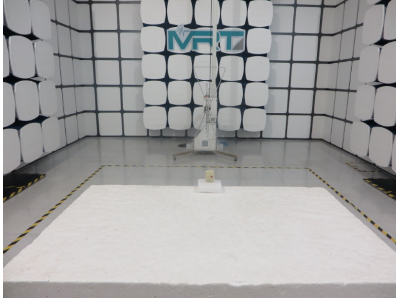
Photograph 1: Test Set-up Photo for measurements below 1GHz
