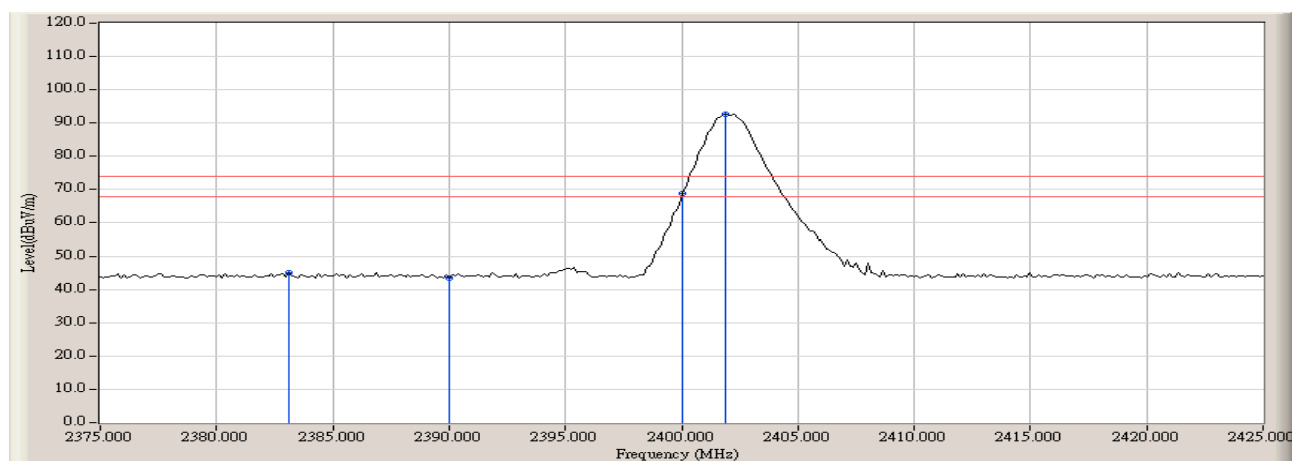
Figure Channel 00: (Vertical)
