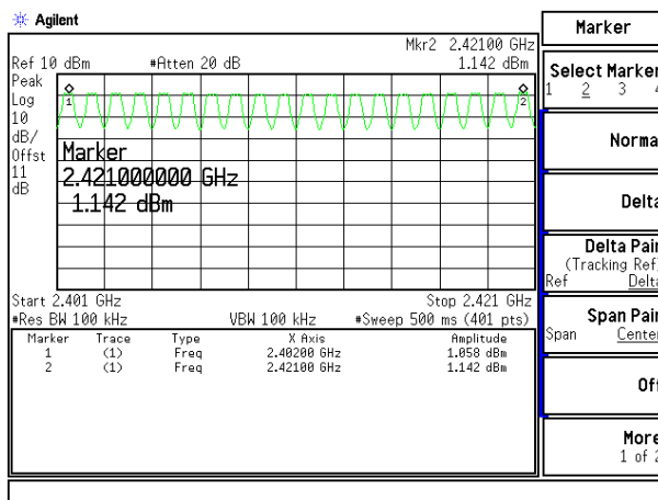
2402-2421MHz
