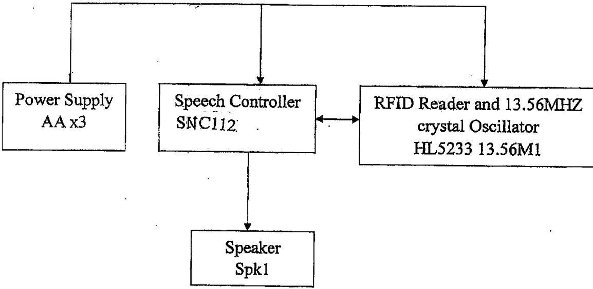
Block diagram (main unit)
