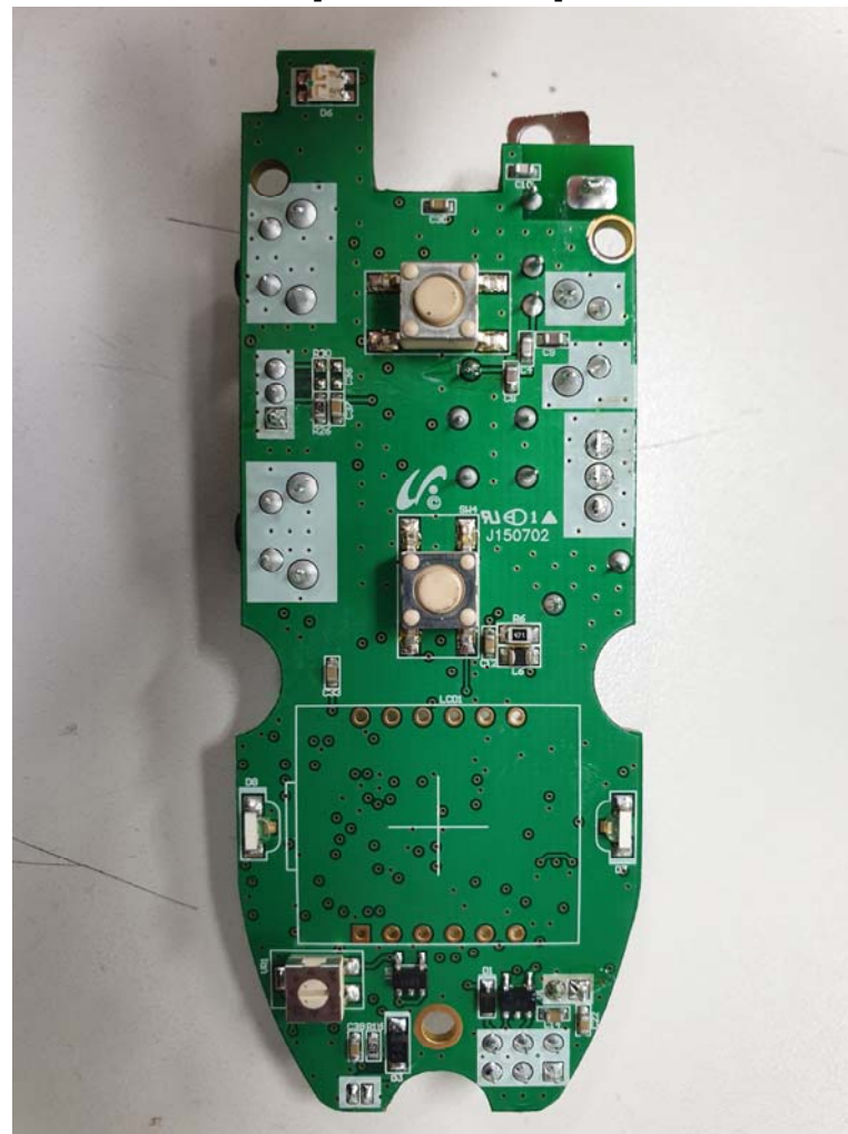
[Main board Rear]
