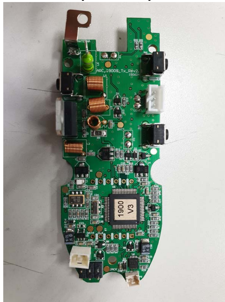
[Main board Front]
