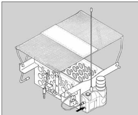
Figure 2. Plugging solenoid cable into the receiver
