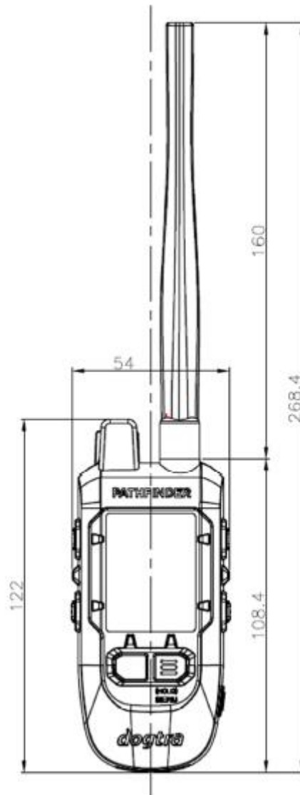
Figure E-1 Antenna Location
