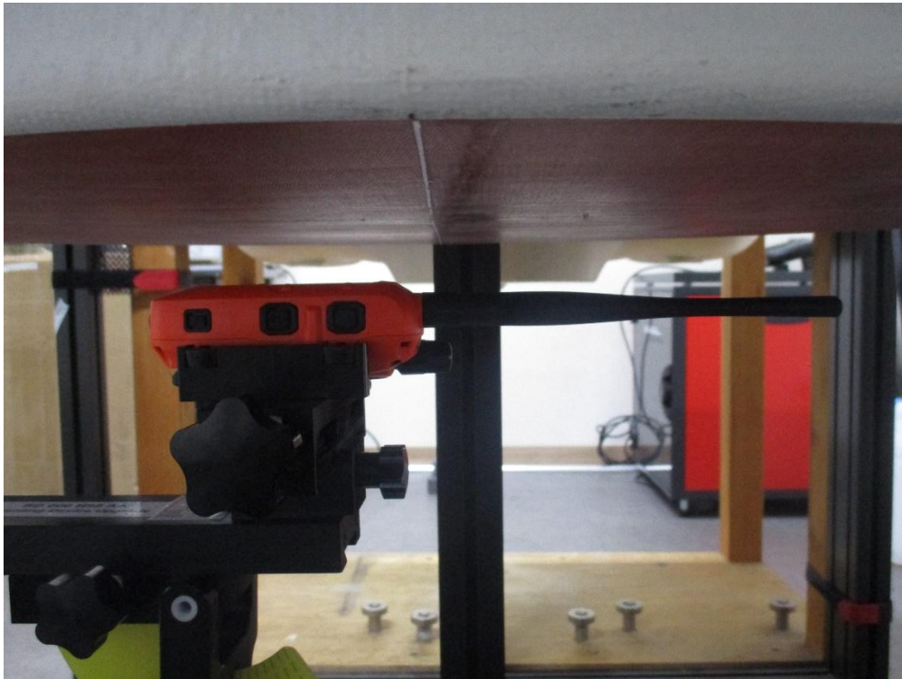
Front Side from Flat Phantom (Separation Distance: 2.5 cm)
