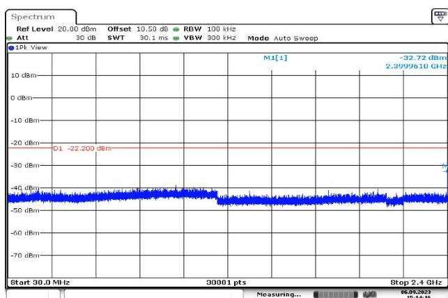
,Plot ,3Transmitter Spurious Emission : 2402,30MHz~2400MHz
