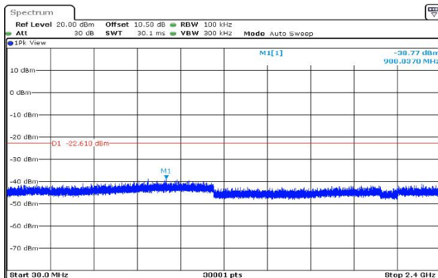
,Plot ,3Transmitter Spurious Emission : 2480,30MHz~2400MHz
