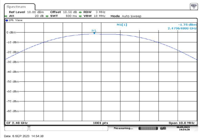
Output Power: 2480MHz – 2Mbps
