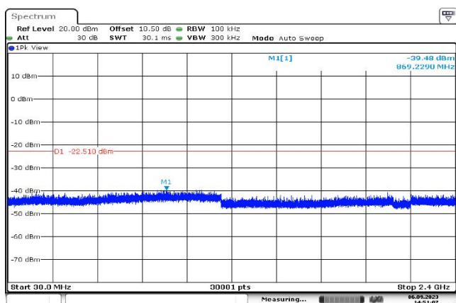
,Plot ,3Transmitter Spurious Emission : 2480,30MHz~2400MHz
