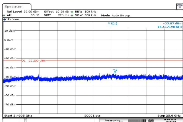
,Plot ,4Transmitter Spurious Emission : 2402,2483.5MHz~25000MHz
