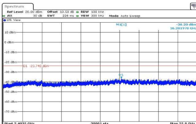
,Plot ,4Transmitter Spurious Emission : 2440,2483.5MHz~25000MHz
