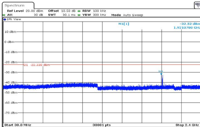
,Plot ,3Transmitter Spurious Emission : 2402,30MHz~2400MHz
