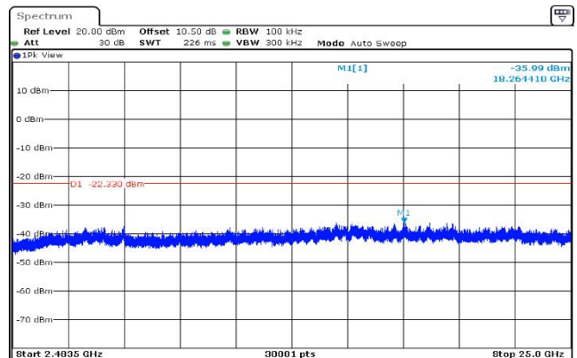
,Plot ,4Transmitter Spurious Emission : 2402,2483.5MHz~25000MHz
