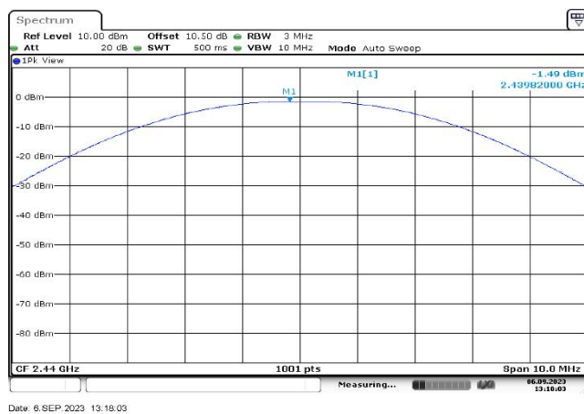
Output Power: 2440MHz – 2Mbps
