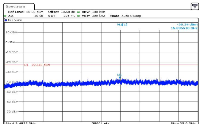
,Plot ,4Transmitter Spurious Emission : 2480,2483.5MHz~25000MHz
