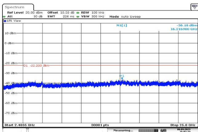
,Plot ,4Transmitter Spurious Emission : 2440,2483.5MHz~25000MHz
