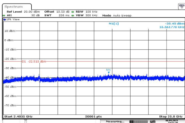
,Plot ,4Transmitter Spurious Emission : 2480,2483.5MHz~25000MHz
