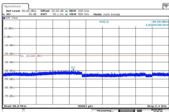
,Plot ,3Transmitter Spurious Emission : 2440,30MHz~2400MHz
