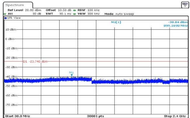
,Plot ,3Transmitter Spurious Emission : 2440,30MHz~2400MHz
