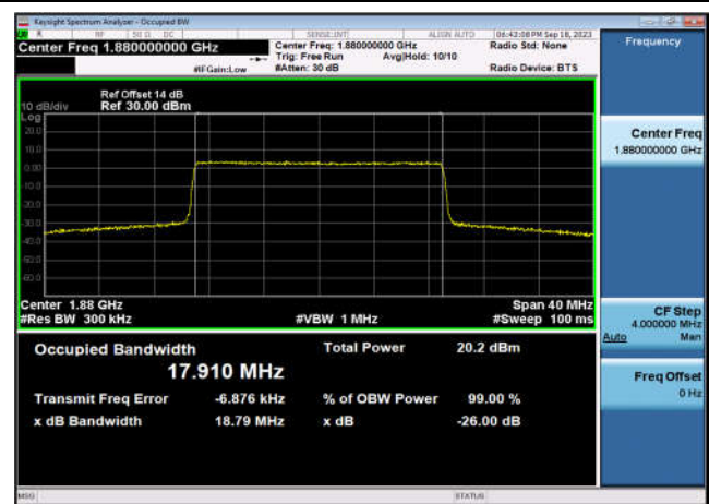
FDD02_MidRange_20_1880_Q16
