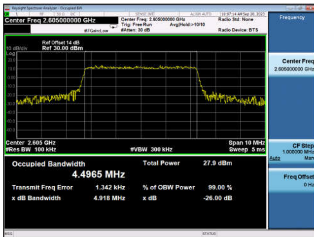
TDD41_MidRange_10_2605_QPSK
