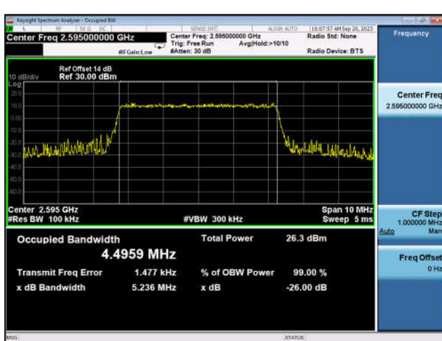
TDD38_MidRange_5_2595_QPSK
