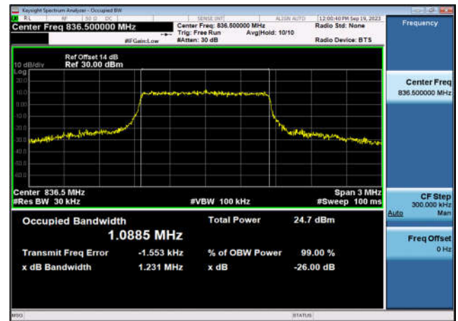
FDD05_MidRange_3_836.5_Q16
