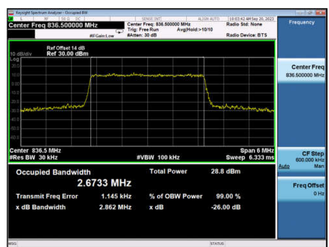
FDD05_MidRange_5_836.5_Q16
