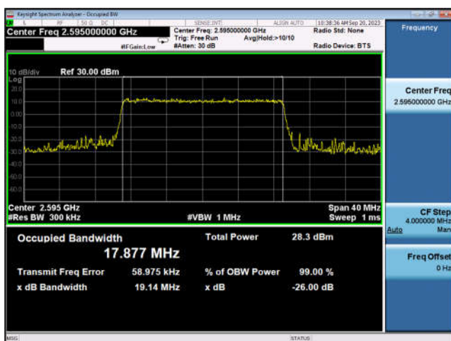
TDD38_MidRange_20_2595_QPSK
