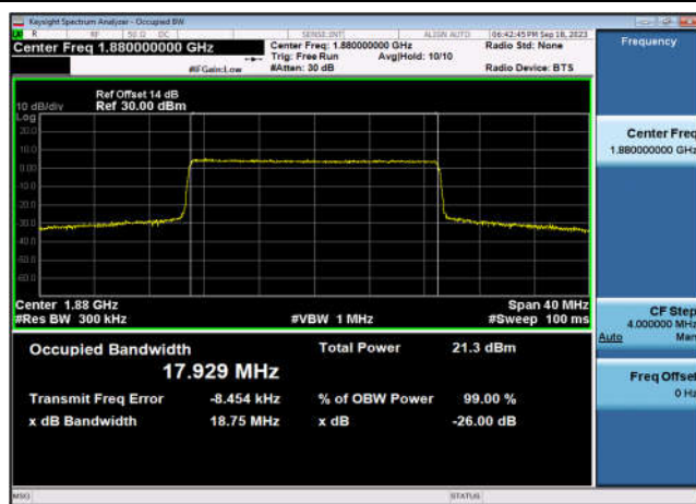
FDD02_MidRange_20_1880_QPSK
