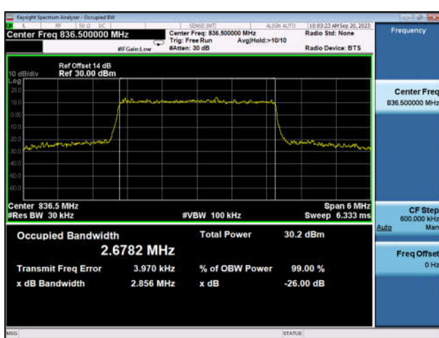
FDD05_MidRange_5_836.5_QPSK
