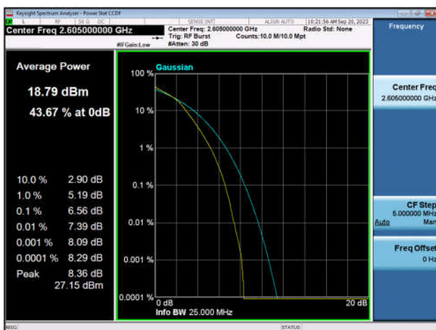
TDD41_MidRange_20MHz_2605_fullRB_Q16
