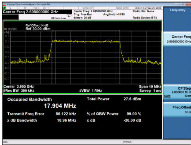
TDD41_MidRange_20_2605_QPSK
