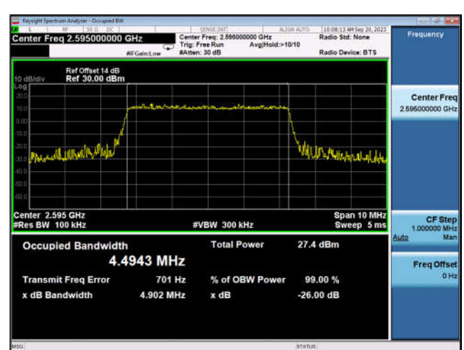
TDD38_MidRange_5_2595_Q16
