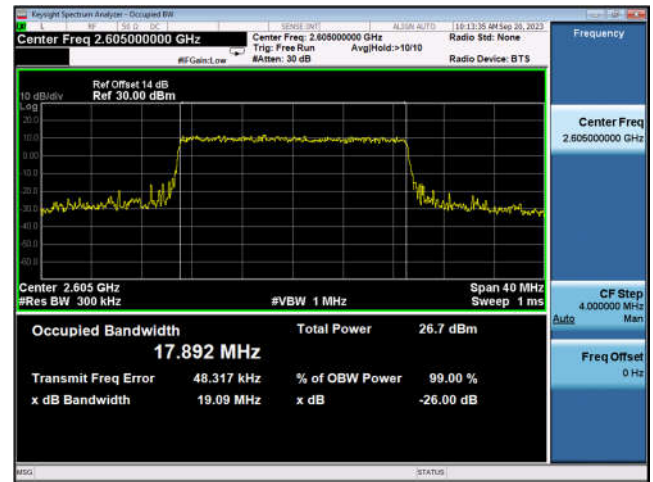
TDD41_MidRange_20_2605_Q16
