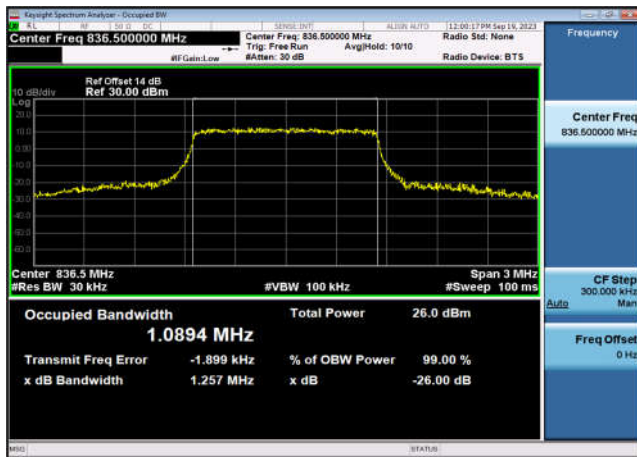
FDD05_MidRange_3_836.5_QPSK
