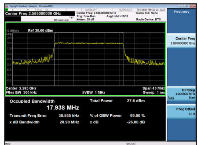
TDD38_MidRange_20_2595_Q16
