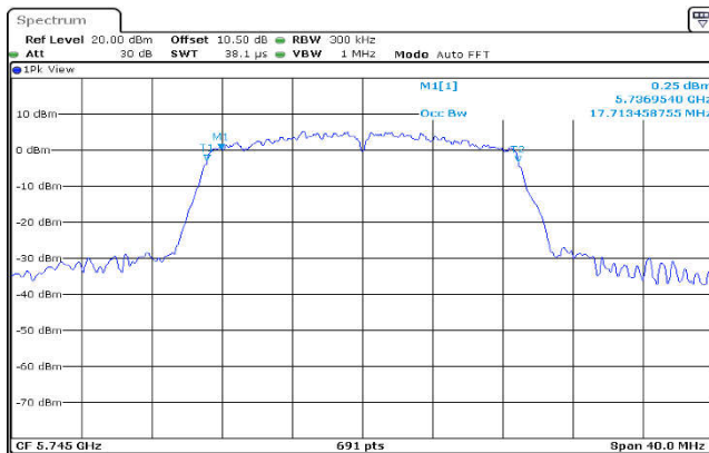
U-NII-3,802.11ac(20MHz),5745MHz ,Ant1
