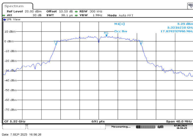
U-NII-2a,802.11n(20MHz),5320MHz ,Ant1
