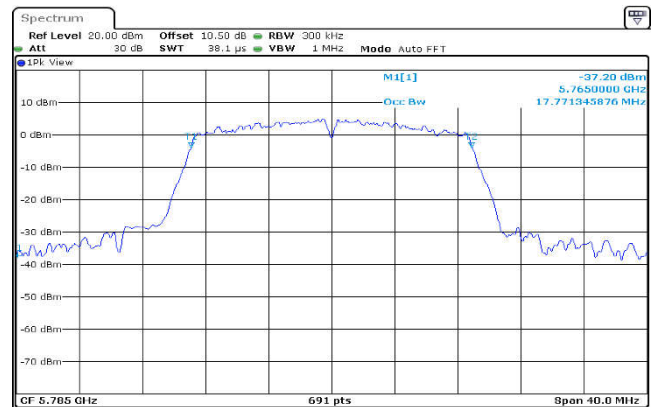
U-NII-3,802.11ac(20MHz),5785MHz ,Ant1
