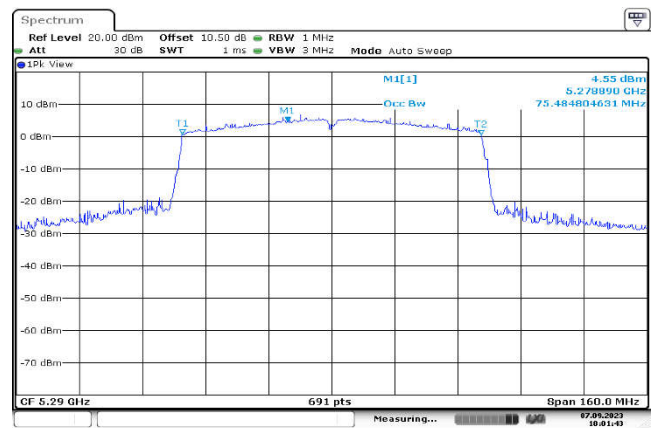
U-NII-2a,802.11ac(80MHz),5290MHz ,Ant1
