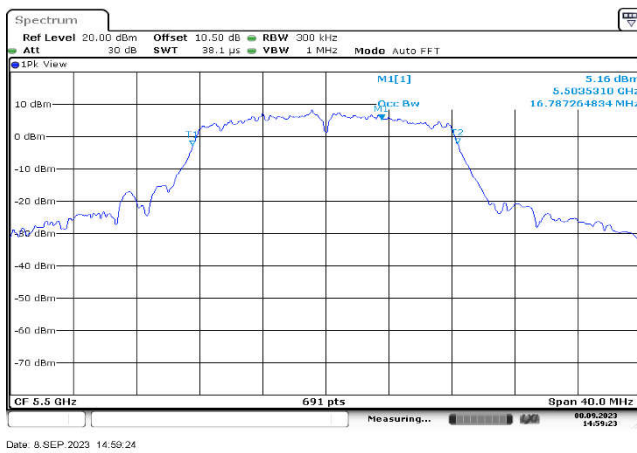
U-NII-2c,802.11a(20MHz),5500MHz ,Ant1
