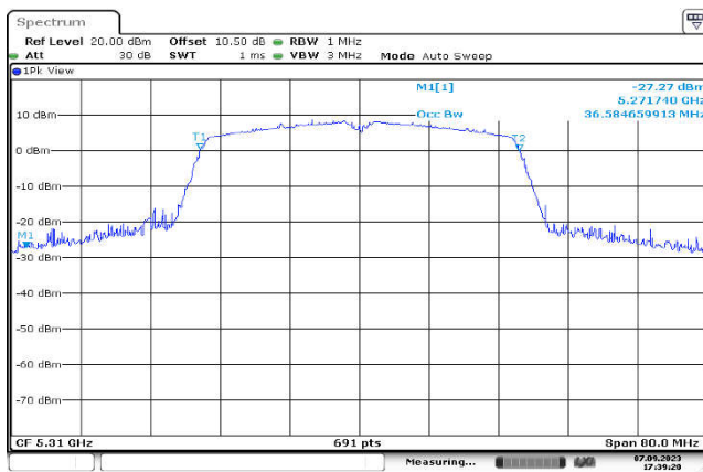
U-NII-2a,802.11ac(40MHz),5310MHz ,Ant1
