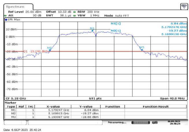
U-NII-1,802.11a(20MHz),5180MHz ,Ant1
