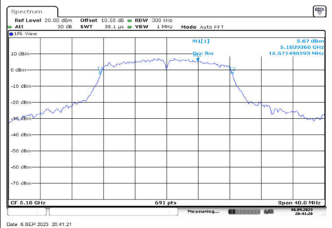
U-NII-1,802.11a(20MHz),5180MHz ,Ant1
