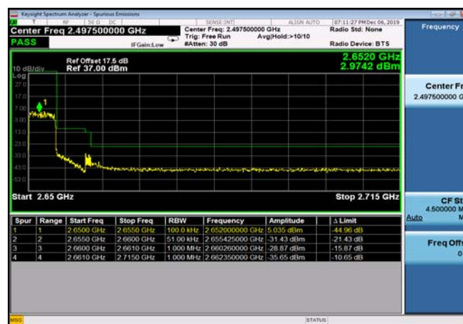
HighRange_TDD41_10MHz_2650_OneRB _high_QPSK
