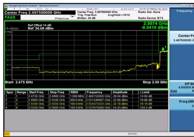
LowRange_TDD41_15MHz_2562.5_fullRB _low_QPSK
