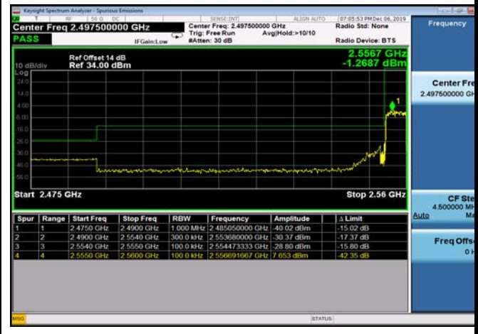
LowRange_TDD41_5MHz_2557.5_fullRB _LowQ16
