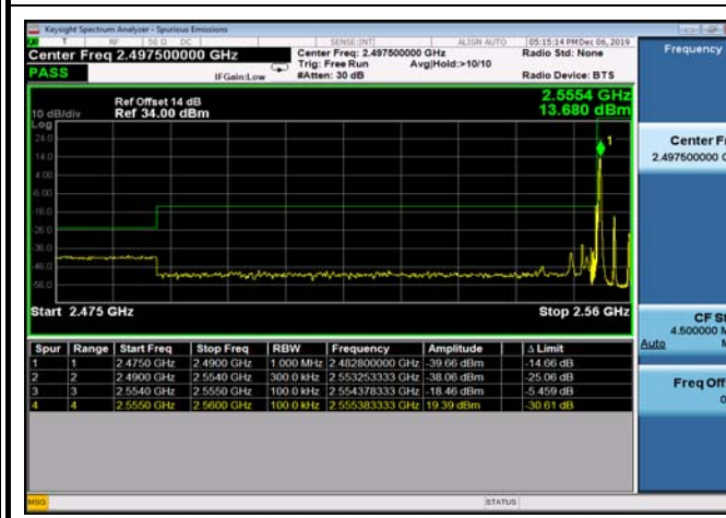
LowRange_TDD41_5MHz_2557.5_OneRB _low_QPSK
