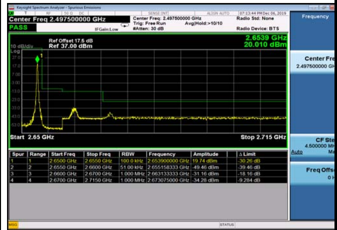
HighRange_TDD41_20MHz_2645_fullRB _HighQ16
