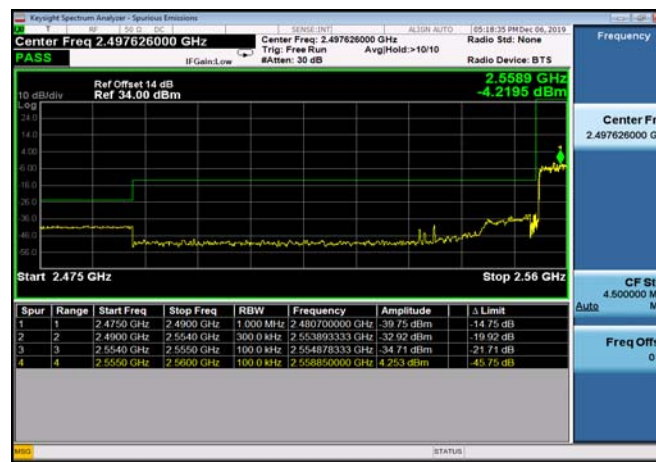
LowRange_TDD41_15MHz_2562.5_OneRB _low_QPSK
