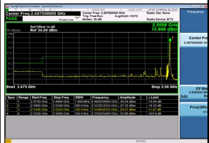
LowRange_TDD41_15MHz_2562.5_fullRB _low_Q16
