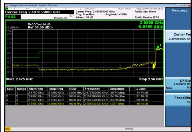
LowRange_TDD41_15MHz_2562.5_fullRB _low_Q16
