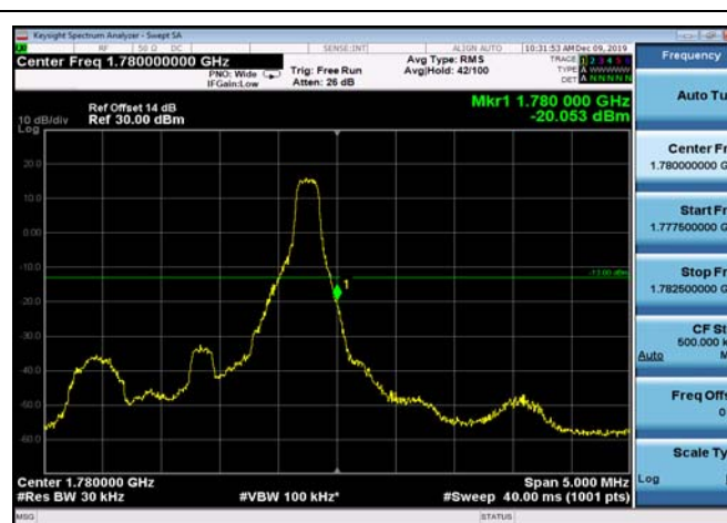
HighRange_FDD66_1.4MHz_1779.3 _fullRB_High_QPSK
