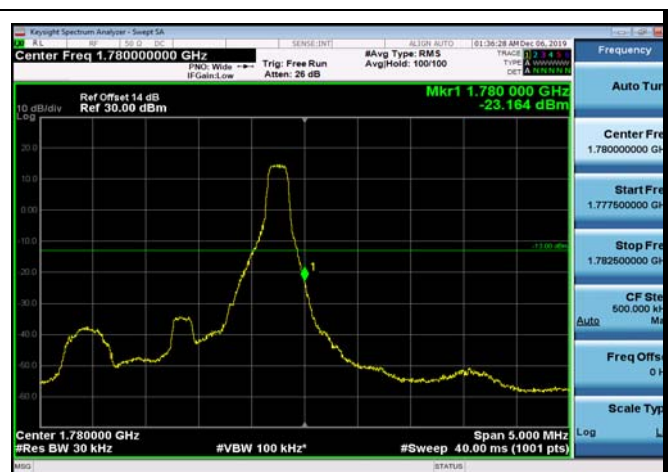
HighRange_FDD66_1.4MHz_1779.3 _fullRB_High_Q16
