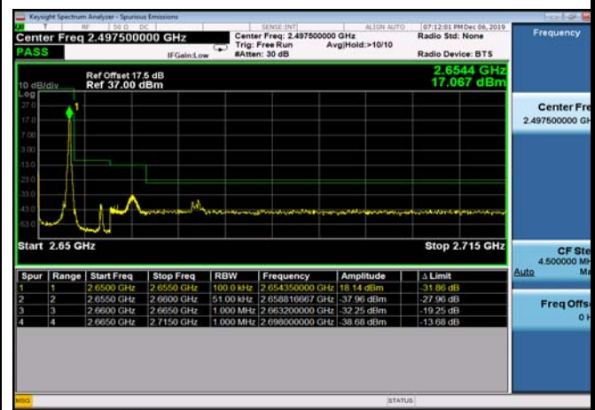
HighRange_TDD41_10MHz_2650_OneRB _high_Q16
