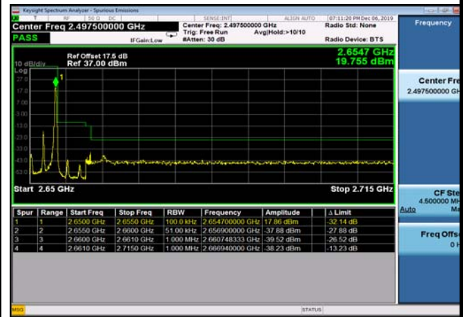
HighRange_TDD41_5MHz_2652.5_fullRB _HighQ16
