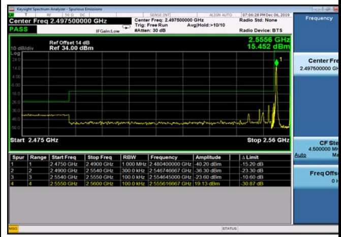
LowRange_TDD41_10MHz_2560_OneRB _low_Q16
