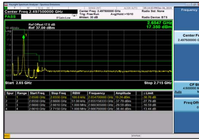
HighRange_TDD41_5MHz_2652.5_fullRB _HighQPSK
