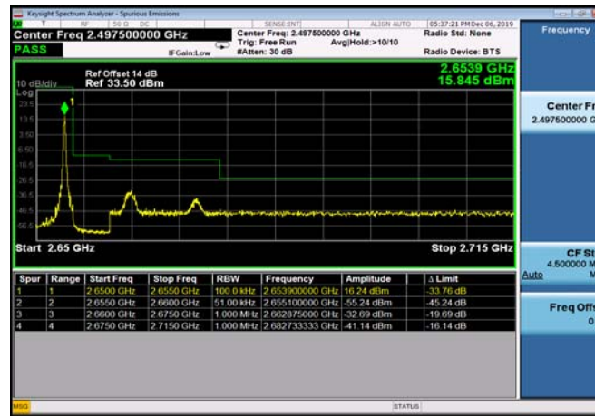
HighRange_TDD41_20MHz_2645_fullRB _HighQPSK
