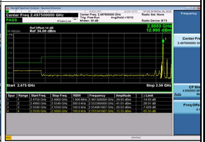
LowRange_TDD41_5MHz_2557.5_OneRB _low_Q16
