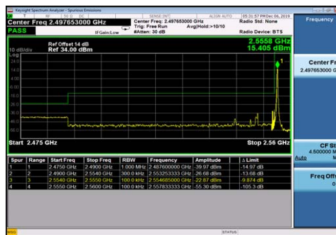
LowRange_TDD41_15MHz_2562.5_fullRB _low_QPSK
