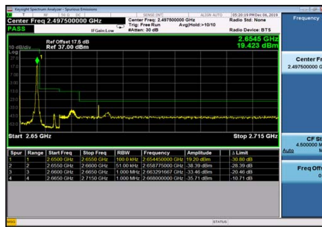
HighRange_TDD41_10MHz_2650_OneRB _high_QPSK
