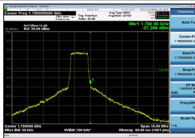
HighRange_FDD66_3MHz_1778.5_OneRB _high_QPSK
