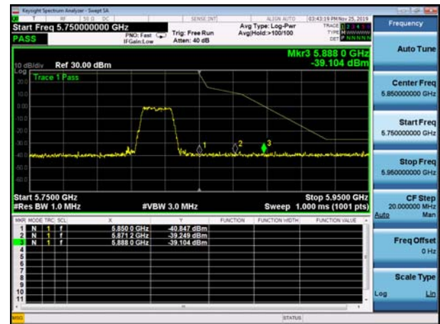
U-NII-3 Band Edge-802.11n(40MHz) ,5795MHz
