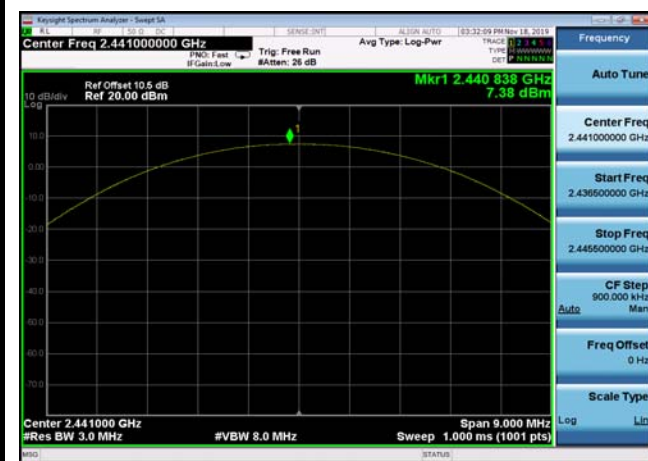
Output Power: DQPSK,2441MHz,2DH5
