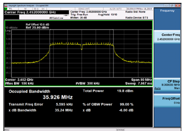
6dB Bandwidth-802.11n(HT40),2452MHz
