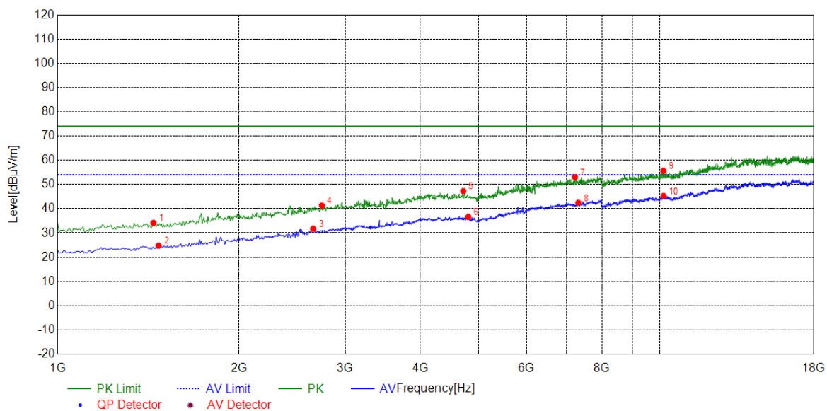
(Plot N: Test Antenna Vertical 1G – 18G)
