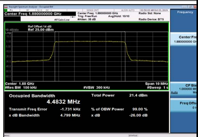
FDD02_MidRange_5_1880_Q16
