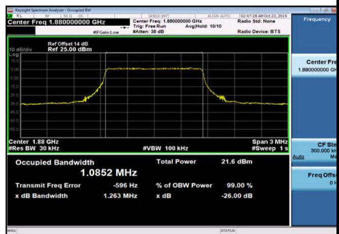
FDD02_MidRange_3_1880_Q16
