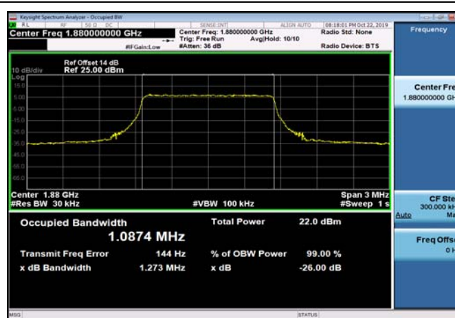
FDD02_MidRange_3MHz_1880MHz_Q16
