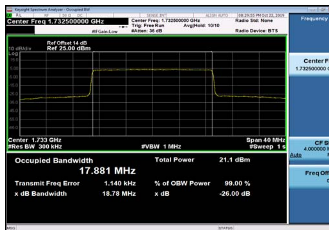
FDD04_MidRange_20MHz_1732.5MHz _Q16
