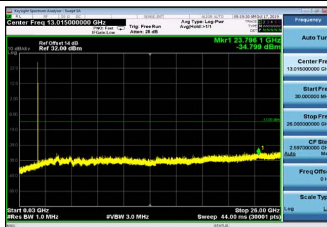
FDD04_HighRange_1.4MHz_30MHz~26GHz
