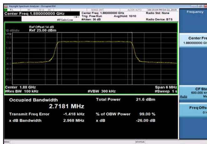
FDD02_MidRange_5MHz_1880MHz_Q16
