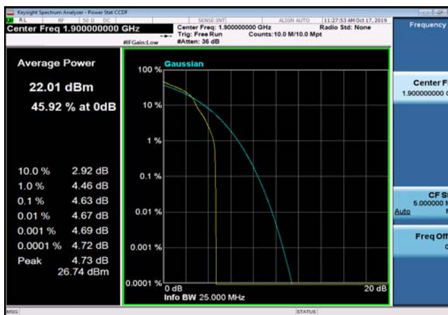
FDD02_HighRange_20MHz_1900_OneRB _high_Q16
