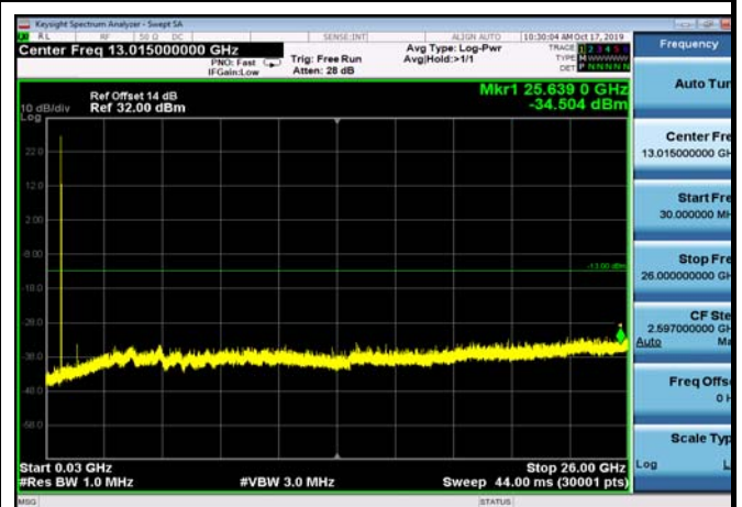
FDD12_MidRange_3MHz_30MHz~26GHz
