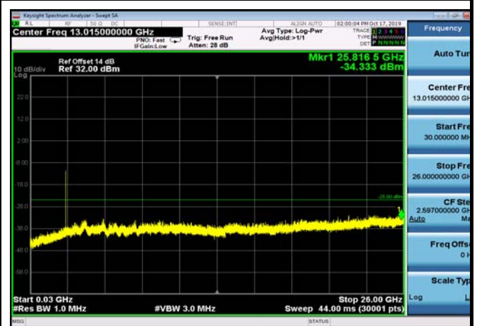
TDD41_MidRange_10MHz_30MHz~26GHz
