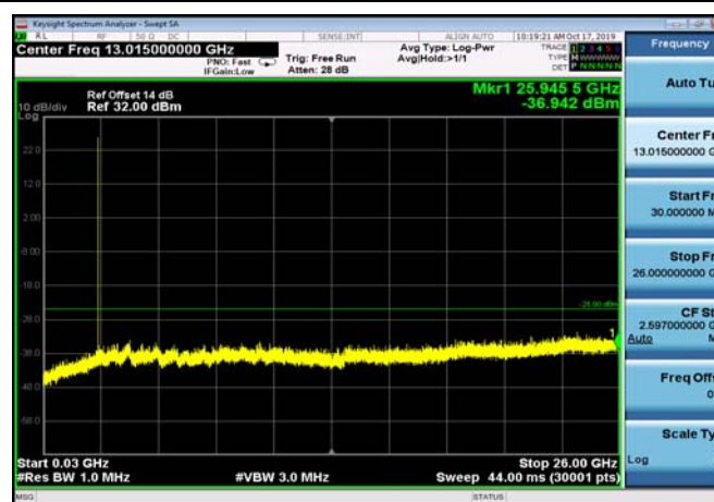
FDD07_MidRange_15MHz_30MHz~26GHz
