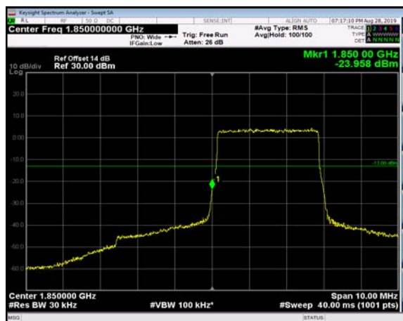
LowRange_FDD02_5MHz_1852.5_OneRB _low_QPSK
