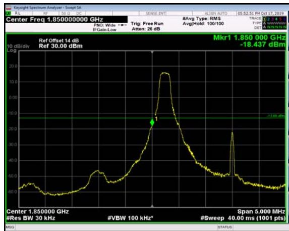
LowRange_FDD02_3MHz_1851.5_fullRB _Low_QPSK
