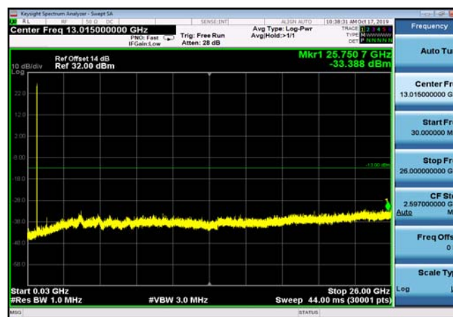
FDD17_LowRange_5MHz_30MHz~26GHz
