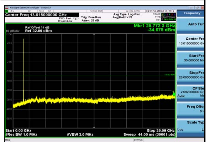
FDD04_HighRange_30MHz_30MHz~26GHz
