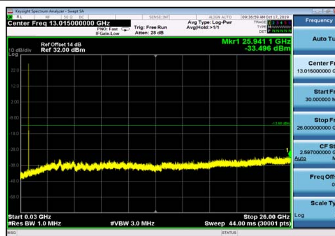
FDD07_HighRange_15MHz_30MHz~26GHz
