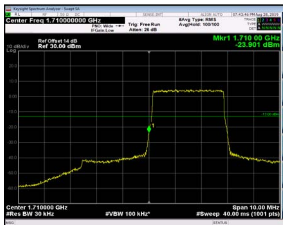
LowRange_FDD04_5MHz_1712.5_OneRB _low_QPSK
