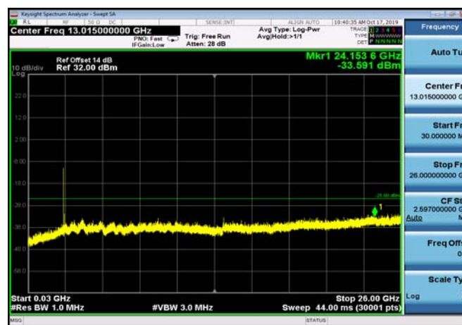
TDD41_MidRange_15MHz_30MHz~26GHz
