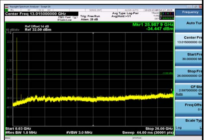
FDD12_MidRange_1.4MHz_30MHz~26GHz
