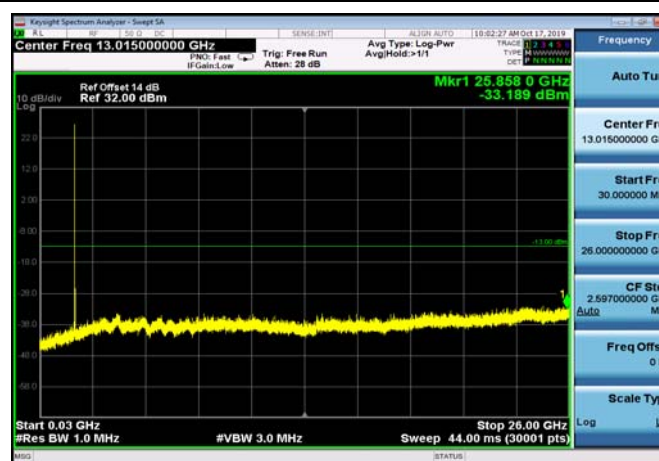
FDD04_HighRange_5MHz_30MHz~26GHz
