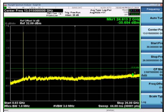
TDD41_LowRange_10MHz_30MHz~26GHz
