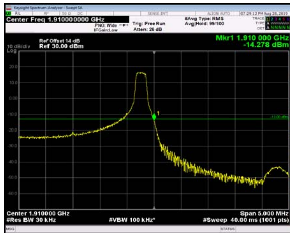
HighRange_FDD02_3MHz_1908.5_fullRB _High_QPSK
