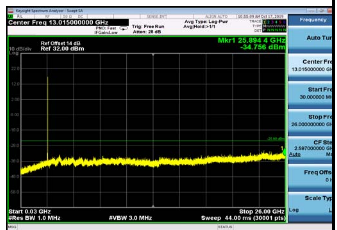
TDD41_HighRange_20MHz_30MHz~26GHz
