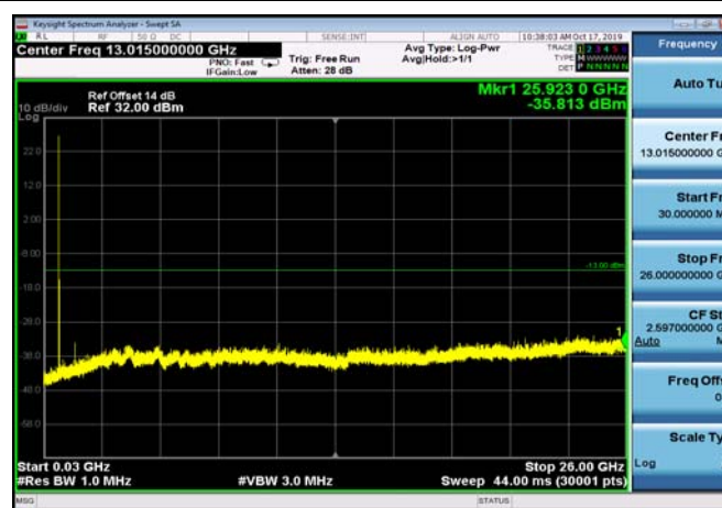
TDD41_HighRange_15MHz_30MHz~26GHz
