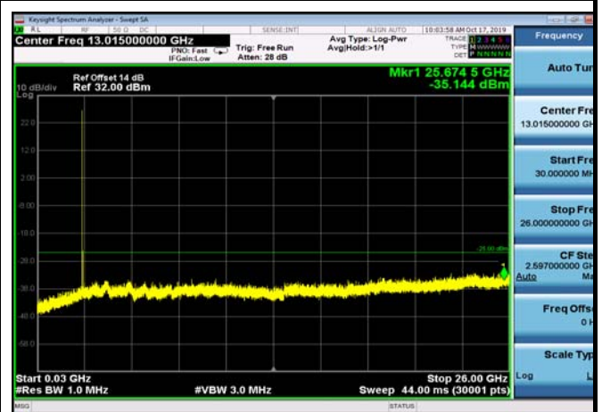
FDD07_MidRange_10MHz_30MHz~26GHz
