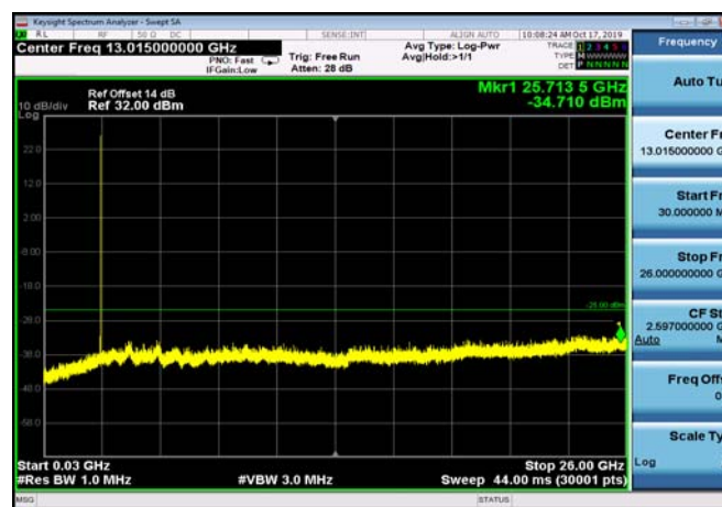
FDD07_HighRange_5MHz_30MHz~26GHz
