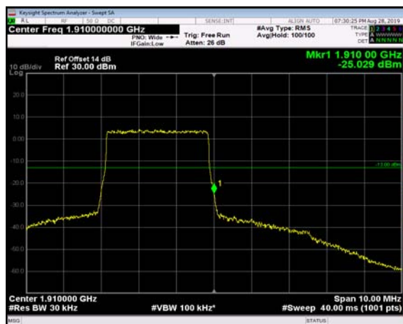
HighRange_FDD02_5MHz_1907.5_OneRB _high_QPSK
