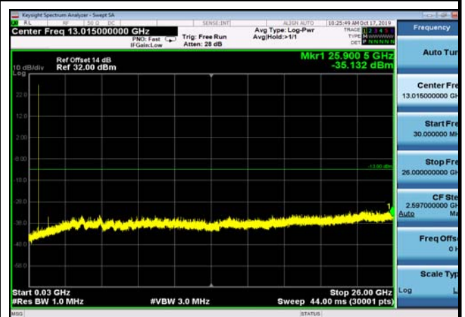
FDD12_LowRange_1.4MHz_30MHz~26GHz
