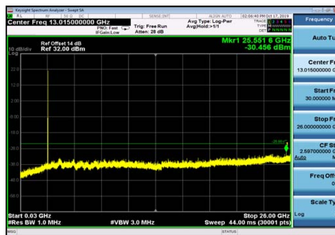
TDD41_HighRange_5MHz_30MHz~26GHz
