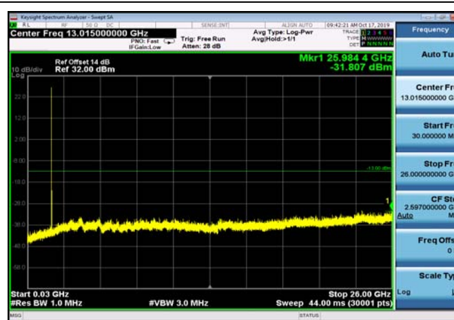
FDD04_HighRange_20MHz_30MHz~26GHz
