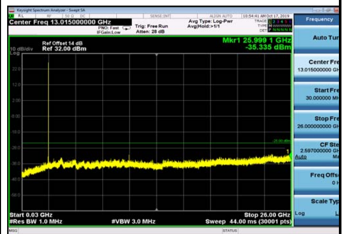
TDD41_MidRange_20MHz_30MHz~26GHz
