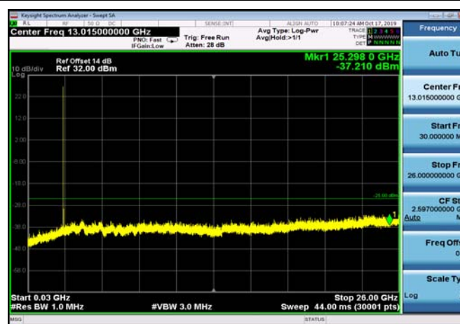
FDD07_LowRange_5MHz_30MHz~26GHz
