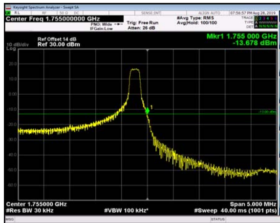
HighRange_FDD04_3MHz_1753.5_fullRB _High_QPSK
