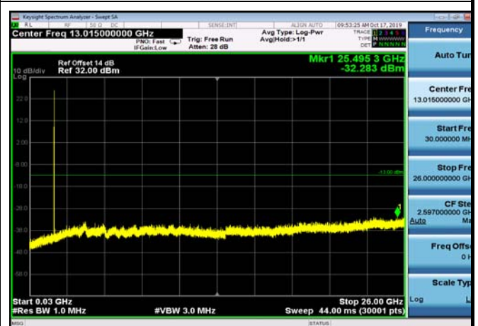
FDD04_MidRange_15MHz_30MHz~26GHz
