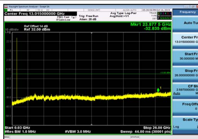
FDD05_LowRange_5MHz_30MHz~26GHz
