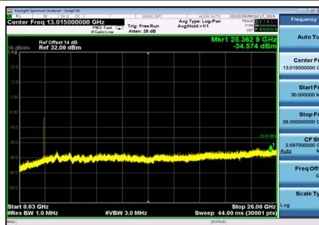
TDD41_LowRange_5MHz_30MHz~26GHz
