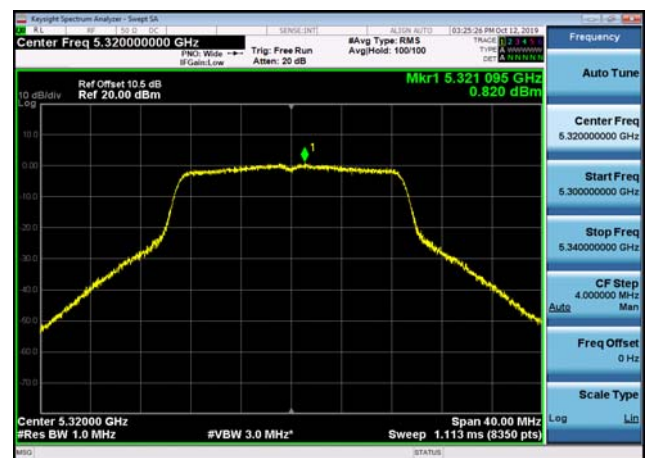
U-NII-2a Power spectral density-802.1 1ac(20MHz),5320MHz,Ant2
