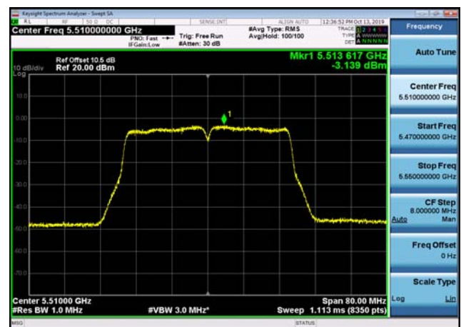
U-NII-2c Power spectral density-802.1 1ac(40MHz),5510MHz,Ant2
