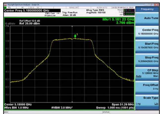
U-NII-1 Power spectral density-802.11 a(20MHz),5180MHz,Ant2
