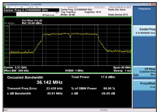
U-NII-2a 26dB Bandwidth-802.11n(40MHz ) ,5310MHz,Ant2
