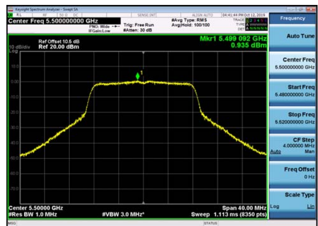
U-NII-2c Power spectral density-802.1 1a(20MHz),5500MHz,Ant2
