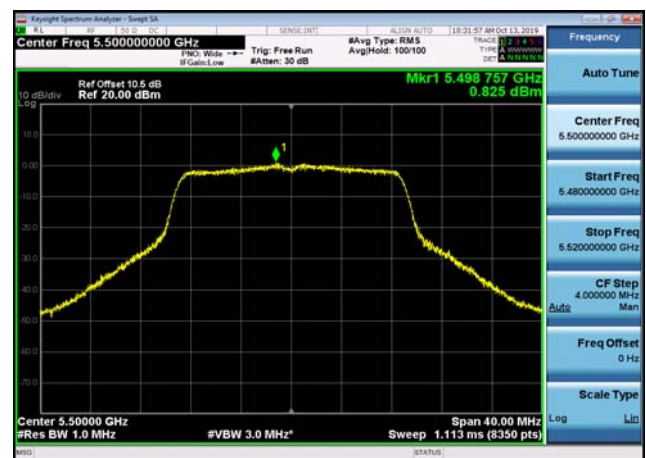
U-NII-2c Power spectral density-802.1 1ac(20MHz),5500MHz,Ant2
