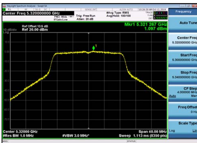
U-NII-2a Power spectral density-802.1 1ac(20MHz),5320MHz,Ant1
