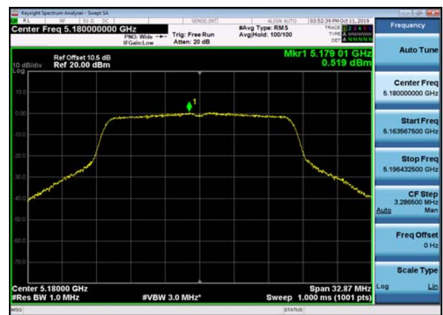
U-NII-1 Power spectral density-802.11 ac(20MHz),5180MHz,Ant2
