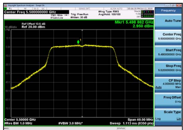
U-NII-2c Power spectral density-802.1 1n(20MHz),5500MHz,Ant2
