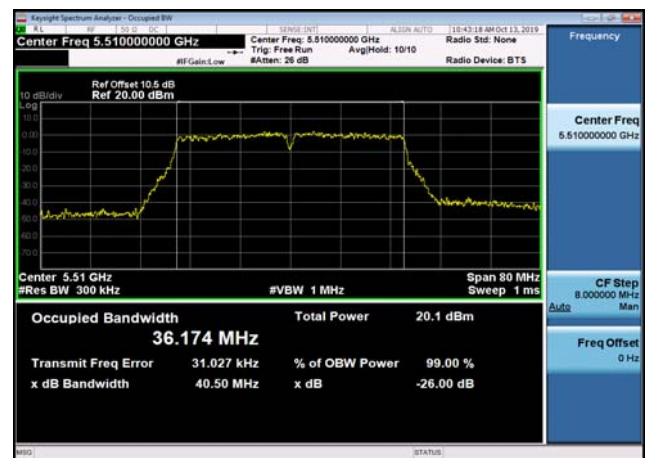
U-NII-2c 26dB Bandwidth-802.11n(40MHz) ,5510MHz,Ant2
