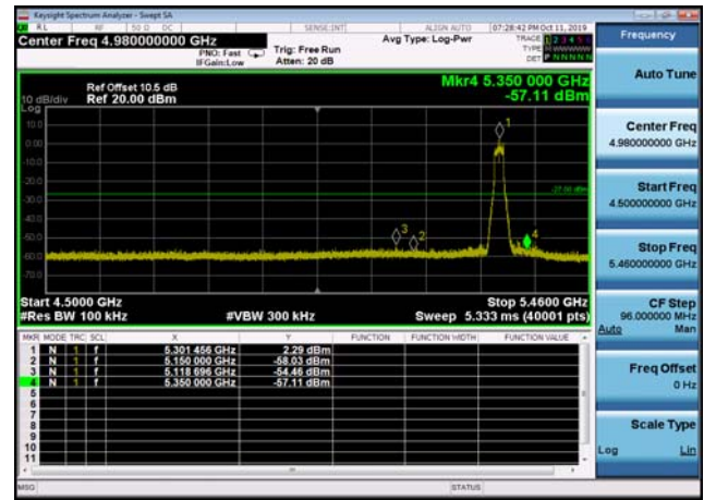
U-NII-2a ,Plot 1,Band Edge-802.11a(20 MHz),5320MHz,Ant2
