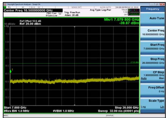
U-NII-2a ,Plot 4,7000MHz~26000MHz-802 .11n(40MHz),5310MHz,Ant2
