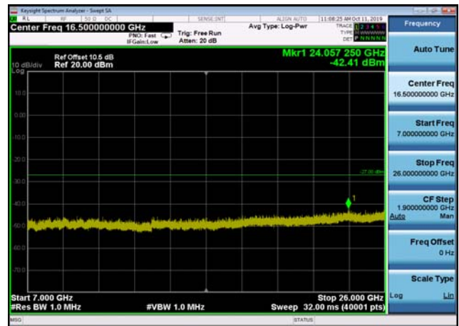
U-NII-1 ,Plot 4,7000MHz~26000MHz-802. 11a(20MHz),5240MHz,Ant2
