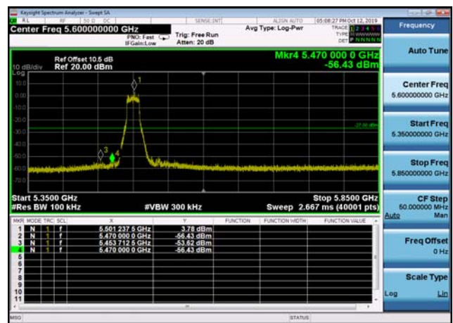
U-NII-2c ,Plot 1,Band Edge-802.11n(20 MHz),5500MHz,Ant2
