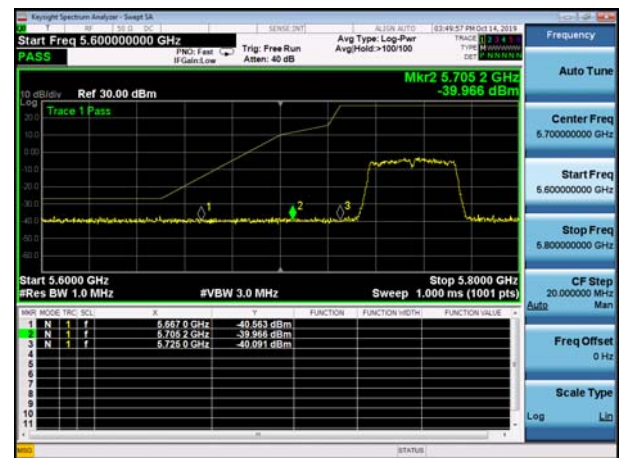
U-NII-3 ,Plot 1,Band Edge-802.11n(40M Hz),5755MHz,Ant2
