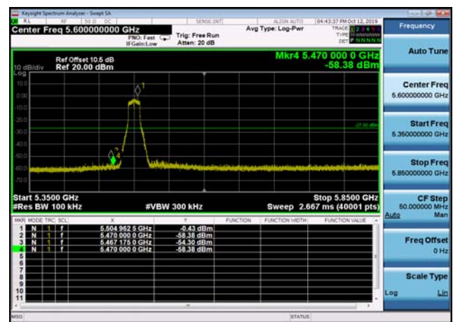
U-NII-2c ,Plot 1,Band Edge-802.11a(20 MHz),5500MHz,Ant2
