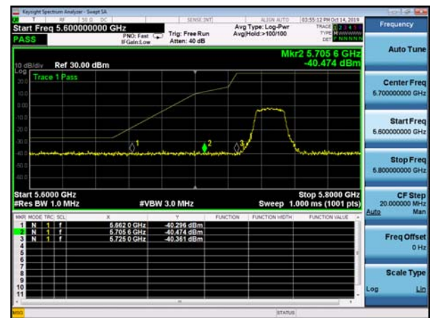
U-NII-3 ,Plot 1,Band Edge-802.11n(20M Hz),5745MHz,Ant2
