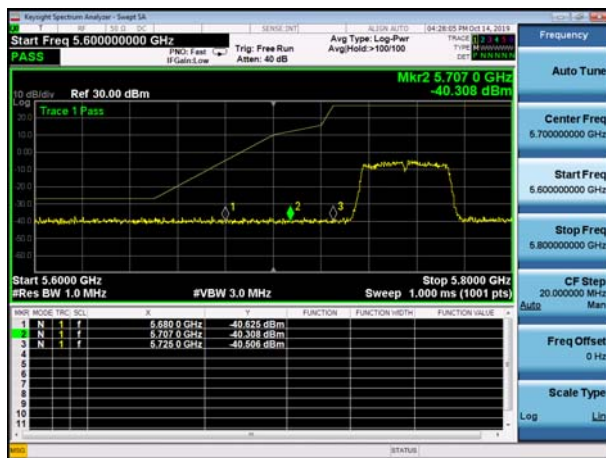
U-NII-3 ,Plot 1,Band Edge-802.11n(40M Hz),5755MHz,Ant1
