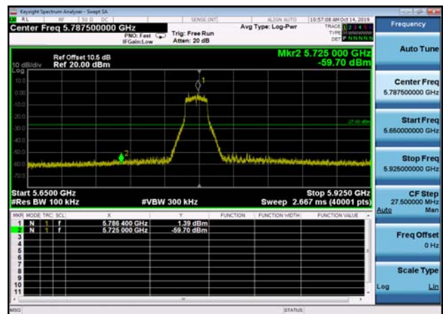
U-NII-3 ,Plot 1,Band Edge-802.11ac(20 MHz),5785MHz,Ant2
