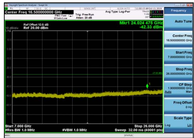
U-NII-2c ,Plot 4,7000MHz~26000MHz-802 .11n(40MHz),5670MHz,Ant2
