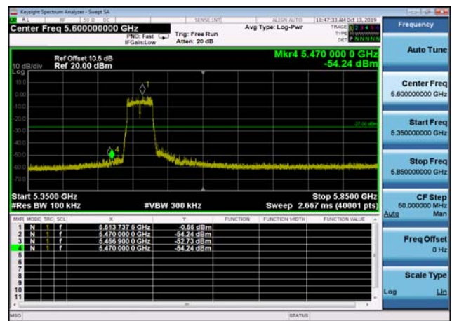
U-NII-2c ,Plot 1,Band Edge-802.11n(40 MHz),5510MHz,Ant2
