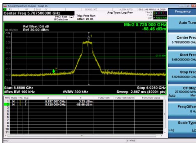
U-NII-3 ,Plot 1,Band Edge-802.11a(20M Hz),5785MHz,Ant2
