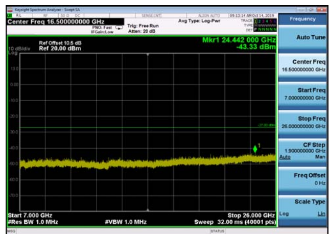
U-NII-3 ,Plot 4,7000MHz~26000MHz-802. 11a(20MHz),5785MHz,Ant2
