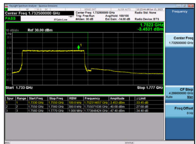
FDD4-20MHz-16QAM-HCH-100RB#0
