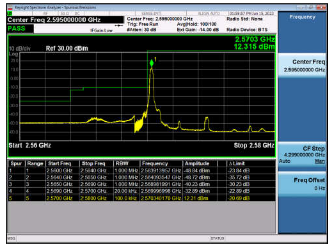
FDD38-5MHz-16QAM-LCH-25RB#0
