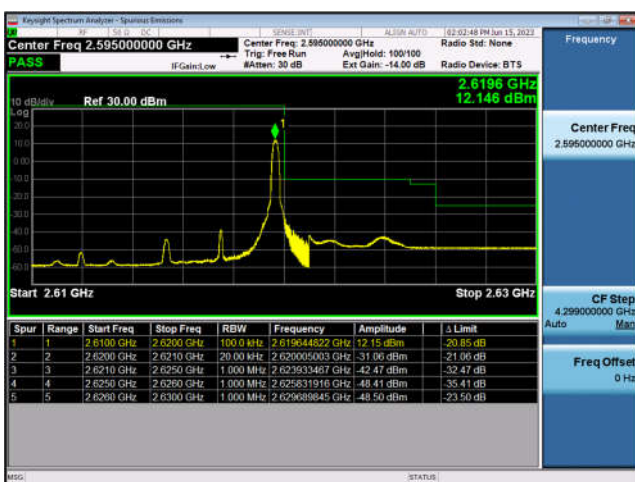
FDD38-5MHz-QPSK-HCH-1RB#24
