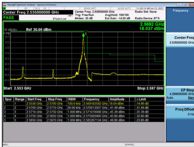
FDD7-15MHz-QPSK-HCH-75RB#0
