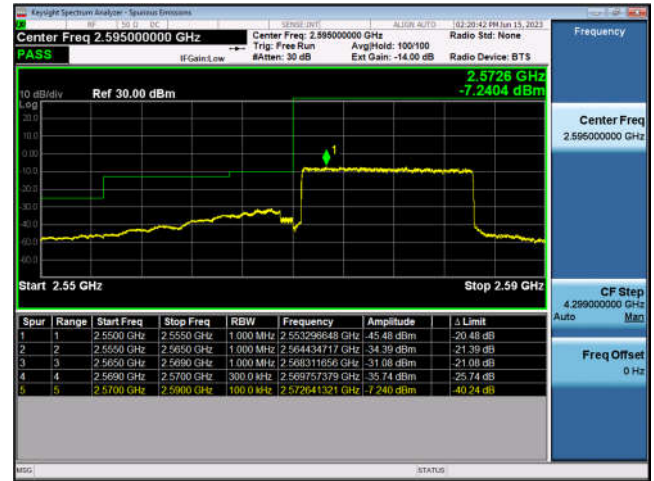
FDD38-15MHz-16QAM-HCH-1RB#74
