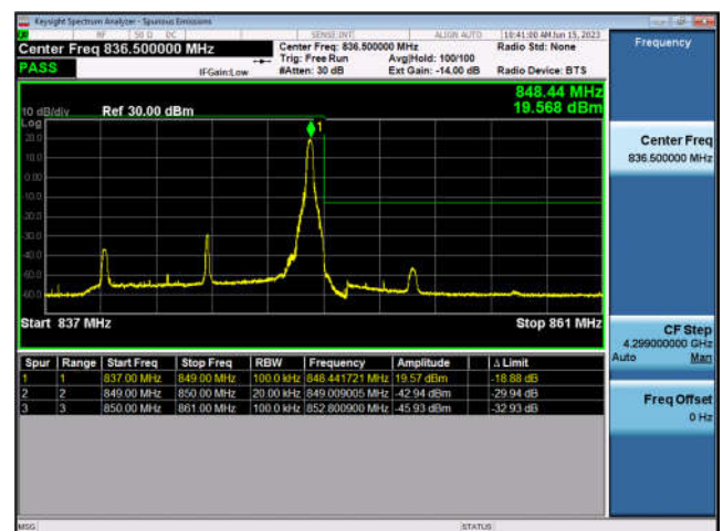
FDD5-10MHz-16QAM-HCH-1RB#49
