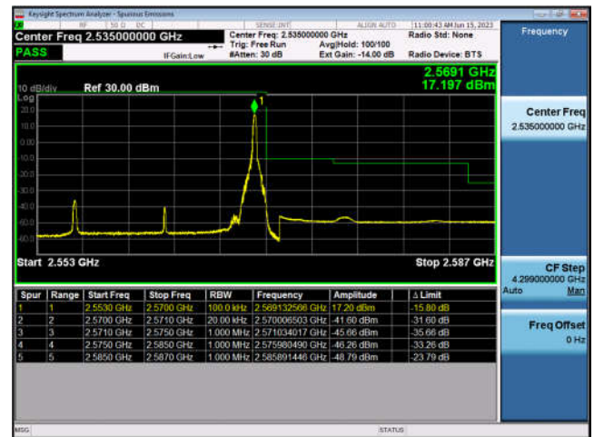
FDD7-15MHz-16QAM-HCH-75RB#0
