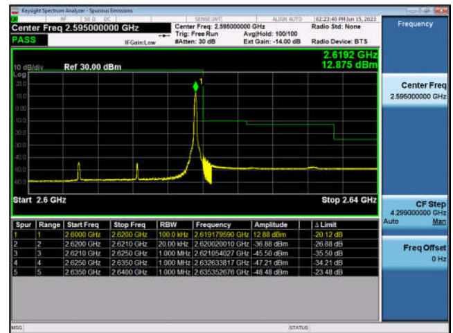
FDD38-15MHz-16QAM-HCH-75RB#0
