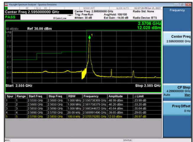
FDD38-10MHz-16QAM-LCH-50RB#0
