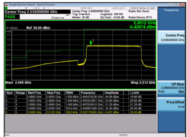
FDD7-10MHz-16QAM-LCH-50RB#0
