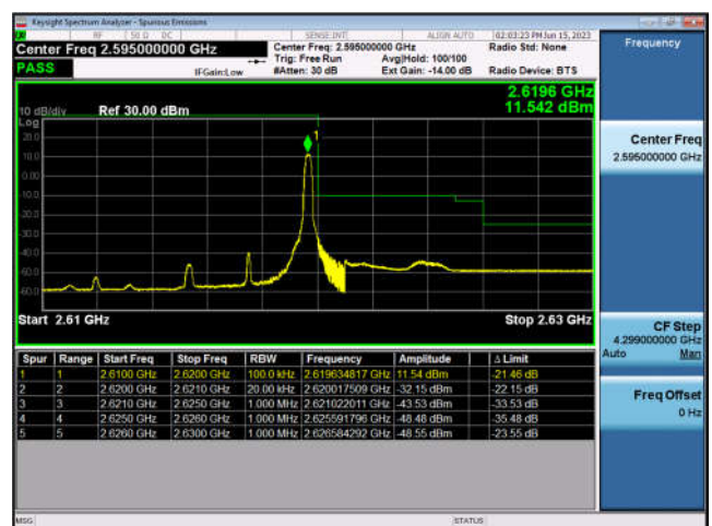
FDD38-5MHz-16QAM-HCH-1RB#24
