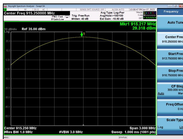
Conducted Output Power: 915.25MHz
