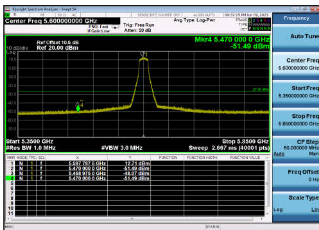
U-NII-2c ,Plot 1,Band Edge-802.11ac(20 MHz),5600MHz,Ant1
