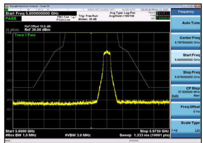
U-NII-3 ,Plot 1,Band Edge-802.11ac(20 MHz),5785MHz,Ant1
