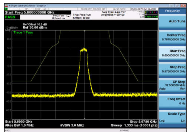
U-NII-3 ,Plot 1,Band Edge-802.11n(20M Hz),5785MHz,Ant1
