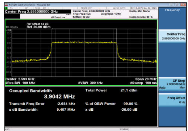
TDD41_MidRange_15_2593_Q16
