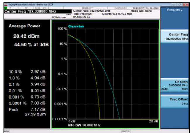
FDD13_MidRange_10MHz_782_fullRB _Q16
