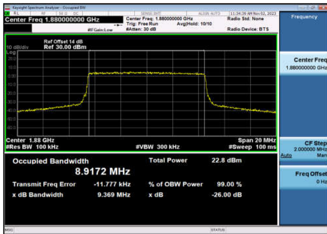
FDD02_MidRange_15_1880_QPSK
