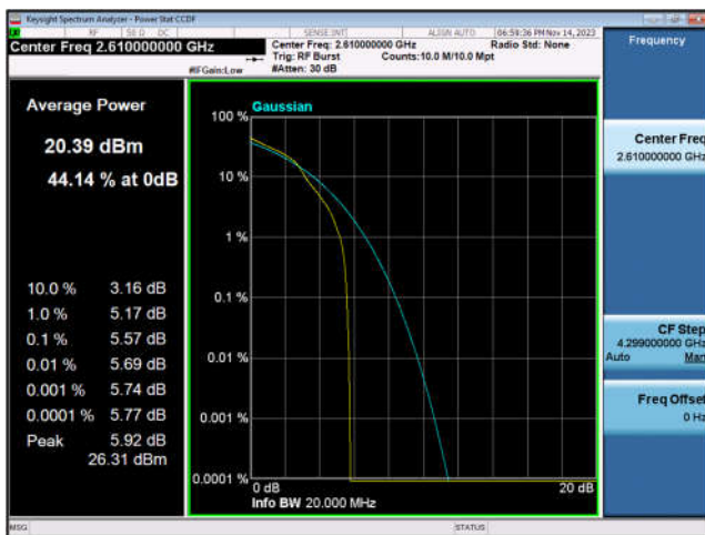
TDD38_HighRange_20MHz_2610_OneRB _high_Q16
