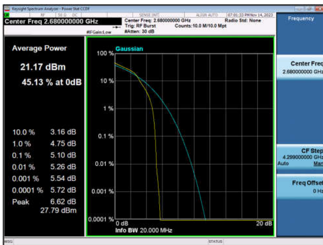
TDD41_HighRange_20MHz_2680_OneRB _high_Q16
