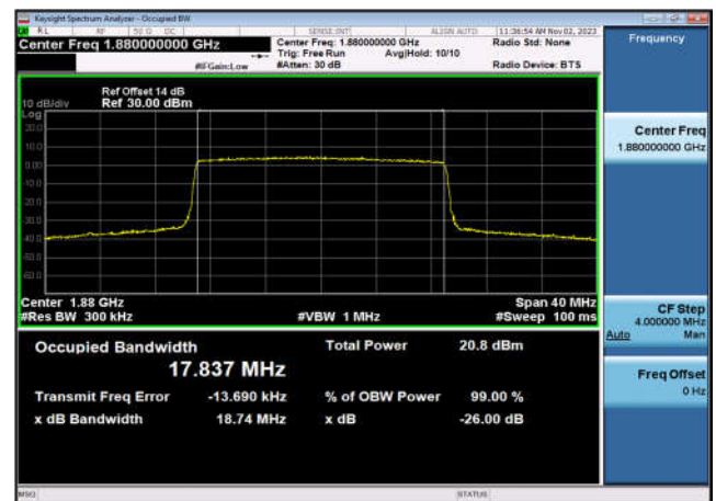
FDD02_MidRange_20_1880_Q16
