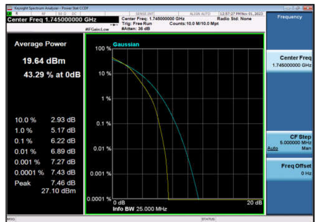
FDD04_HighRange_20MHz_1745_fullIRB _Q16
