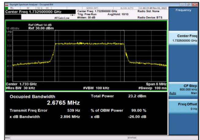
FDD04_MidRange_5_1732.5_Q16
