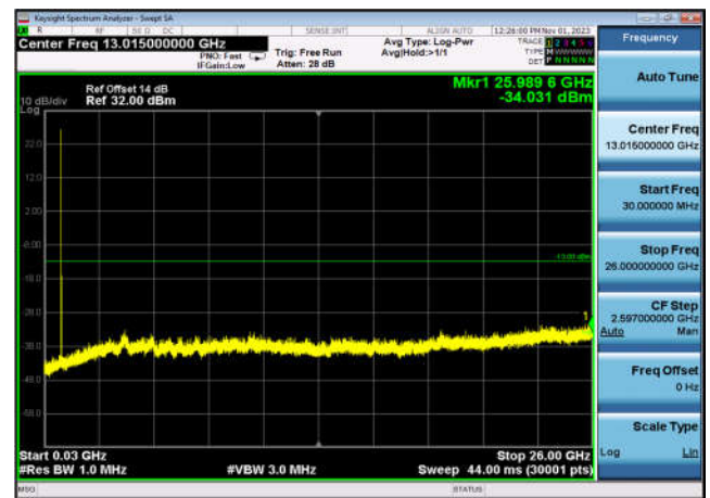
FDD07_LowRange_20MHz_30MHz~26GHz
