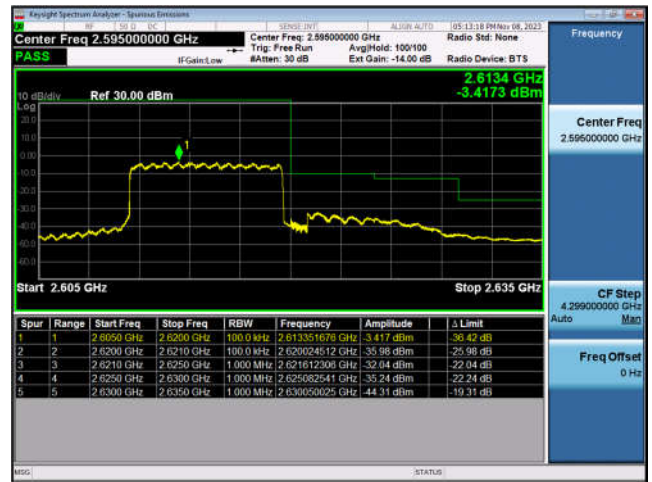
LTE Band 38-15MHz-QPSK-LCH-75RB#0
