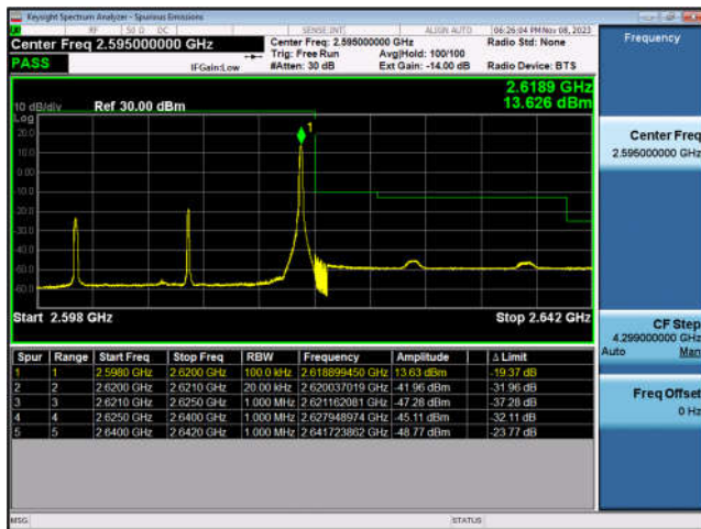
LTE Band 38-20MHz-QPSK-HCH-1RB#99
