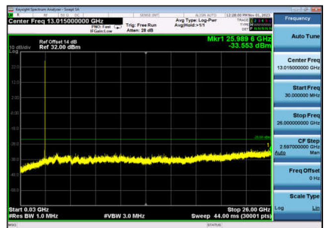
FDD07_HighRange_10MHz_30MHz~26GHz
