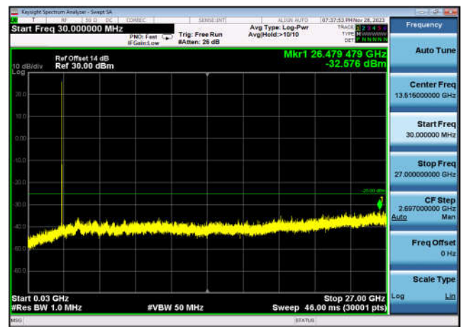
TDD38_HighRange_20MHz_30MHz~27GHz
