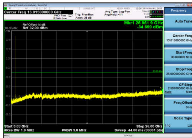
FDD12_HighRange_10MHz_30MHz~26GHz
