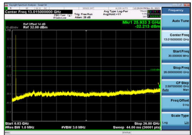
FDD13_LowRange_10MHz_30MHz~26GHz
