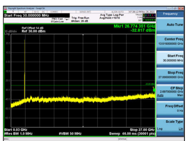
TDD38_HighRange_20MHz_30MHz~27GHz
