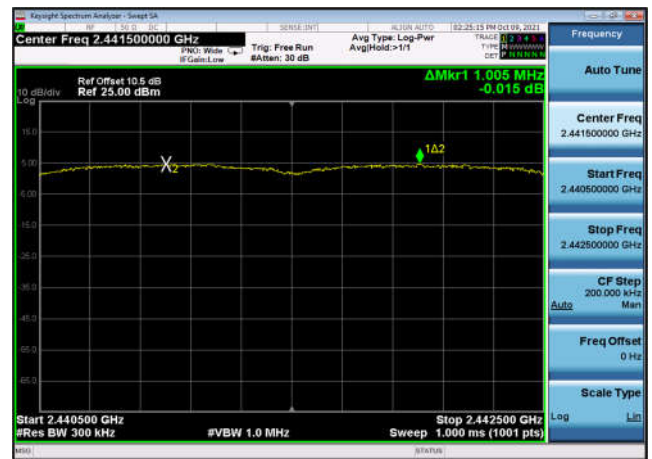
8DPSK,Hopping3DH5,2440.5~2442.5
