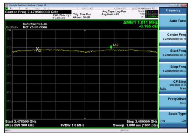
DQPSK,Hopping2DH5,2478.5~2480.5
