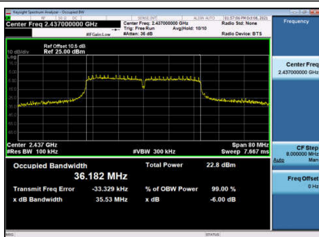
6dB Bandwidth-802.11n(HT40),2437MHz
