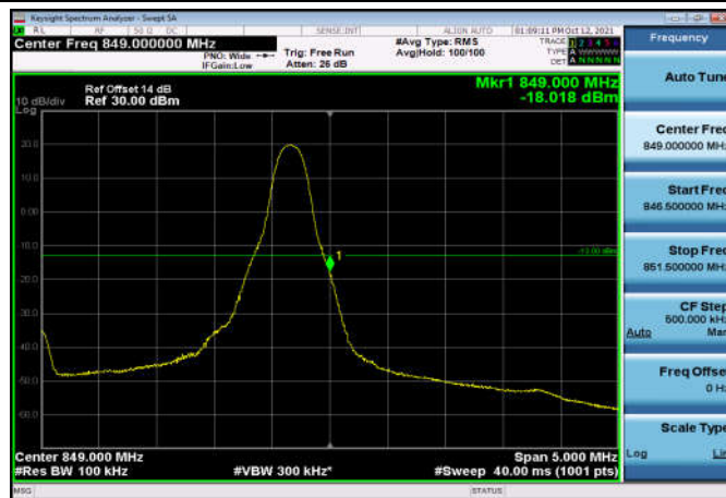
HighRange_FDD26_5MHz_846.5_OneRB _high_QPSK
