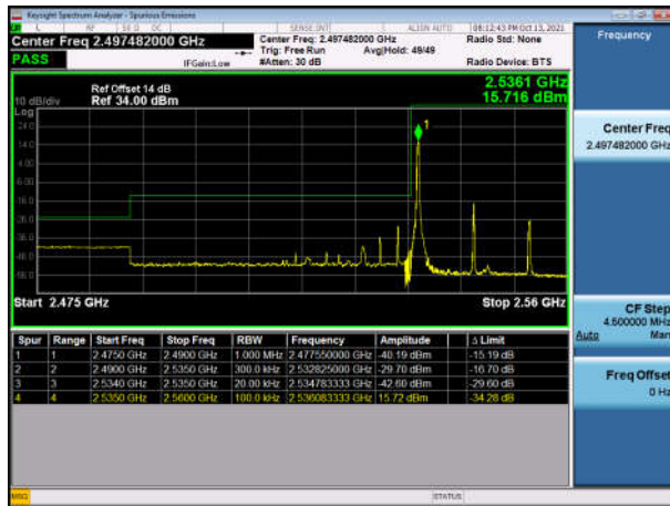
TDD41_20M Low FullRB QPSK
