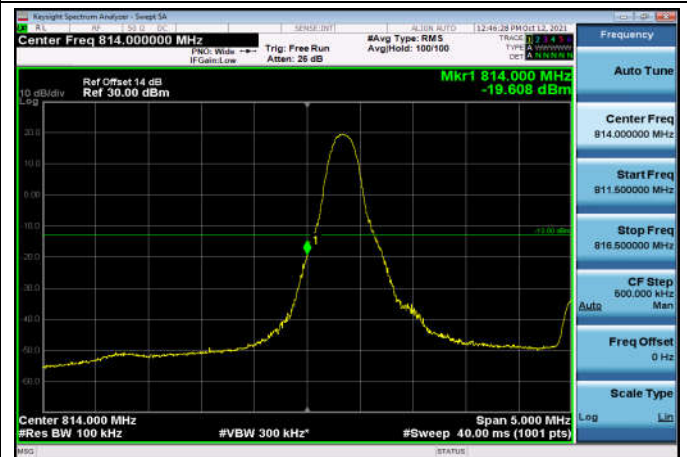
LowRange_FDD26_5MHz_816.5_fullRB _Low_Q16
