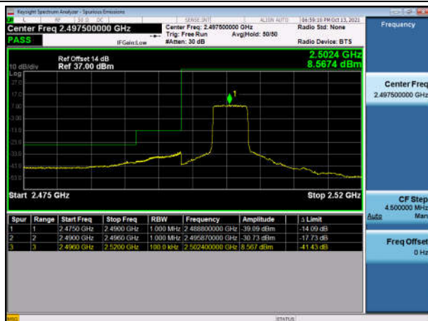
TDD7_5M Low FullIRB QPSK
