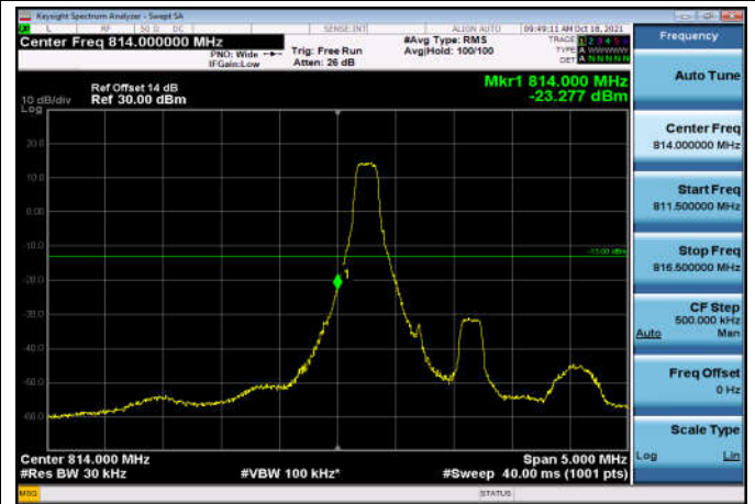
LowRange_FDD26_1.4MHz_814.7_fullRB _Low_Q16
