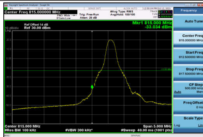
LowRange_ FDD26_10MHz_820_fullRB Low QPSK
