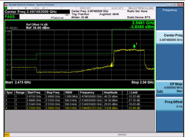
TDD41_20M High oneRB 16Q
