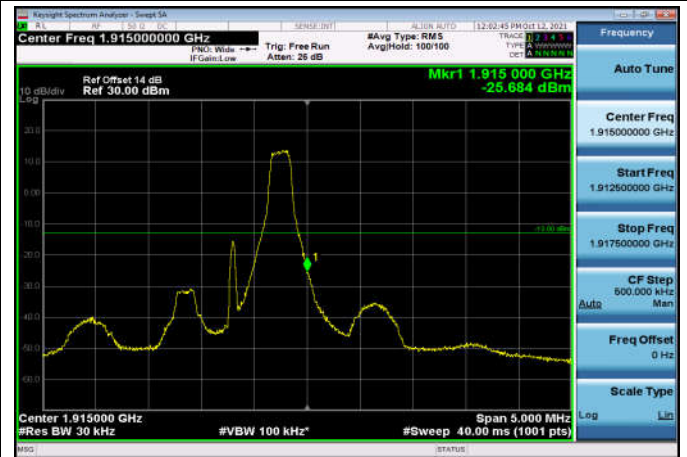
HighRange_FDD25_1.4MHz_1914.3 _fullRB_High_Q16
