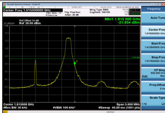
HighRange_FDD25_3MHz_1913.5_OneRB _high_QPSK
