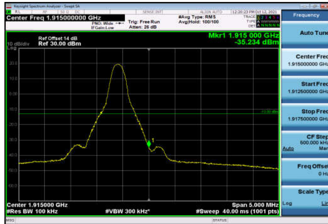
HighRange_FDD25_10MHz_1910_fullRB _High_QPSK
