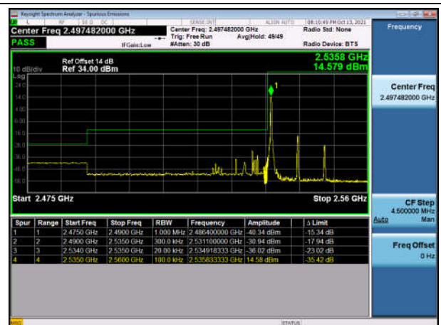
TDD41_15M Low oneRB 16Q
