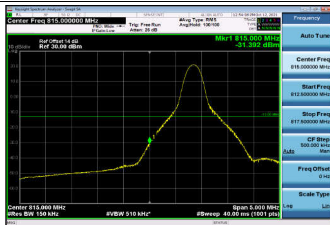
LowRange_FDD26_15MHz_822.5_OneRB low QPSK
