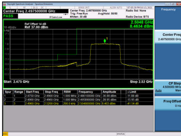
TDD7_10M High oneRB QPSK
