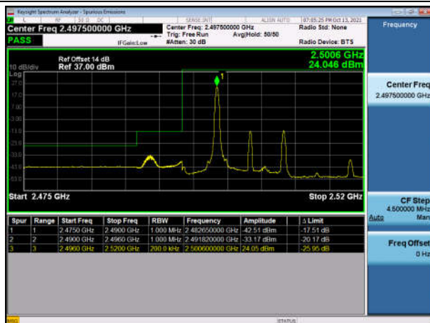
TDD7_10M Low oneRB QPSK
