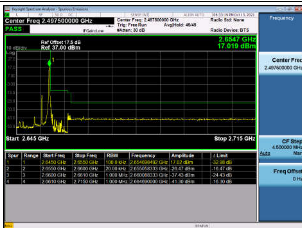
TDD41_5M High oneRB QPSK
