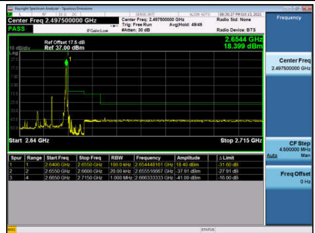
TDD41_10M High FullRB 16Q
