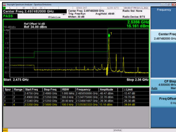
TDD41_10M Low FullIRB QPSK
