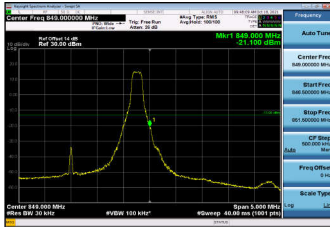
HighRange_FDD26_3MHz_847.5_fullRB _High_QPSK
