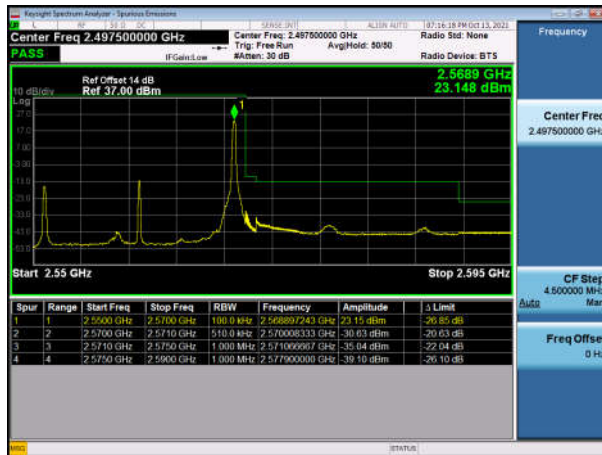
TDD7_20M High FullIRB QPSK
