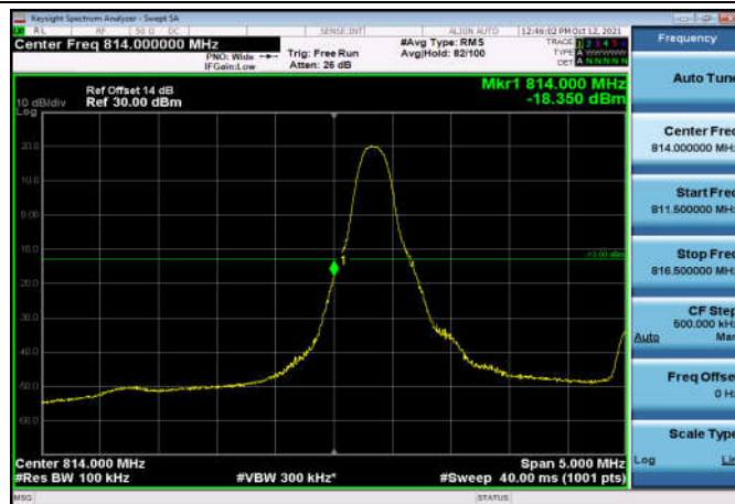
LowRange_FDD26_5MHz_816.5_fullRB _Low_QPSK
