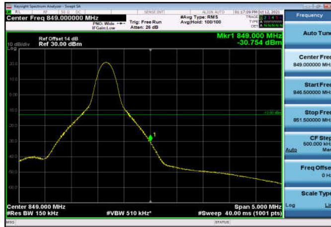
HighRange_FDD26_15MHz_841.5_fullRB _High_QPSK
