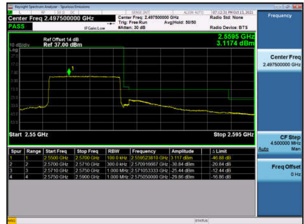
TDD7_20M Low oneRB 16Q
