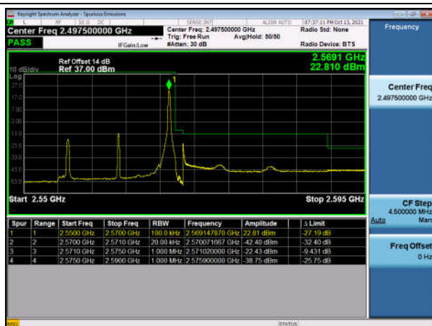
TDD7_15M High oneRB QPSK
