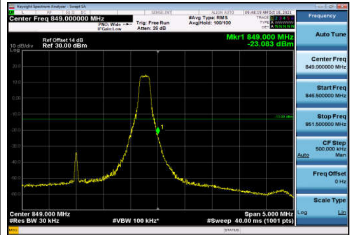
HighRange_FDD26_3MHz_847.5_fullRB _High_Q16
