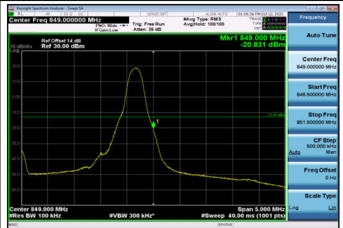
HighRange_FDD26_5MHz_846.5_OneRB _high_Q16
