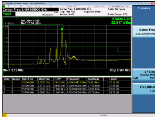
TDD7_5M High FullRB QPSK
