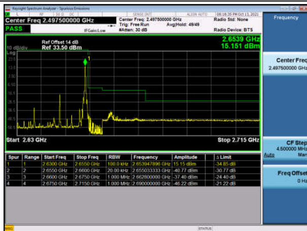
TDD41_20M High oneRB QPSK
