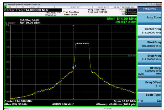
LowRange_FDD26_3MHz_815.5_OneRB _low_Q16
