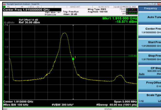
HighRange_FDD25_5MHz_1912.5_fullRB _High_QPSK
