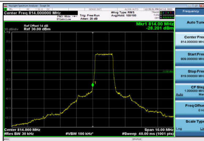
LowRange_FDD26_3MHz_815.5_OneRB _low_QPSK
