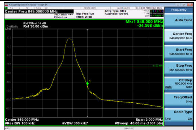
HighRange_FDD26_10MHz_844_fullRB _High_Q16
