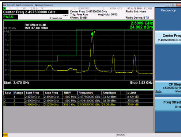
TDD7_15M Low FullRB QPSK
