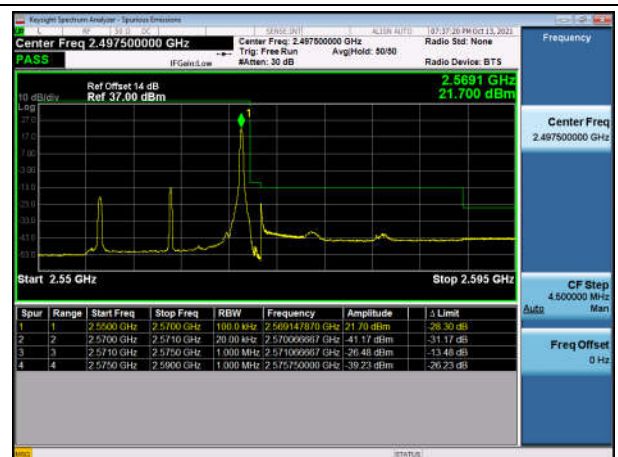
TDD7_15M High oneRB 16Q
