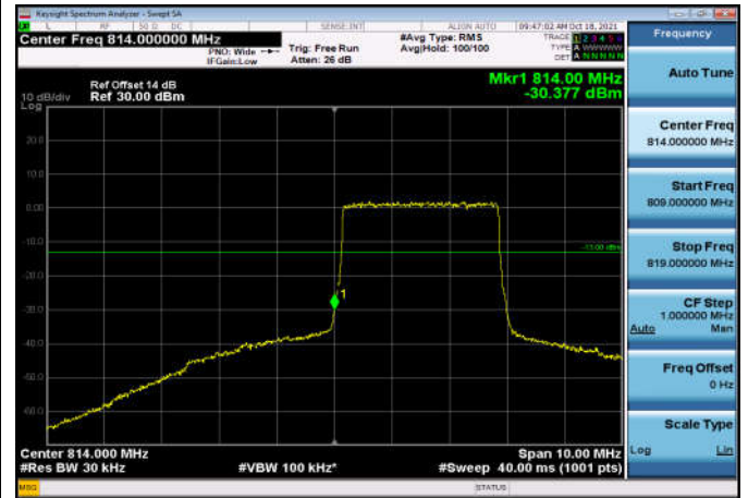
LowRange_FDD26_5MHz_816.5_OneRB _low_Q16
