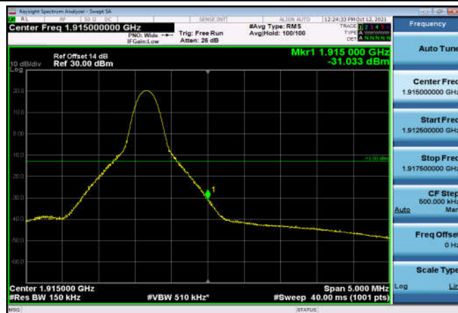
HighRange_FDD25_15MHz_1907.5_OneRB _high_QPSK
