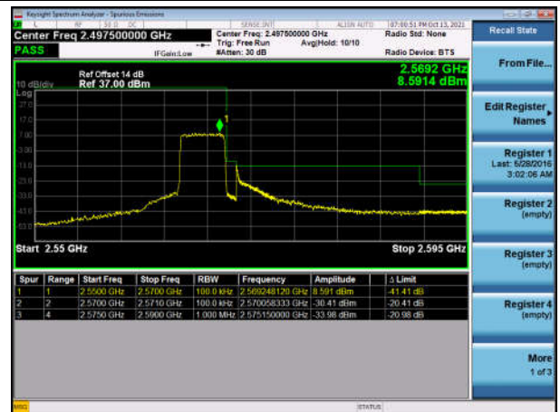
TDD7_10M Low oneRB 16Q
