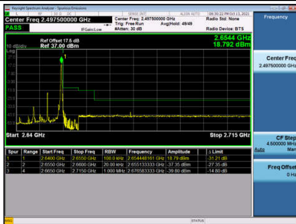
TDD41_10M High FullRB QPSK
