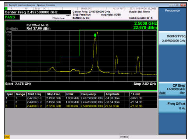
TDD7_15M Low FullRB 16Q
