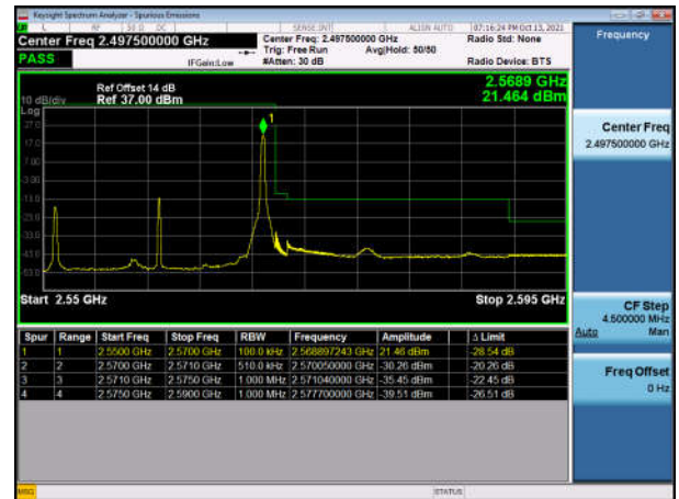
TDD7_20M High FullIRB 16Q
