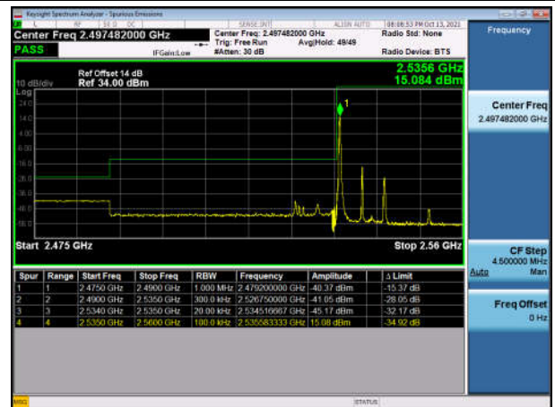
TDD41_10M Low FullIRB 16Q
