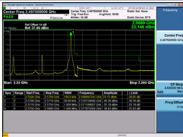
TDD7_10M High FullIRB QPSK
