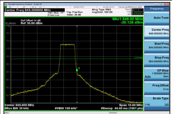
HighRange_FDD26_1.4MHz_848.3_fullRB _High_Q16
