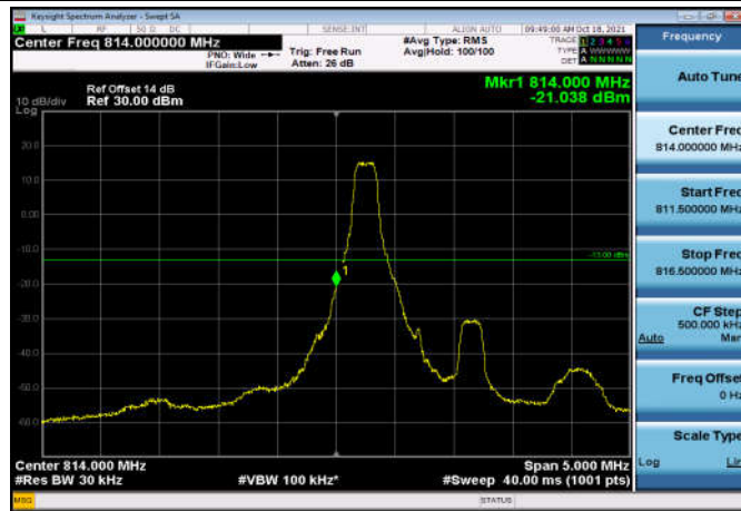
LowRange_FDD26_1.4MHz_814.7_fullRB _Low_QPSK
