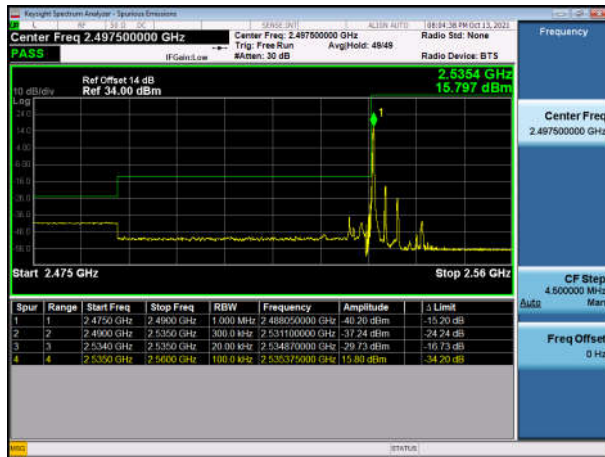
TDD41_5M Low FullRB QPSK
