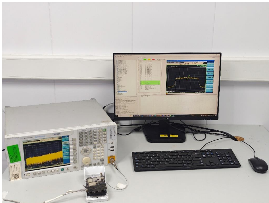
Conducted Test-BT/WIFI
