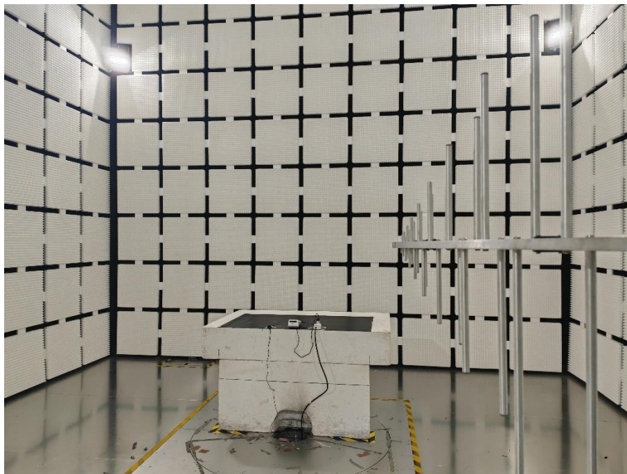
RSE-30MHz-1GHz-RF
