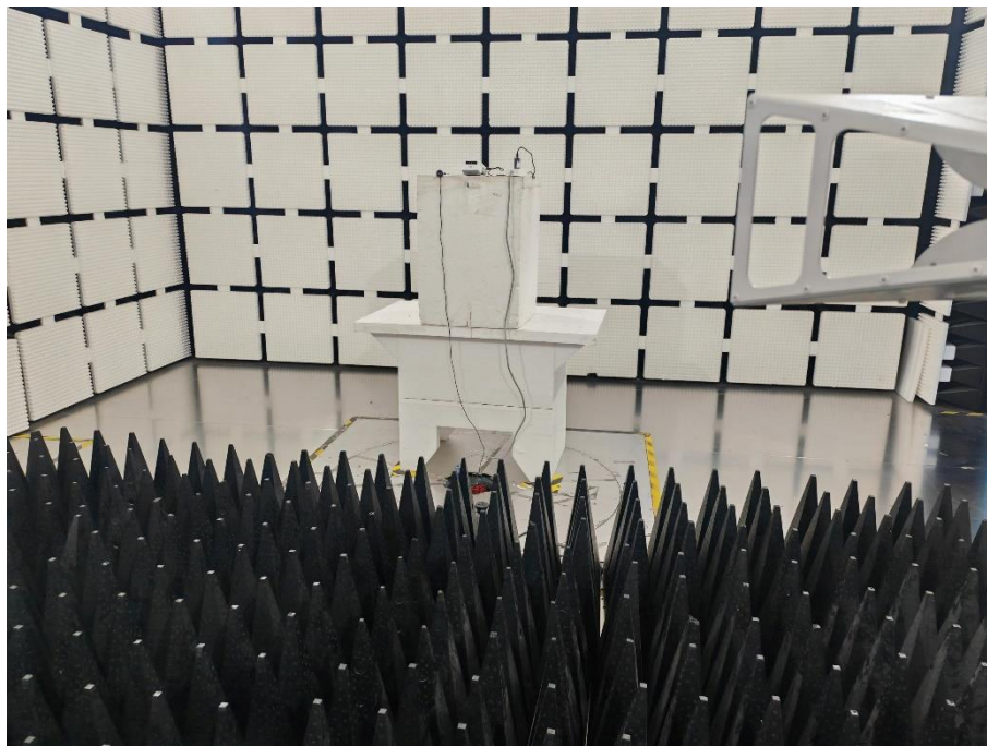
RSE-Above 1GHz-RF
