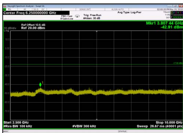
Transmitter Spurious Emission: 2402,Re ference Level
