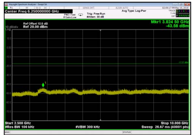
Transmitter Spurious Emission: 2440,Re ference Level
