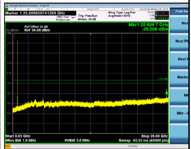
FDD07_MidRange_5MHz_30MHz~26GHz
