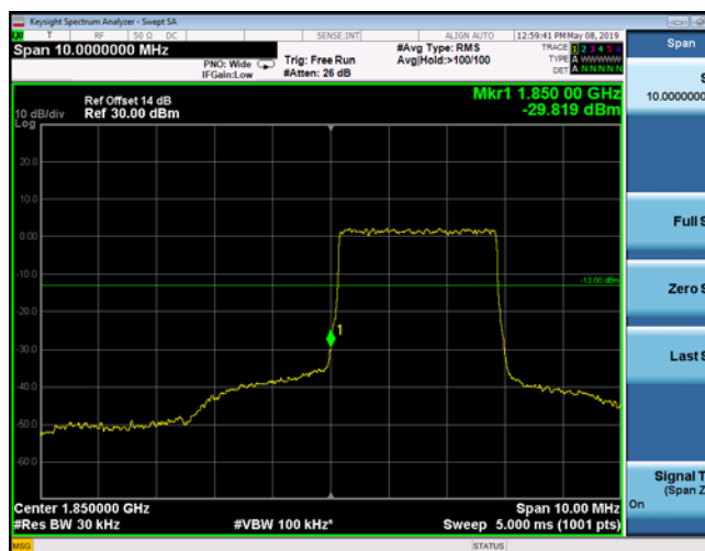
LowRange_FDD02_5MHz_1852.5_OneRB _low_QPSK
