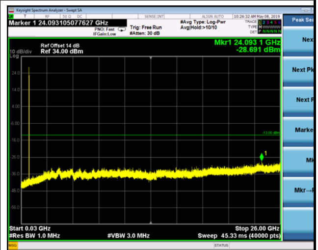
FDD05_LowRange_3MHz_30MHz~26GHz
