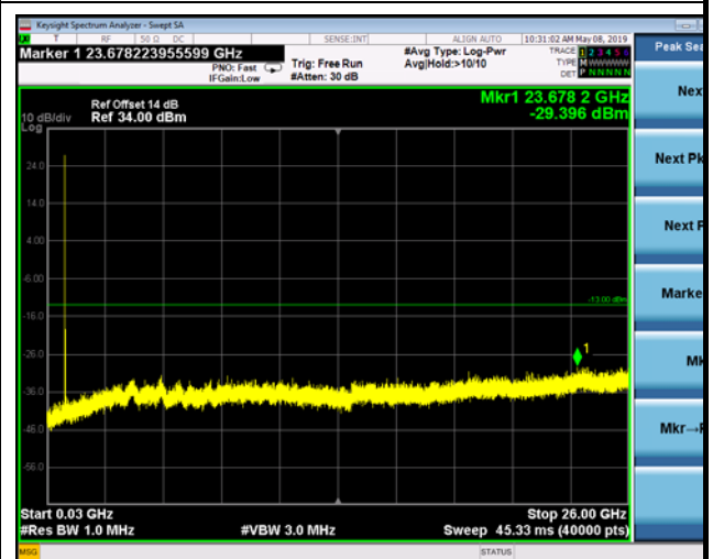
FDD05_LowRange_10MHz_30MHz~26GHz
