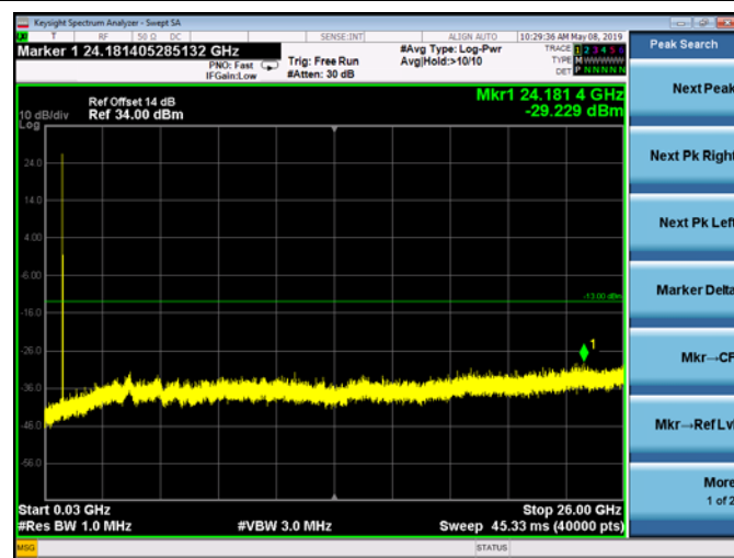
FDD05_LowRange_5MHz_30MHz~26GHz
