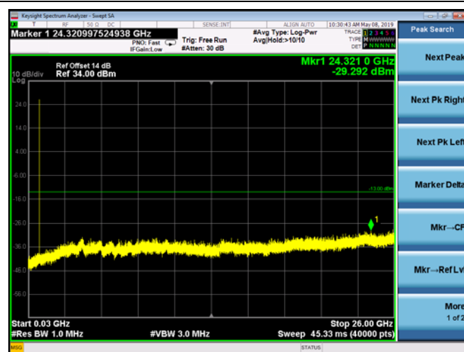
FDD05_HighRange_5MHz_30MHz~26GHz
