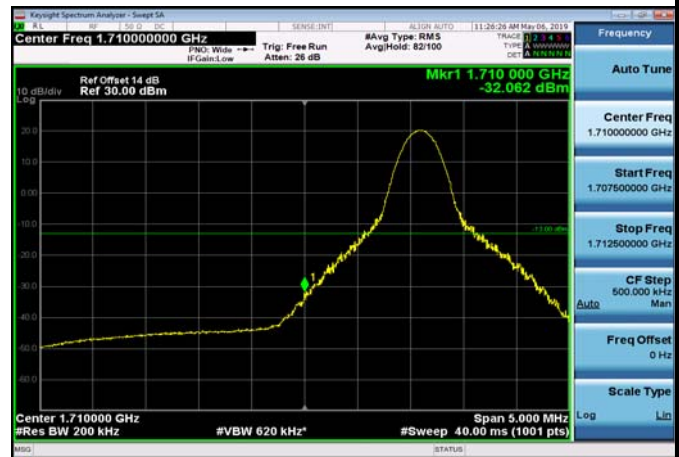
LowRange_FDD04_20MHz_1720_fullRB _Low_Q16
