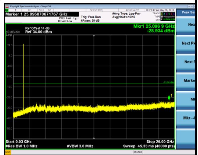
FDD05_MidRange_1.4MHz_30MHz~26GHz
