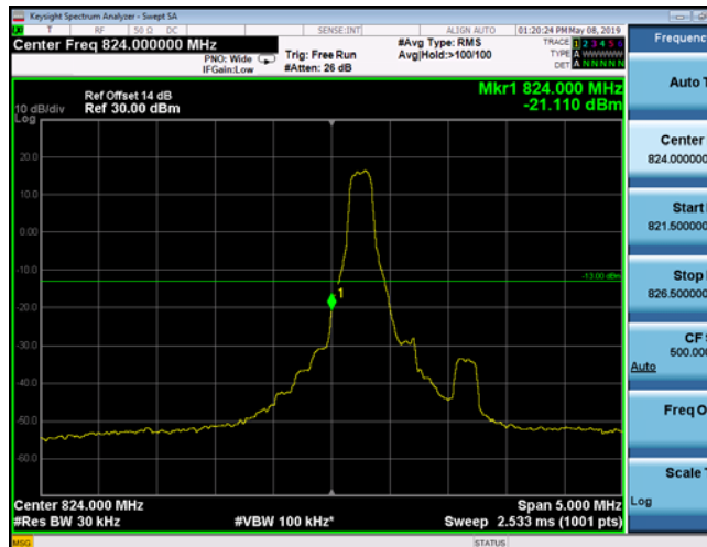
LowRange_FDD05_1.4MHz_824.7_fullRB _Low_QPSK
