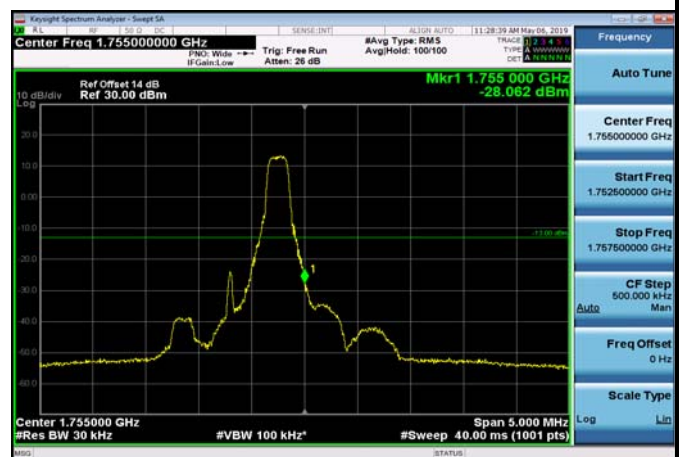
HighRange_FDD04_1.4MHz_1754.3_OneRB _high_Q16
