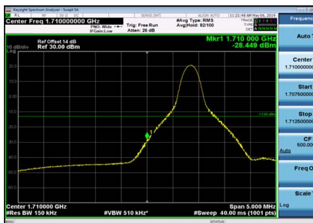
LowRange_FDD04_15MHz_1717.5_fullRB _Low_QPSK
