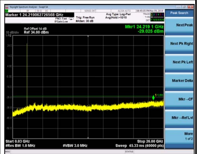
FDD07_LowRange_10MHz_30MHz~26GHz
