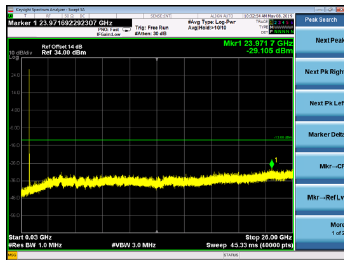
FDD07_LowRange_5MHz_30MHz~26GHz
