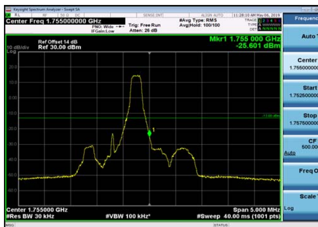
HighRange_FDD04_1.4MHz_1754.3_OneRB _high_QPSK
