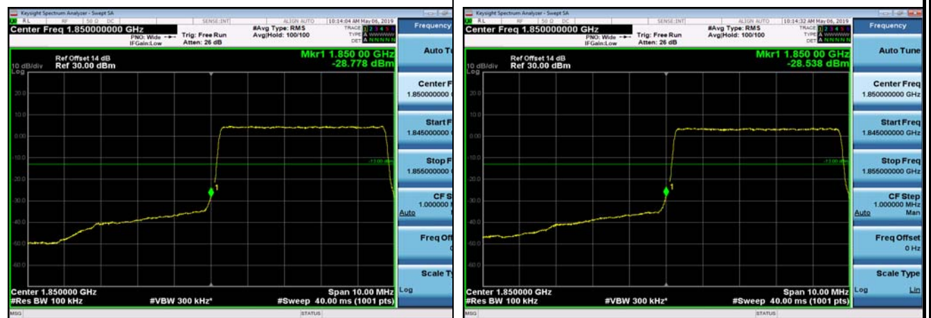
LowRange_FDD02_10MHz_1855_OneRB _low_QPSK
