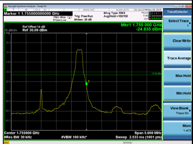
HighRange_FDD04_3MHz_1753.5_OneRB _high_Q16
