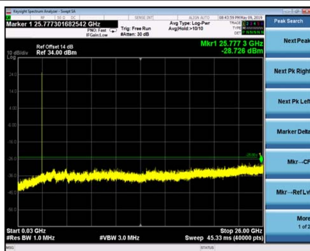
FDD07_HighRange_5MHz_30MHz~26GHz
