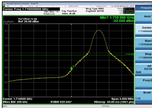
LowRange_FDD04_20MHz_1720_fullRB _Low_QPSK
