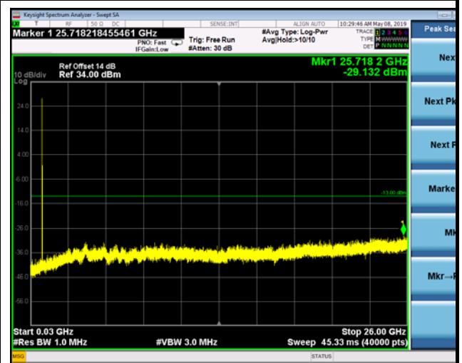
FDD05_MidRange_5MHz_30MHz~26GHz
