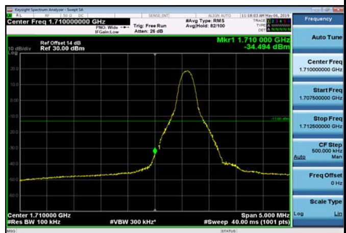
LowRange_FDD04_10MHz_1715_OneRB _low_Q16
