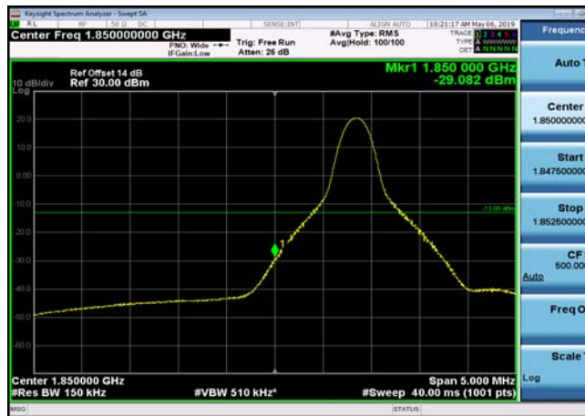
LowRange_FDD02_15MHz_1857.5_fullRB _Low_QPSK
