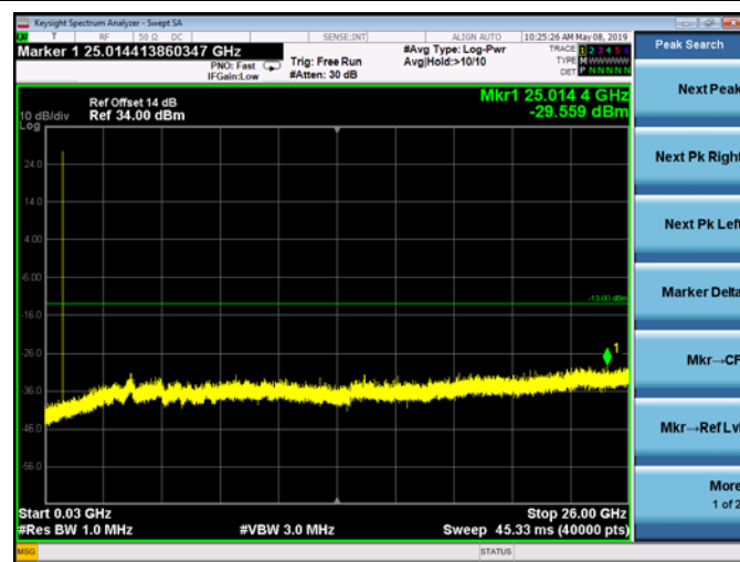
FDD05_HighRange_1.4MHz_30MHz~26GHz
