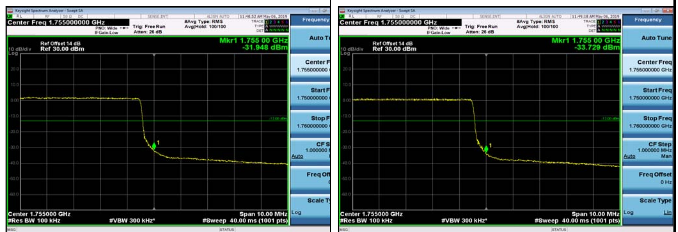
HighRange_FDD04_15MHz_1747.5_OneRB _high_QPSK
