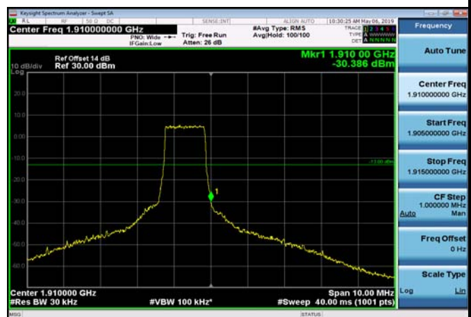
HighRange_FDD02_1.4MHz_1909.3 _fullRB_High_Q16
