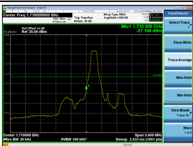
LowRange_FDD04_1.4MHz_1710.7_fullRB _Low_Q16
