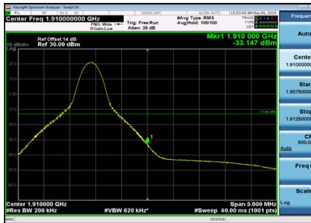
HighRange_FDD02_20MHz_1900_fullRB _High_QPSK
