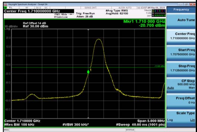
LowRange_FDD04_5MHz_1712.5_fullRB _Low_Q16
