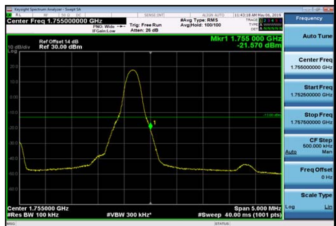
HighRange_FDD04_5MHz_1752.5_fullRB _High_Q16
