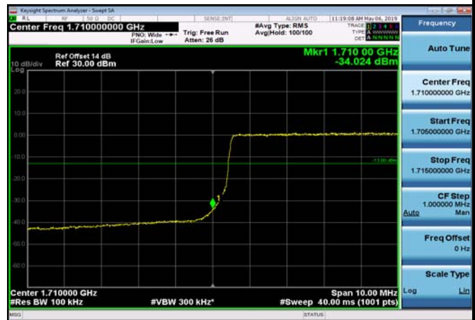
LowRange_FDD04_15MHz_1717.5_OneRB _low_Q16
