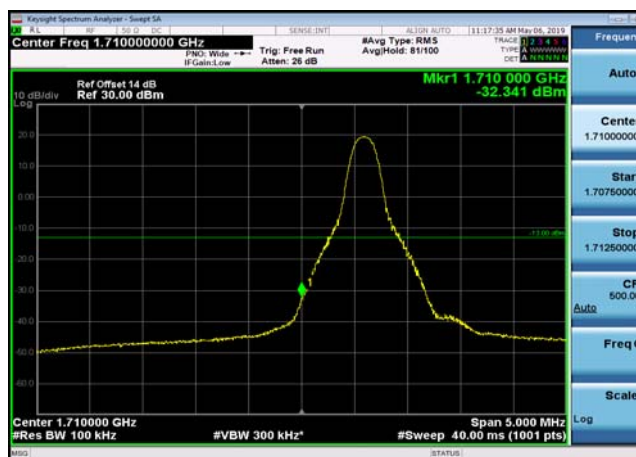
LowRange_FDD04_10MHz_1715_OneRB _low_QPSK
