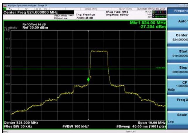
LowRange_FDD05_3MHz_825.5_OneRB _low_QPSK
