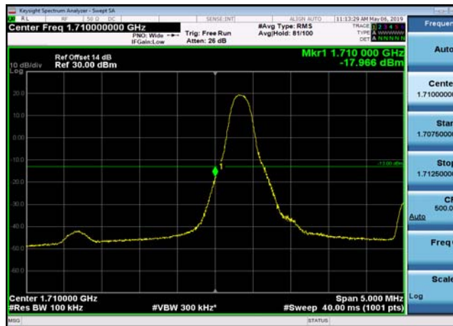
LowRange_FDD04_5MHz_1712.5_fullRB _Low_QPSK
