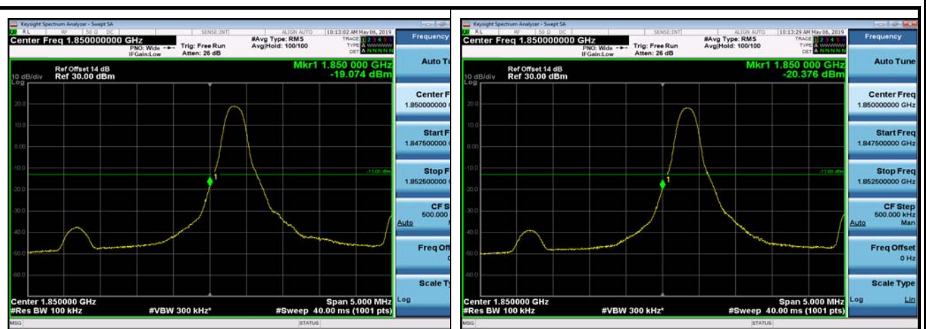
LowRange_FDD02_5MHz_1852.5_fullRB _Low_QPSK
