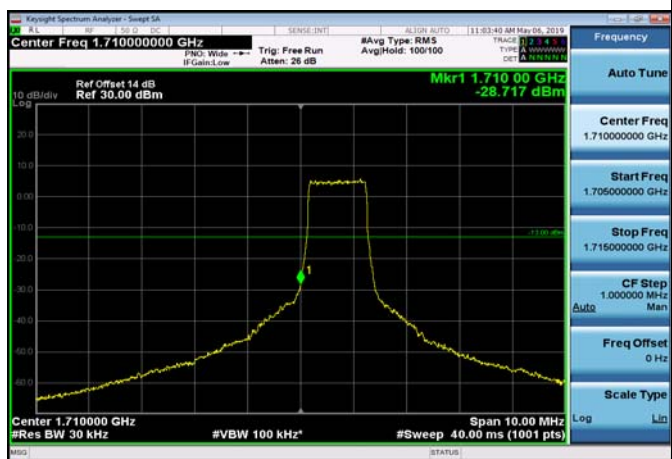
LowRange_FDD04_3MHz_1711.5_OneRB low Q16
