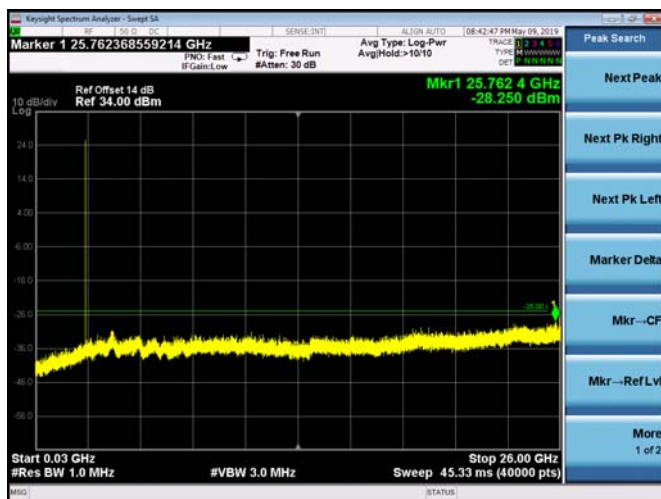
FDD07_HighRange_5MHz_30MHz~26GHz
