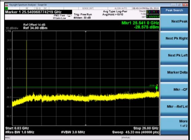
FDD07_HighRange_20MHz_30MHz~26GHz
