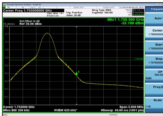
HighRange_FDD04_20MHz_1745_fullRB _High_QPSK
