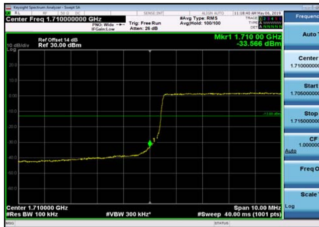
LowRange_FDD04_15MHz_1717.5_OneRB _low_QPSK
