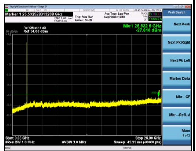
FDD07_LowRange_10MHz_30MHz~26GHz
