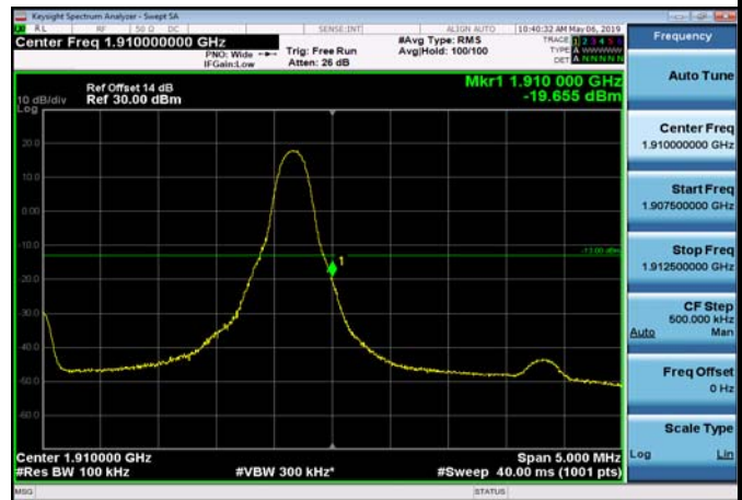
HighRange_FDD02_5MHz_1907.5_fullRB _High_Q16
