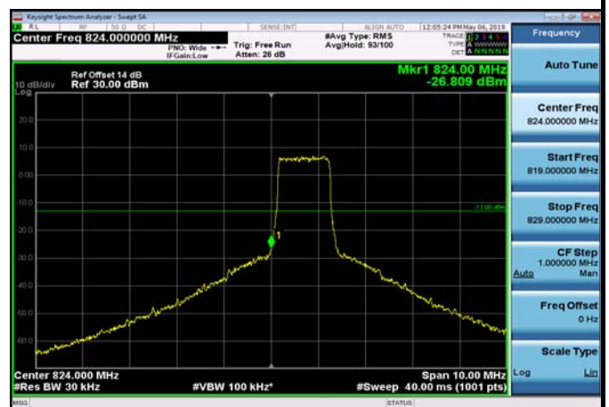
LowRange_FDD05_3MHz_825.5_OneRB _low_Q16
