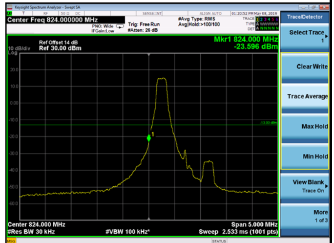
LowRange_FDD05_1.4MHz_824.7_fullRB _Low_Q16
