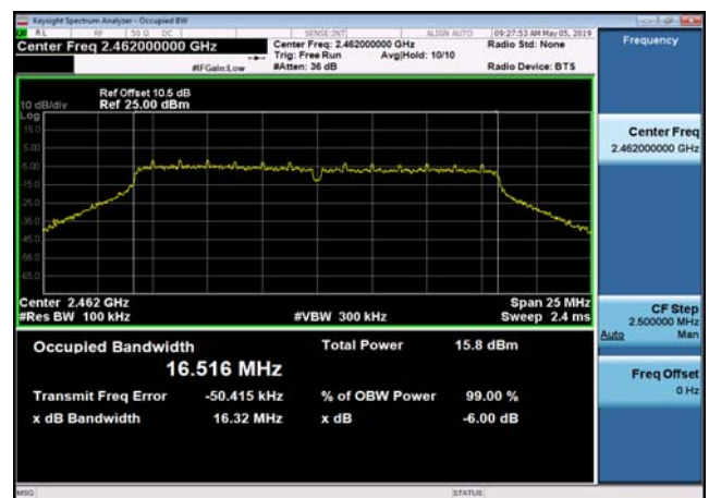
6dB Bandwidth-802.11g,2462MHz
