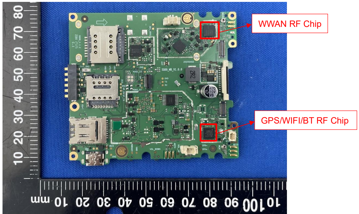
MAIN BOARD TOP VIEW (WITHOUT SHIELDING)
