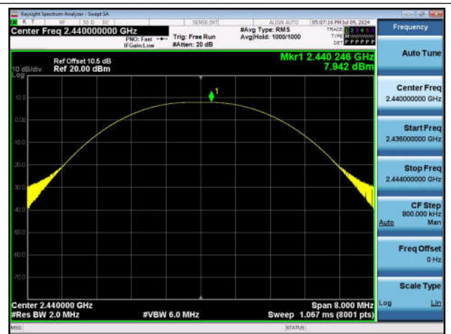
BLE_1M-Ant1-2440-PASS
