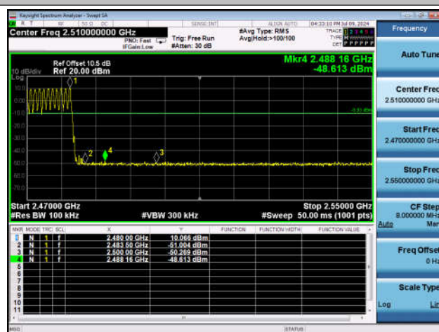
DH5-Ant1-Hop_2480-PASS
