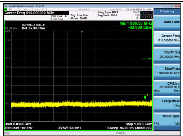
3DH5-Ant1-2480-30~1000-PASS
