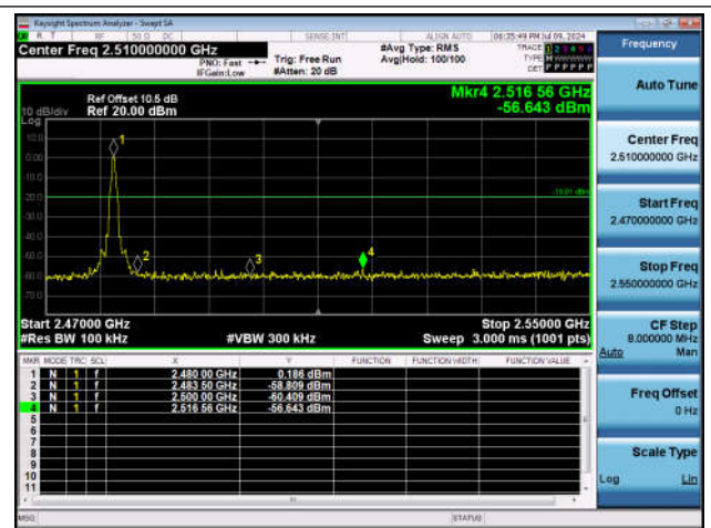
DH5-Ant1-2480-PASS
