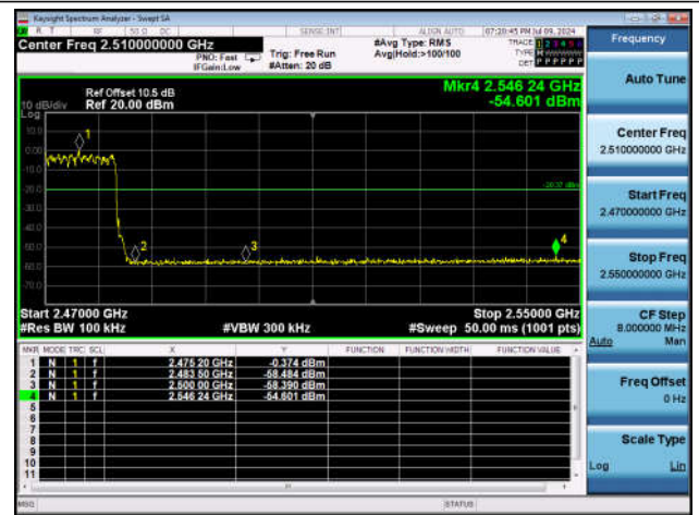
3DH5-Ant1-Hop_2480-PASS
