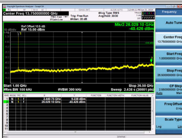
2DHS-Ant1-2441-1000~26500-PASS
