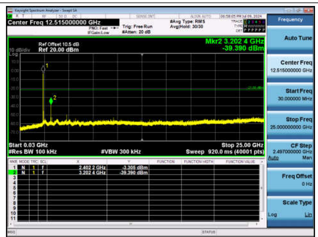
2DH5-Ant1-2402-30~25000-PASS
