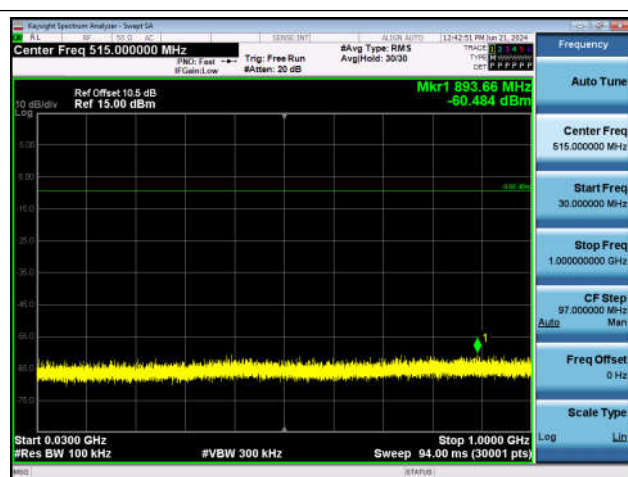
2DHS-Ant1-2441-30~1000-PASS
