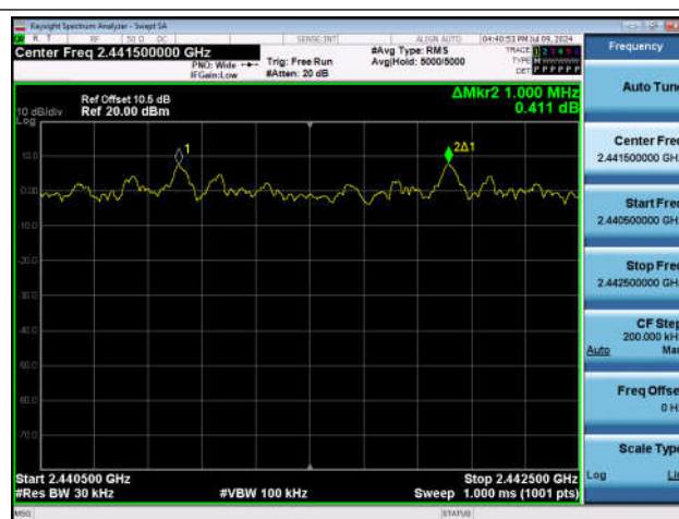
2DH5-Ant1-Hop-PASS
