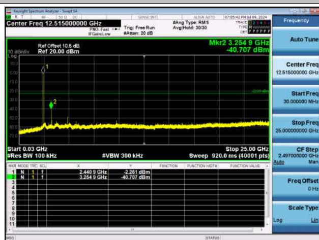
3DH5-Ant1-2441-30~25000-PASS
