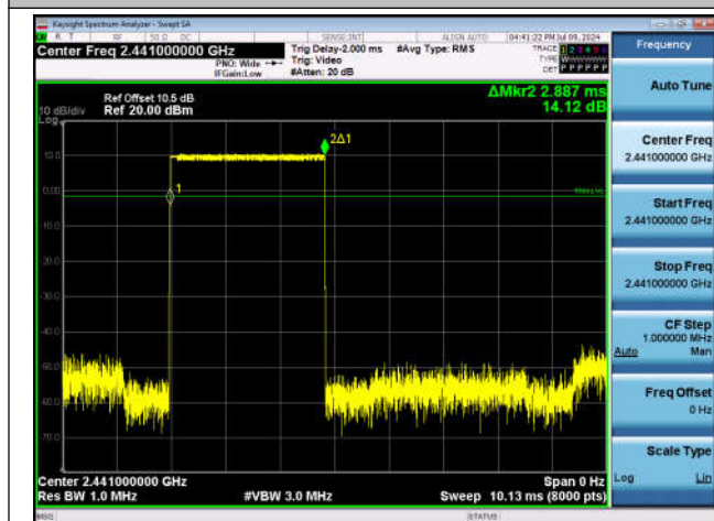
2DH5-Ant1-Hop-PASS
