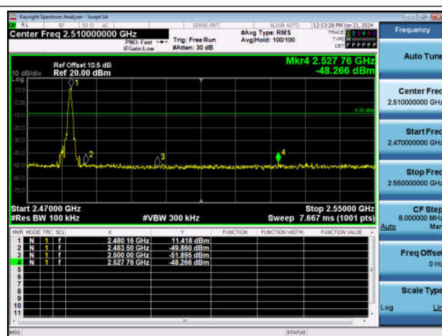
DH5-Ant1-2480-PASS
