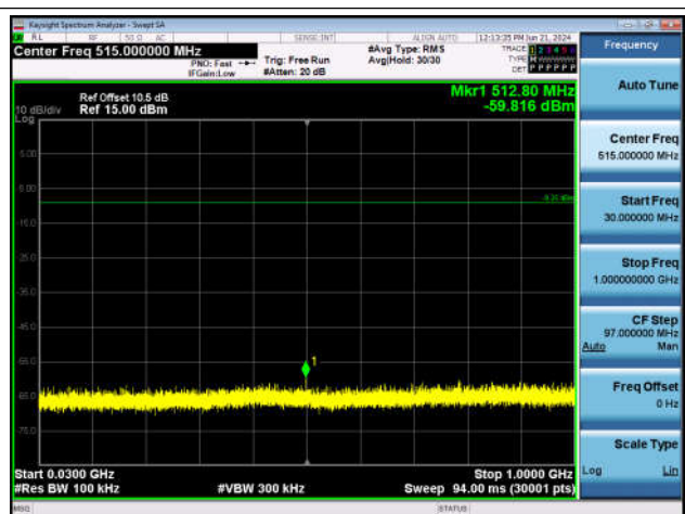
DH5-Ant1-2480-30~1000-PASS
