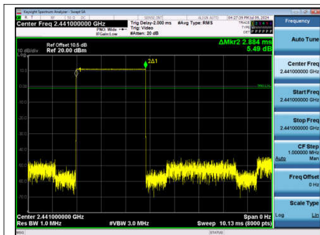
DH5-Ant1-Hop-PASS
