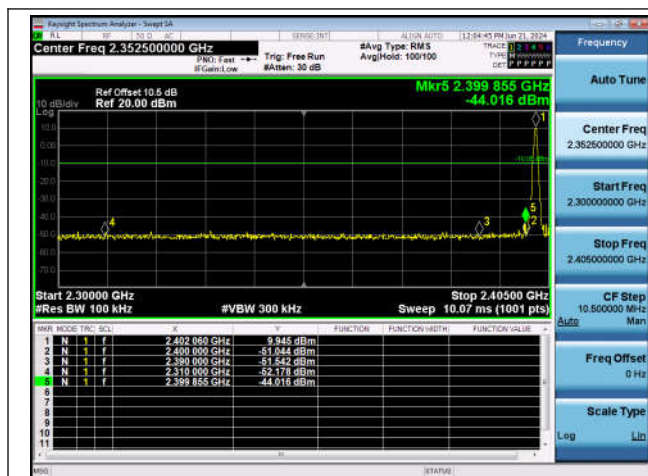
DH5-Ant1-2402-PASS
