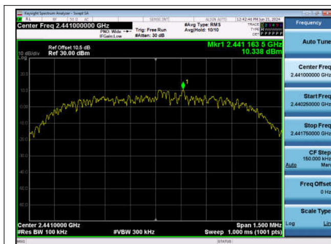
2DHS-Ant1-2441-0~Reference-PASS
