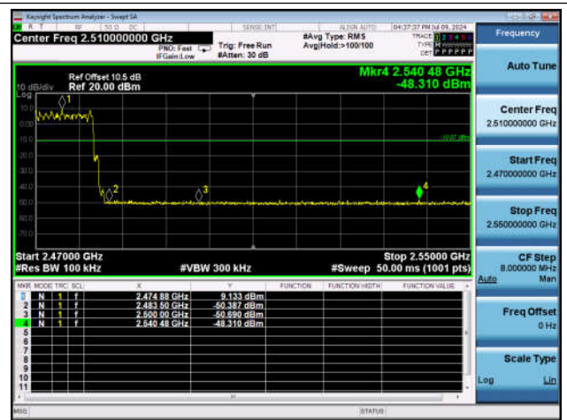
2DH5-Ant1-Hop_2480-PASS
