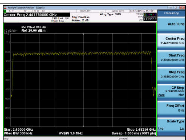
2DH5-Ant1-Hop-PASS
