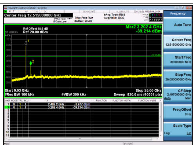
DH5-Ant1-2402-30~25000-PASS
