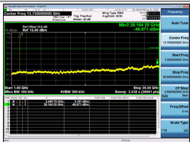
3DH5-Ant1-2441-1000~26500-PASS
