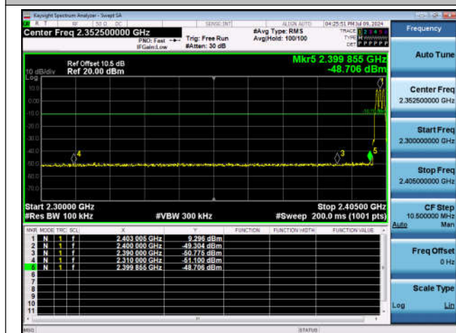
DH5-Ant1-Hop_2402-PASS
