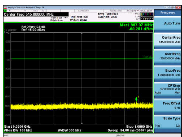
3DH5-Ant1-2402-30~1000-PASS
