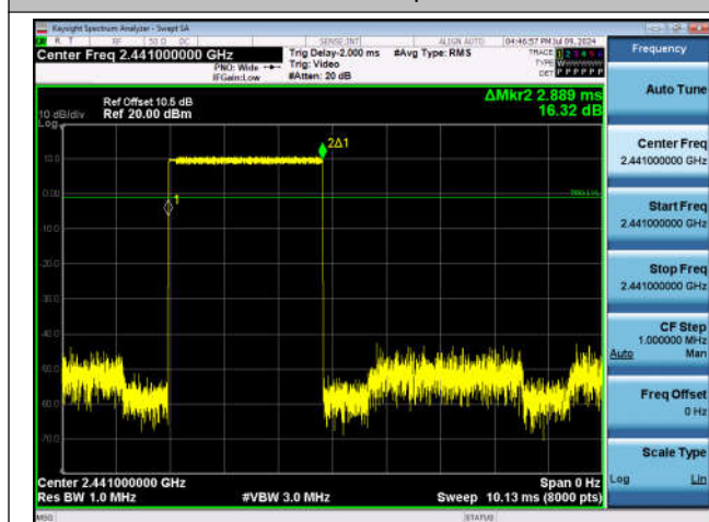
3DH5-Ant1-Hop-PASS
