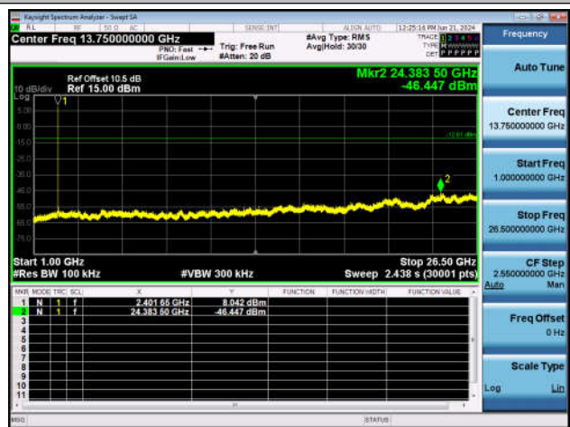
2DH5-Ant1-2402-1000~26500-PASS
