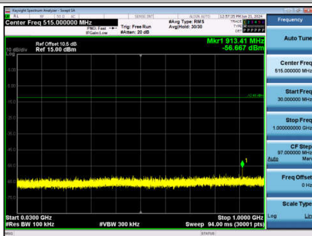
2DHS-Ant1-2480-30~1000-PASS
