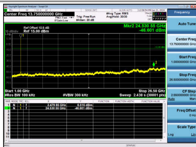
2DHS-Ant1-2480-1000~26500-PASS
