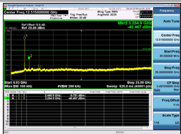
DH5-Ant1-2441-30~25000-PASS
