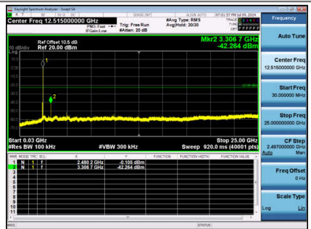
2DH5-Ant1-2480-30~25000-PASS
