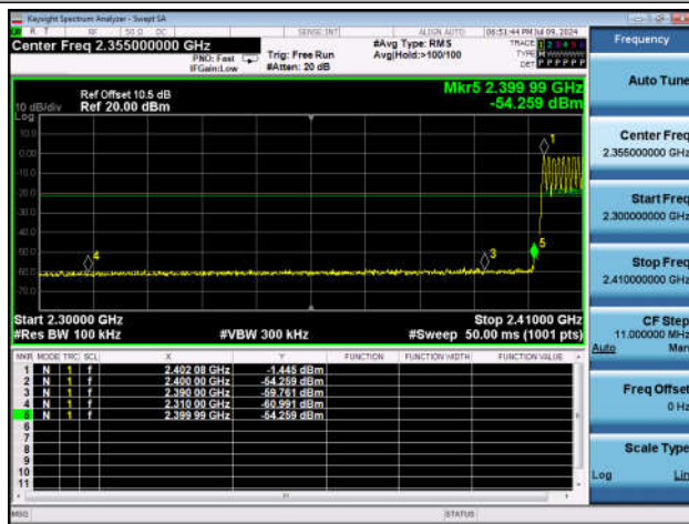
DH5-Ant1-Hop_2402-PASS
