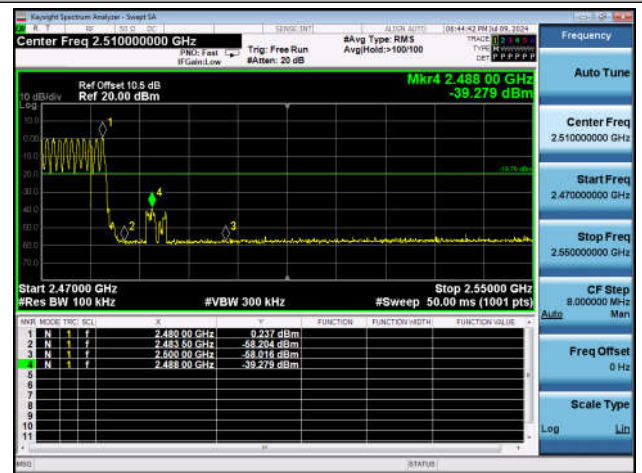
DH5-Ant1-Hop_2480-PASS
