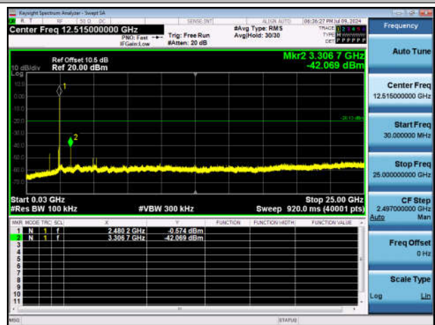
DH5-Ant1-2480-30~25000-PASS
