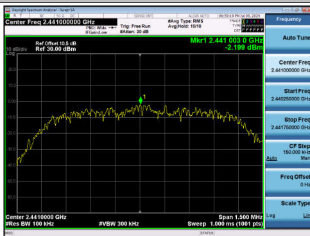
2DH5-Ant1-2441-0~Reference-PASS
