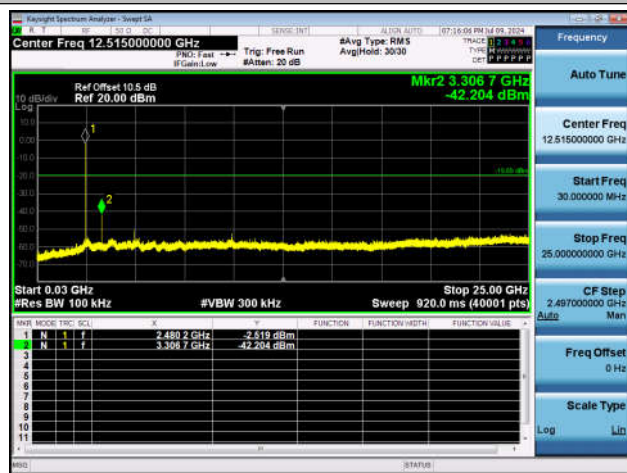
3DH5-Ant1-2480-30~25000-PASS
