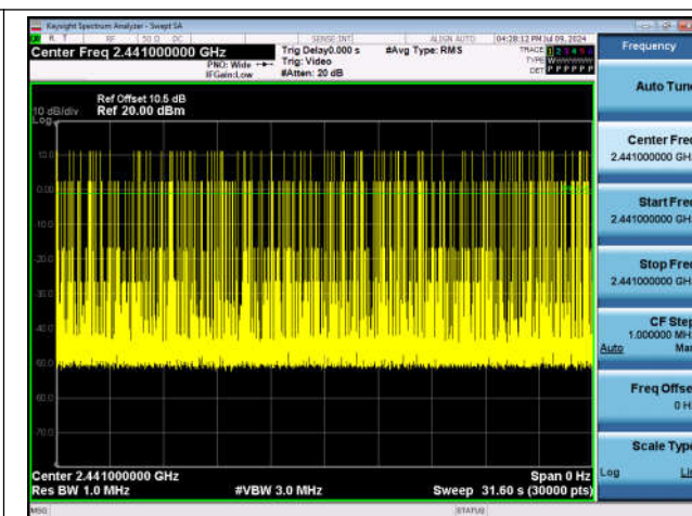
DH5-Ant1-Hop-PASS
