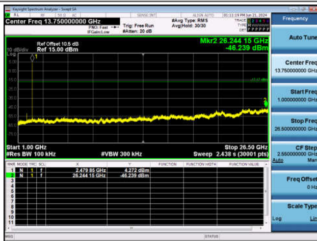
3DH5-Ant1-2480-1000~26500-PASS
