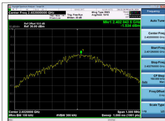
DH5-Ant1-2402-0~Reference-PASS
