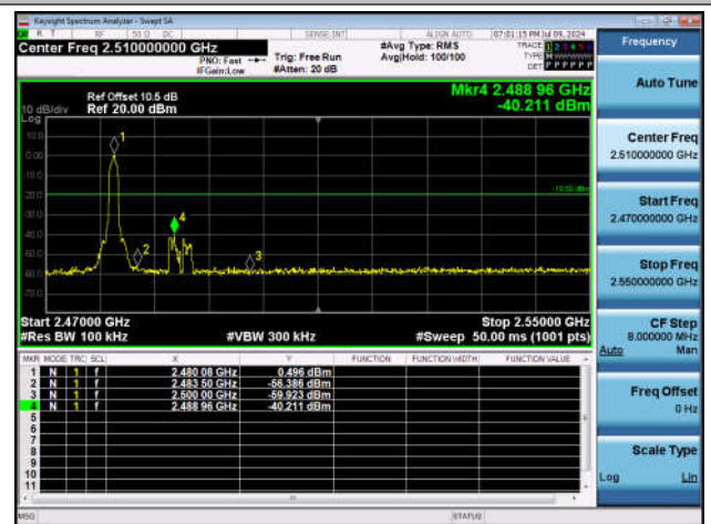
2DH5-Ant1-2480-PASS
