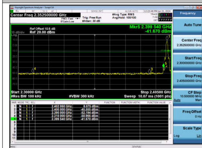
2DH5-Ant1-2402-PASS
