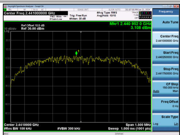
3DH5-Ant1-2441-0~Reference-PASS
