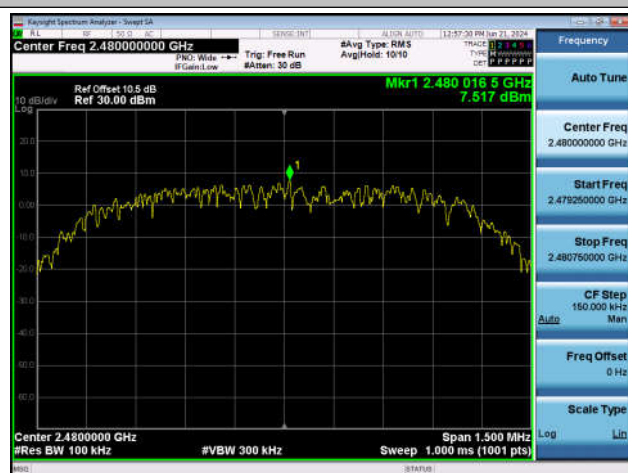
2DHS-Ant1-2480-0~Reference-PASS
