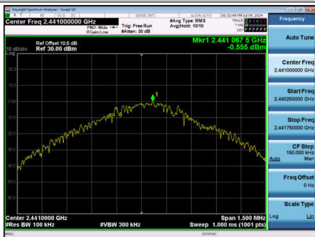
DH5-Ant1-2441-0~Reference-PASS
