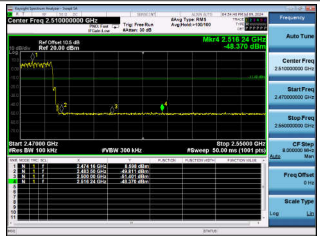
3DH5-Ant1-Hop_2480-PASS
