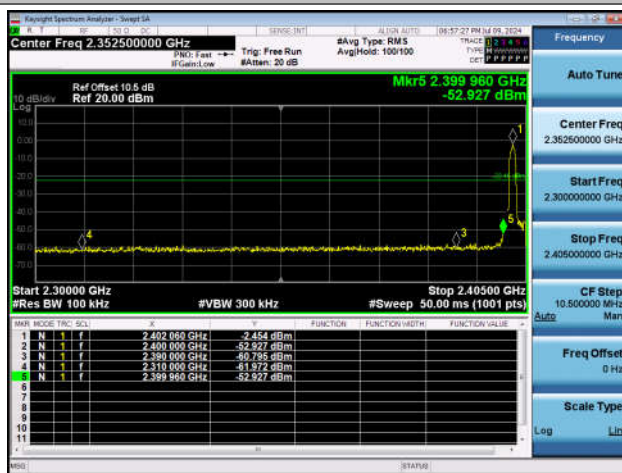
2DH5-Ant1-2402-PASS
