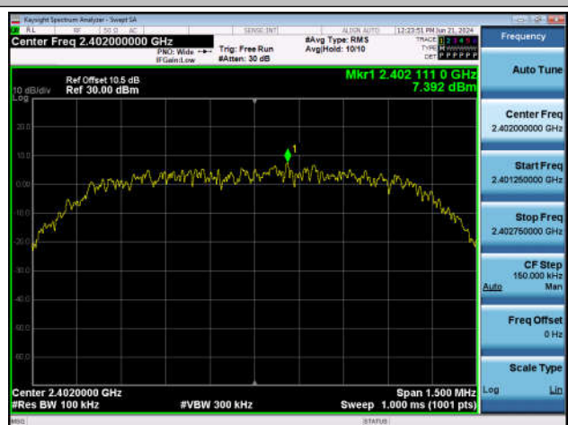
2DH5-Ant1-2402-0~Reference-PASS
