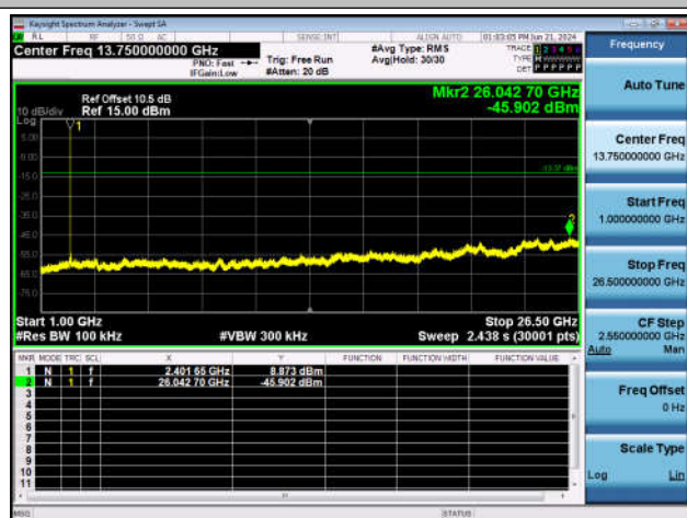
3DH5-Ant1-2402-1000~26500-PASS
