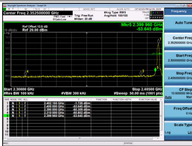
3DH5-Ant1-2402-PASS
