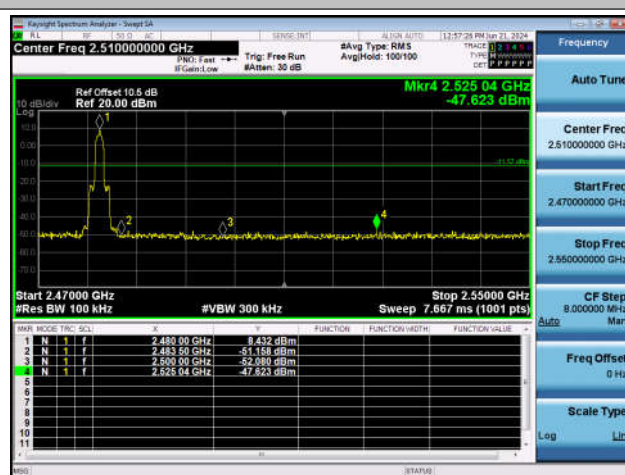
2DH5-Ant1-2480-PASS
