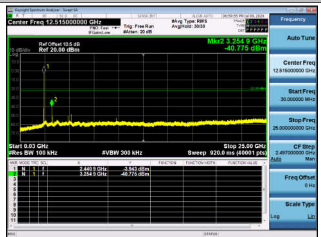
2DH5-Ant1-2441-30~25000-PASS
