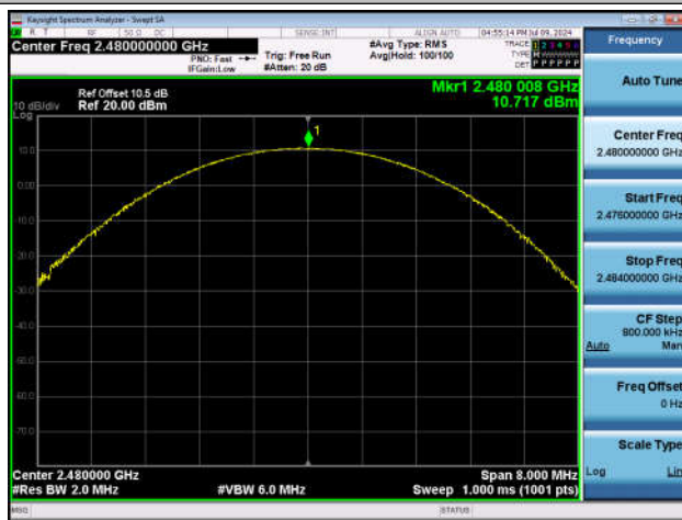
3DH5-Ant1-2480-PASS
