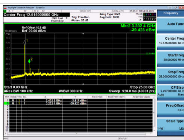
3DH5-Ant1-2402-30~25000-PASS
