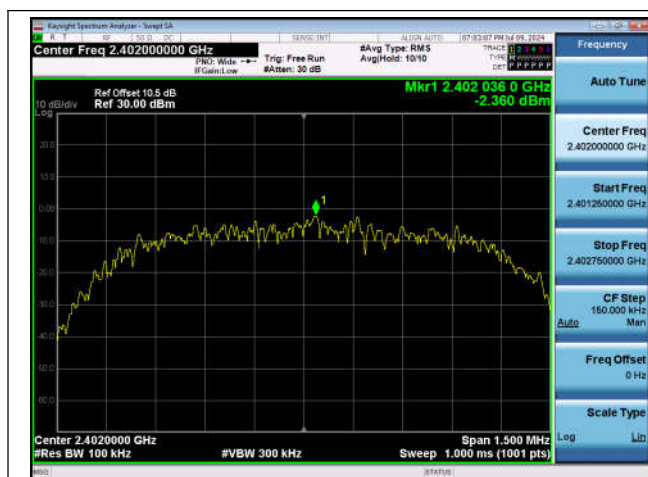
3DH5-Ant1-2402-0~Reference-PASS
