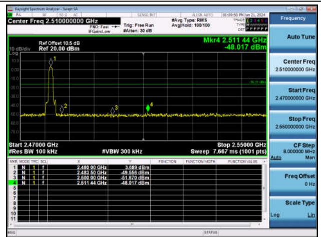
3DH5-Ant1-2480-PASS
