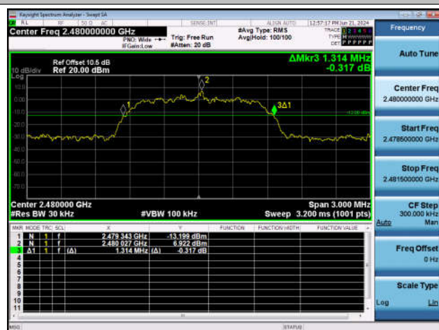
2DH5-Ant1-2480
